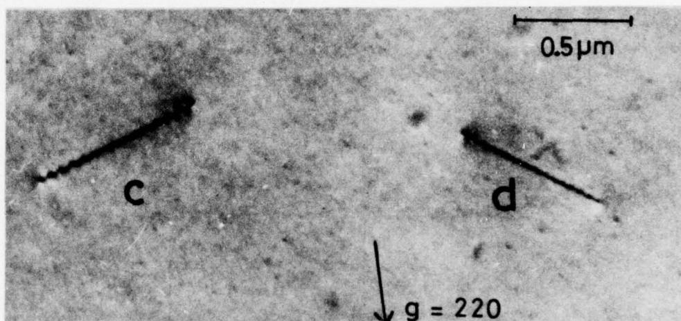
FIGURE 4. A higher magnification TEM micrograph of two dislocations which show typical oscillating contrast but no obvious precipitation.
