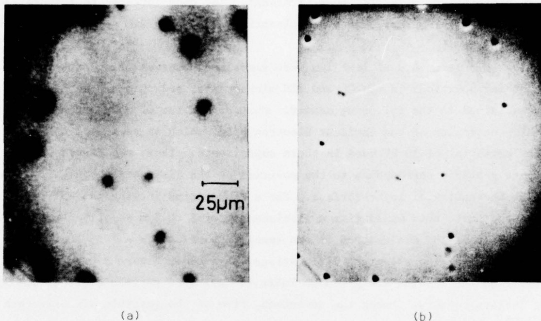
FIGURE 5. (a) A CL micrograph of the (111)A oriented Te-doped layer and (b) the same area after etching to reveal dislocation sites imaged in the secondary electron mode of an SEM
