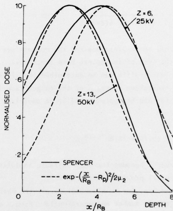
FIGURE 2. Dose-depth curves for Z < 14 \epsilon \approx 250 , \frac{R_B}{K} = 0.34 \epsilon^{1.78}
