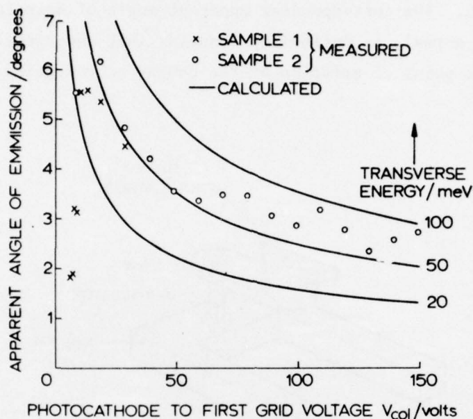
FIGURE 7. The apparent angle of emission at half the maximum electron density as a function of the collection voltage.
