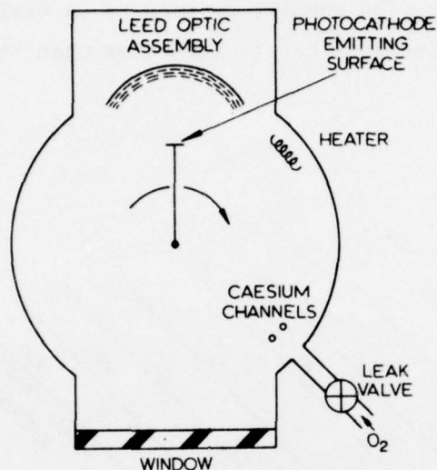
FIGURE 5. Cross section of the activation chamber.
