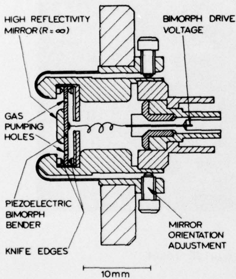
FIGURE 2. Bimorph bender mirror mount.
