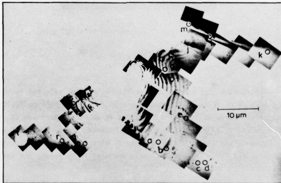
FIGURE 3. A low-magnification TEM micrograph montage of part of the same area shown in Figure 2. The lettered circles mark the positions of dislocations in the thin foil and these can be compared with the positions of the lettered dark spots in Figure 2.
