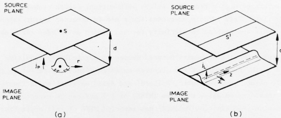
FIGURE 1. (a) Electron point spread function (b) Electron line spread function.
