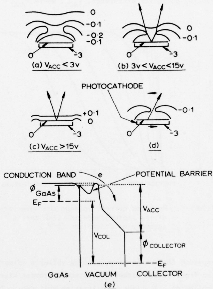
FIGURE 9. (a)(b)(c) The equipotentials in front of the cathode. The voltages are referred to the cathode. (d) The reverse motions of the illuminating spot and image on the phosphor. (e) The potential energy versus distance for an electron.
