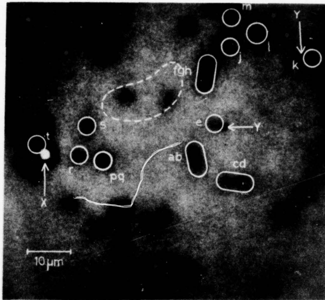
FIGURE 2. A CL micrograph of a (100) oriented Si-doped GaP layer. The dashed line marks the position of a hole produced during the TEM specimen preparation of this same area. The feature marked X is a pinhole in the epitaxial layer and those marked Y are small particles of dirt. The remaining letters refer to dark spots.
