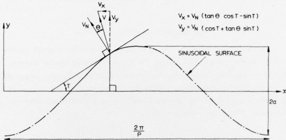
FIGURE 2. Velocity components of electrons emitted from a sinusoidal photocathode surface
