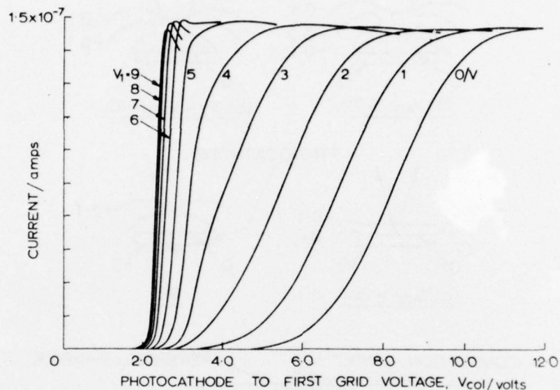
FIGURE 8. Measured current-voltage characteristics of the photocathode and LEED optics assembly as a function of V_1 .
