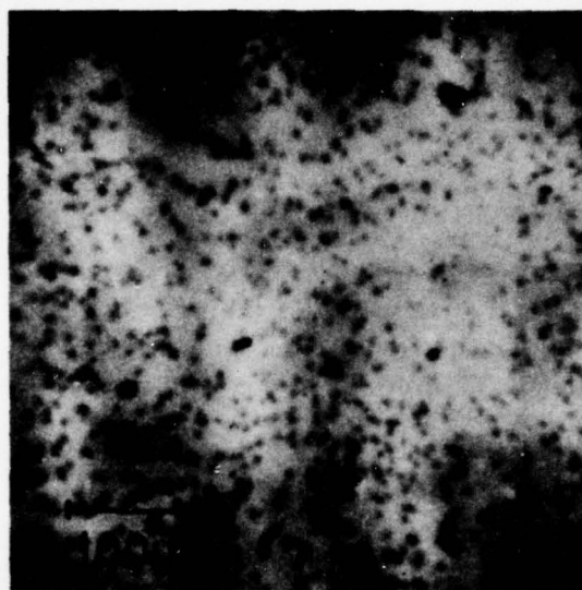
FIGURE 1. A typical CL micrograph of a GaP epitaxial layer with a dark spot density of approximately 5 \times 10^5 cm -2 .
