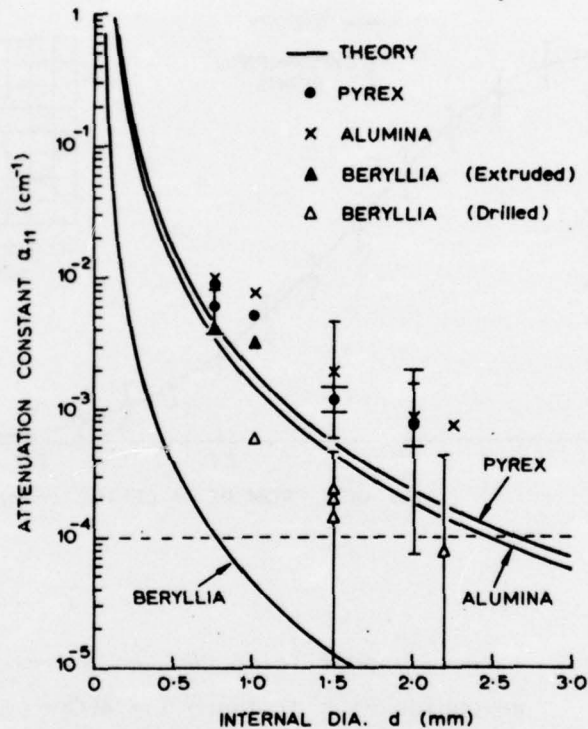
FIGURE 4. Variation of attenuation constant \alpha_{11} with internal diameter of waveguide for Pyrex, alumina and beryllia tubes
