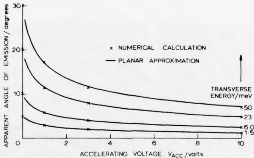
FIGURE 10. The apparent angle of emission of electrons with 0.2 eV emission energy.
