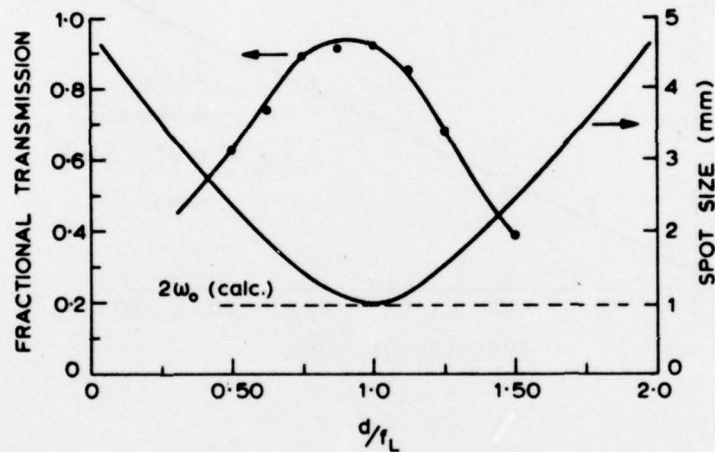
FIGURE 2. Dependence of transmitted spot size on lens-to-waveguide separation for a 1.5 mm bore alumina tube
