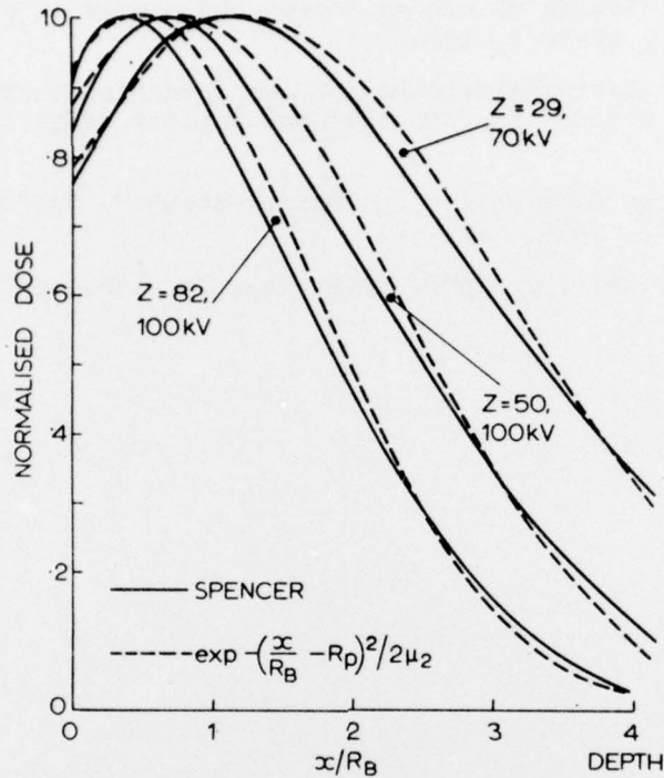
FIGURE 3. Dose-depth curve for Z > 14 \epsilon \sim 250, \frac{R_B}{K} = 0.34e^{1.78}
