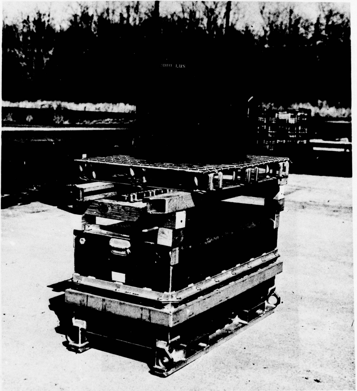
FIG. 16 CONCENTRATED OVERLOAD TEST (STACKING)
