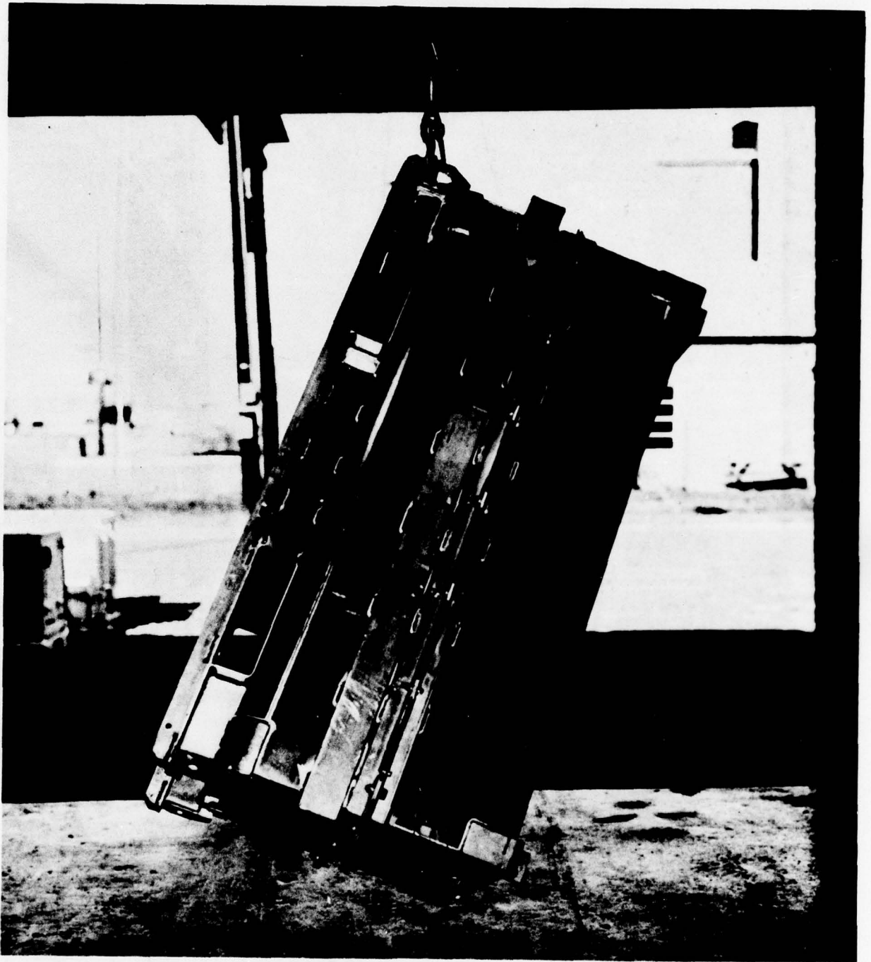
FIG. 18 CONTAINER SUSPENDED BY ONE HOISTING FITTING.
