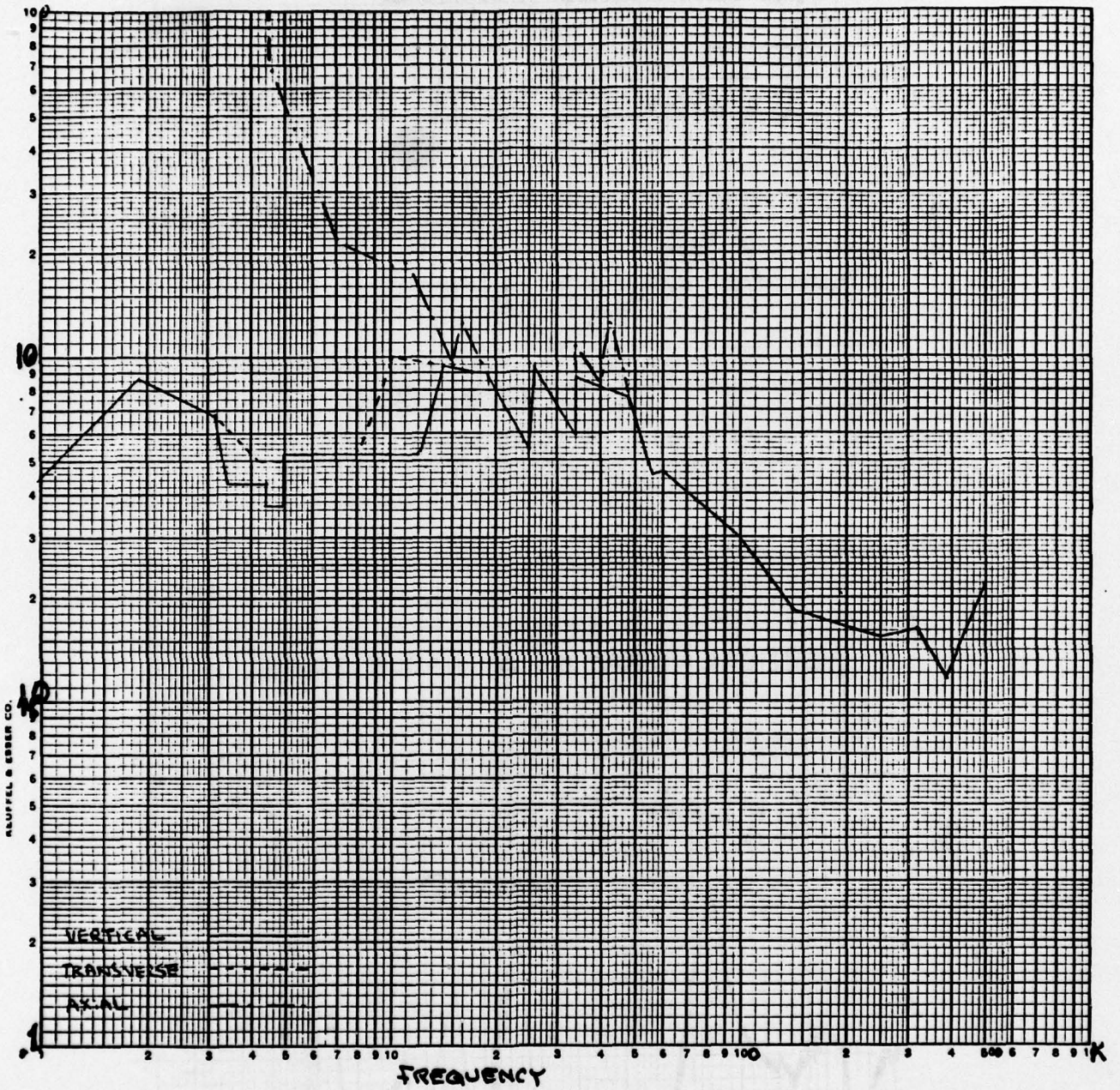
FIG. 9 PERMISSIBLE TRANSMISSIBILITY
