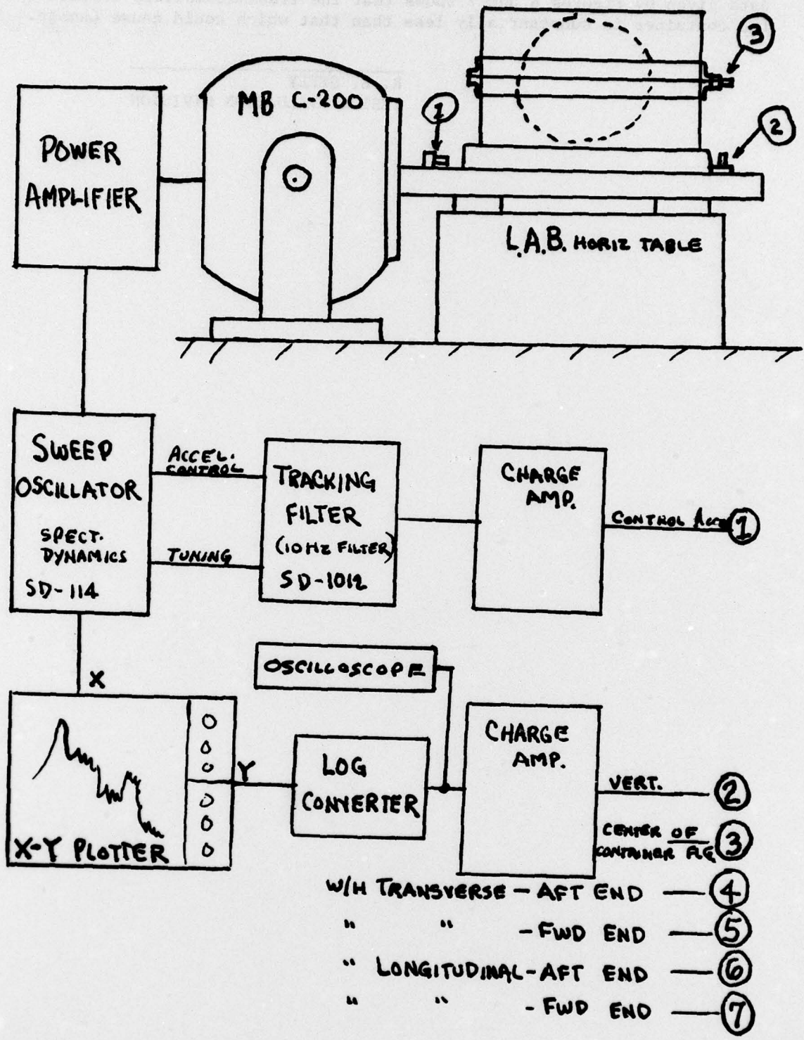
FIG. 1 TEST ARRANGEMENT
