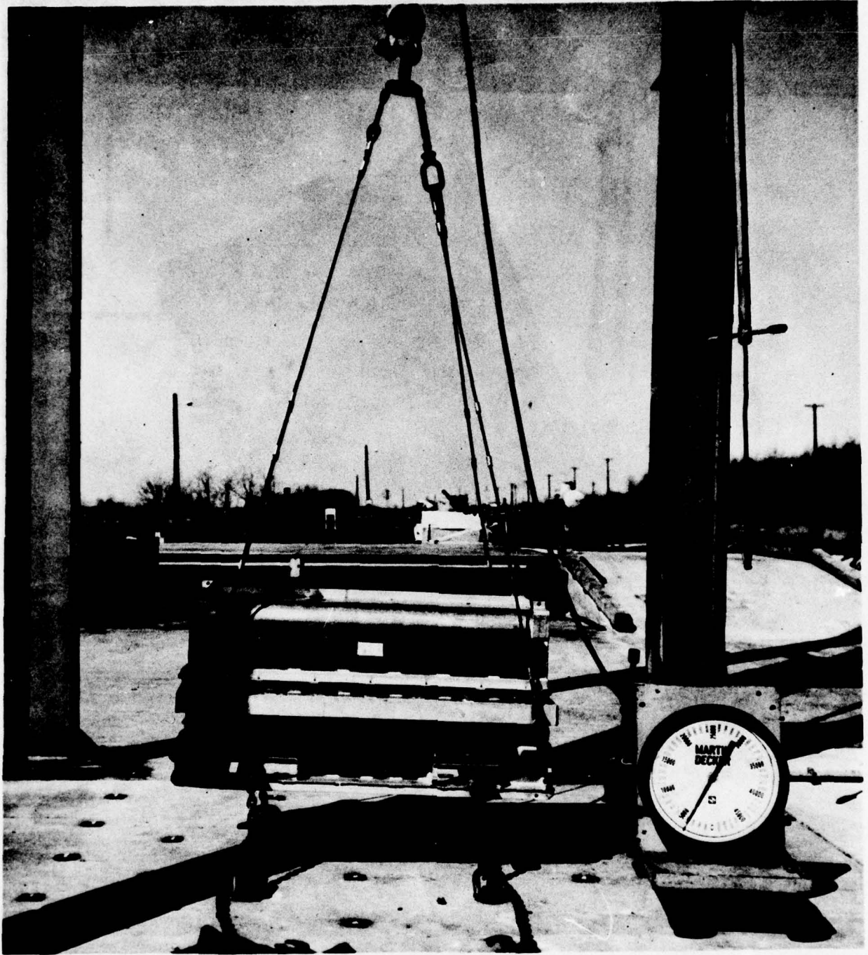
FIG. 19 HOISTING FITTING - 5:1 OVERLOAD TEST.
