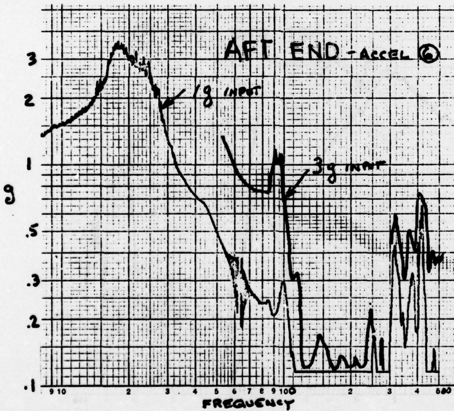
WARHEAD RESPONSE TO LONGITUDINAL CONTAINER VIBRATION
