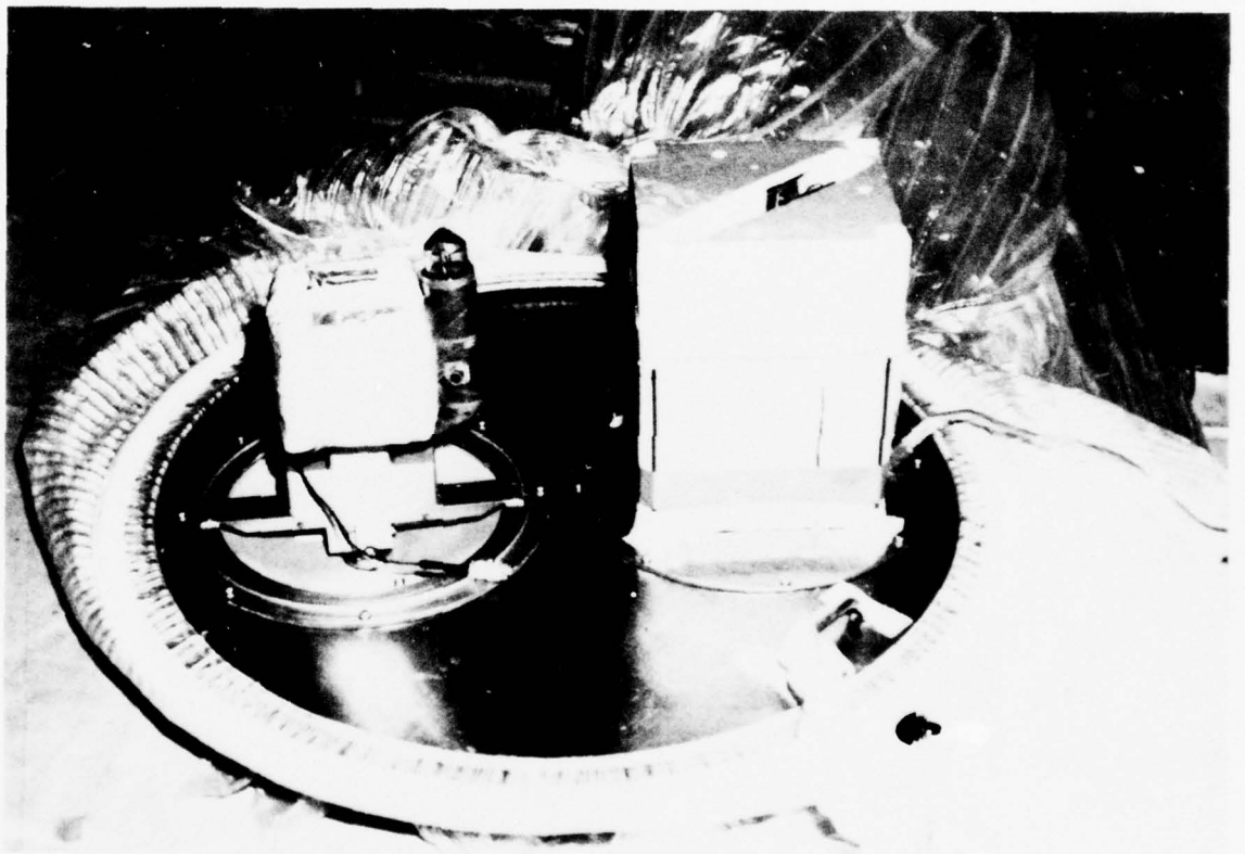
Figure 10. STRATCOM III payload on apex plate of balloon - September 1972.
