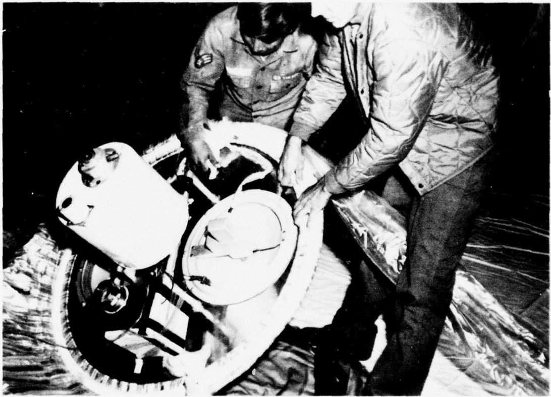
Figure 24. STRATCOM VI apex plate, mounted instrument package - September 1975.
