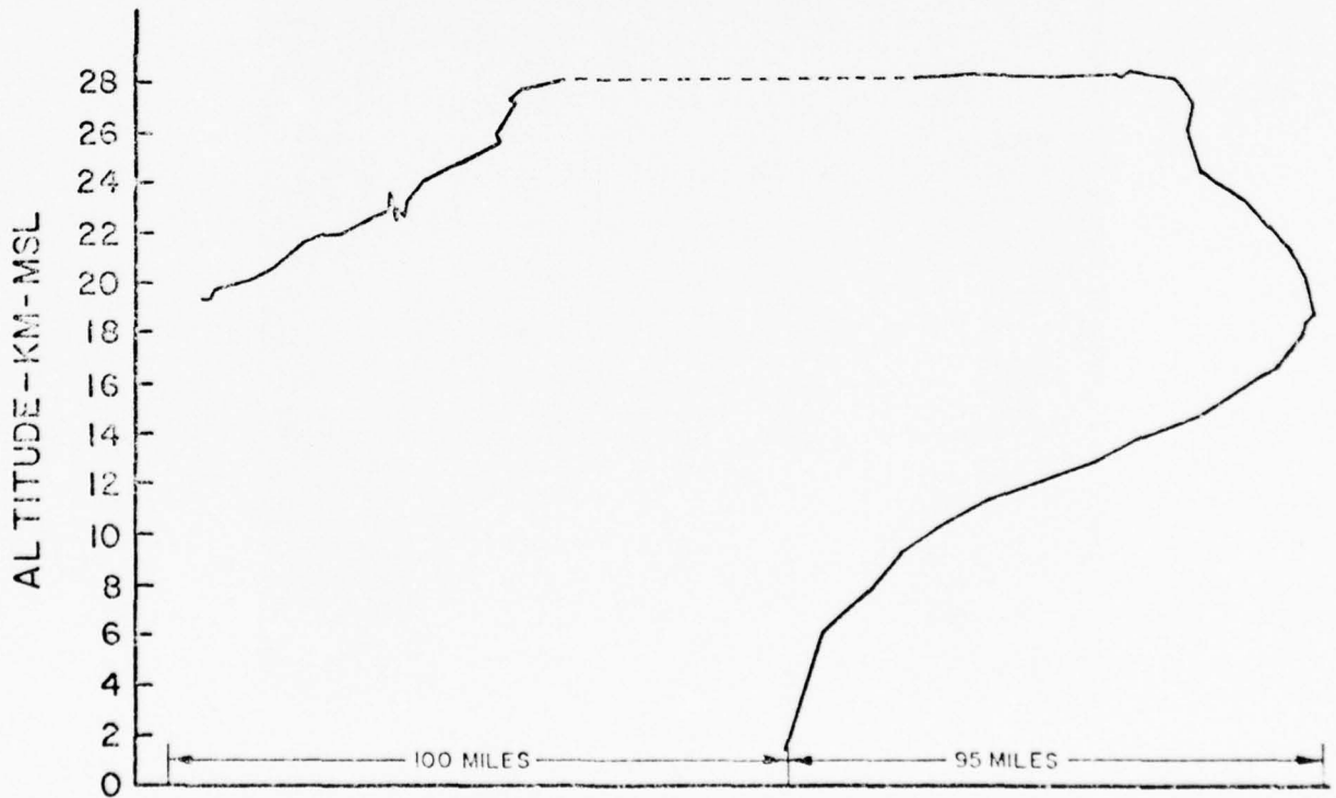
Figure 20. STRATCOM V horizontal trajectory and corresponding balloon altitude vs distance from point of launching - May 1974.
