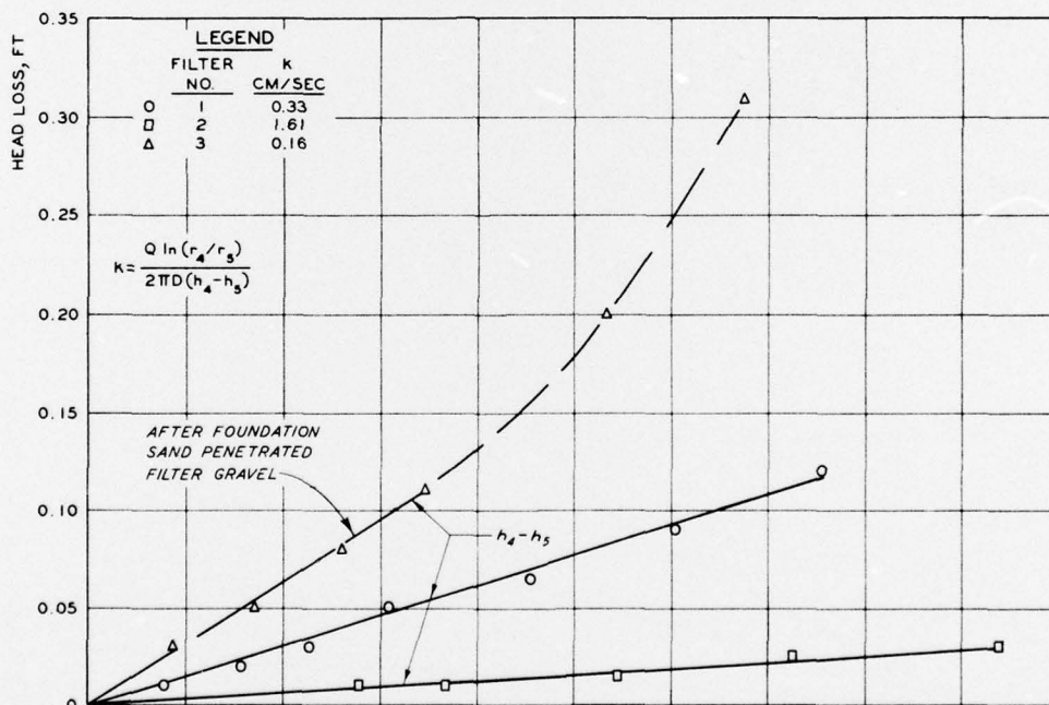
HEAD LOSS IN FILTER GRAVEL (BETWEEN PIEZOMETERS 4 AND 5)
