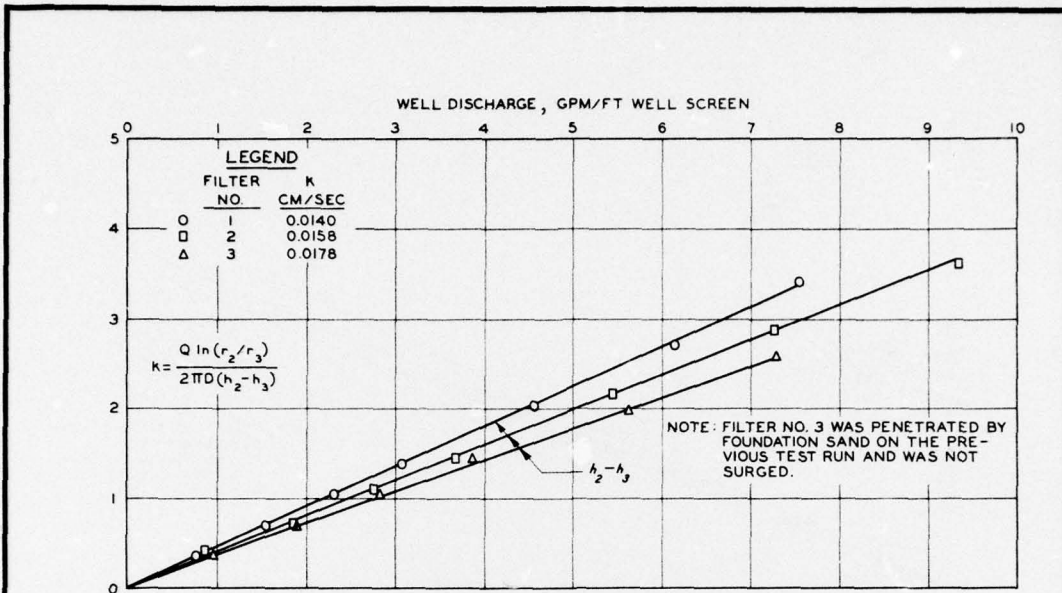
HEAD LOSS IN FOUNDATION SAND (BETWEEN PIEZOMETERS 2 AND 3)
