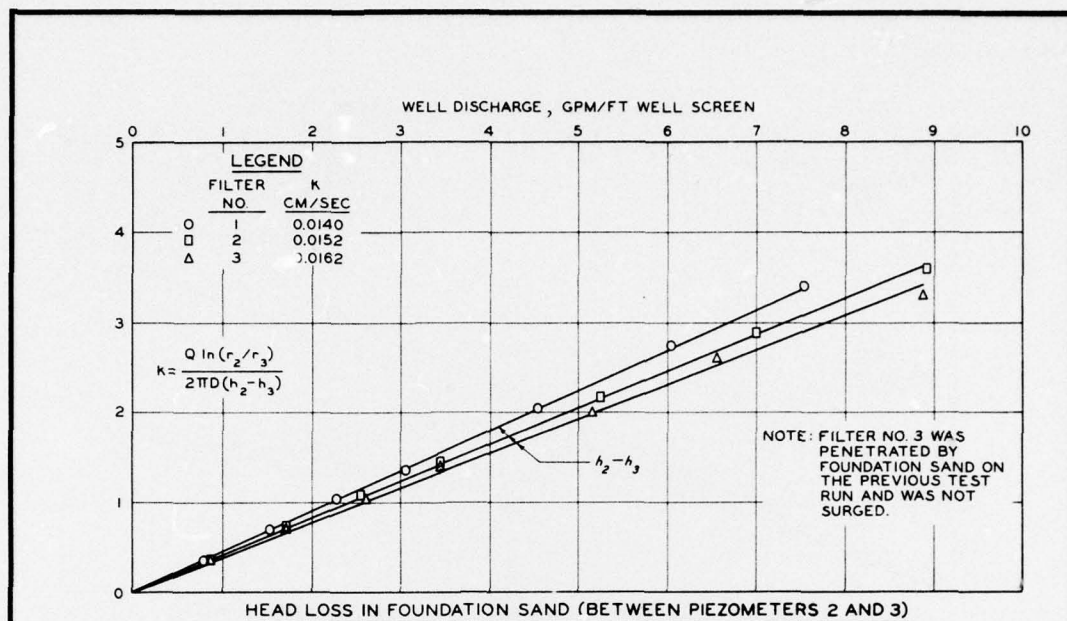
HEAD LOSS IN FOUNDATION SAND (BETWEEN PIEZOMETERS 2 AND 3)
