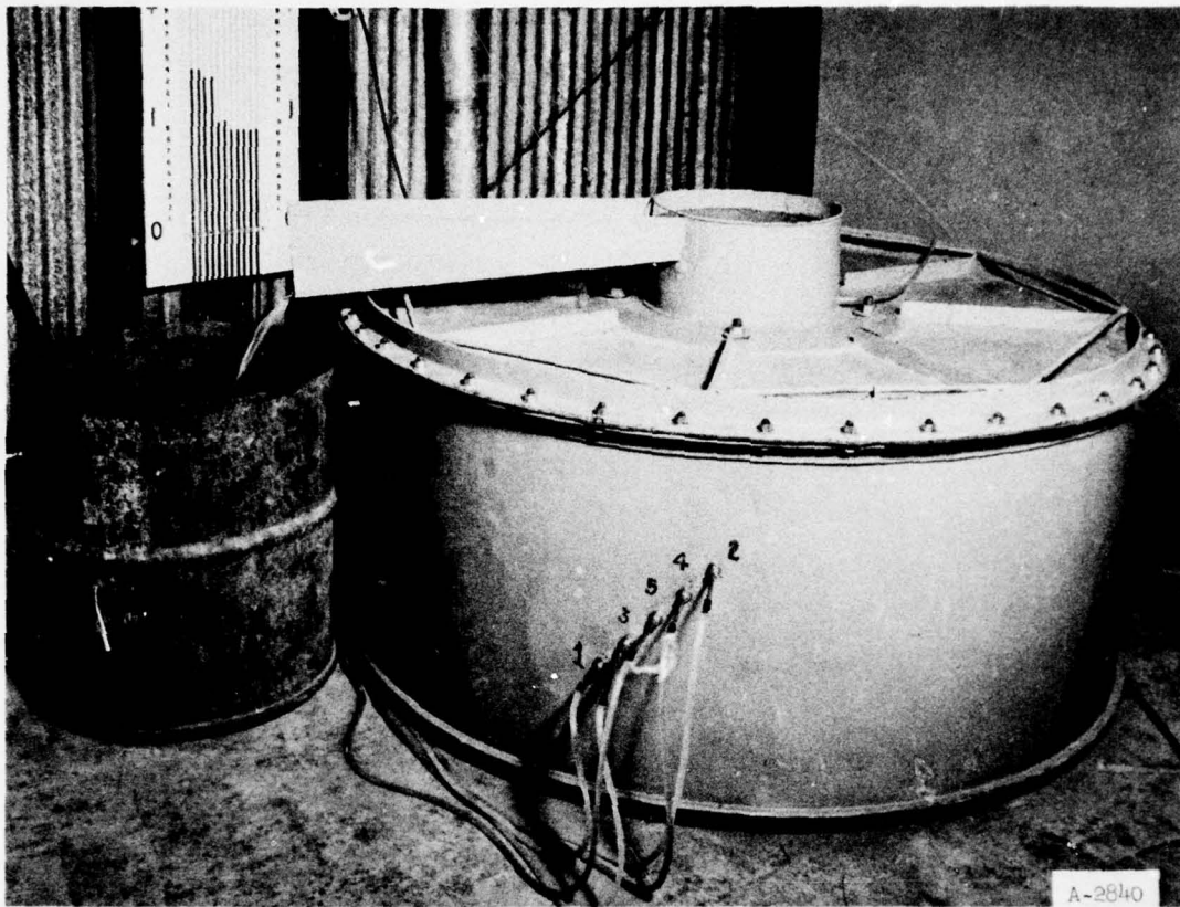
Fig. 3. Well tank in operation
