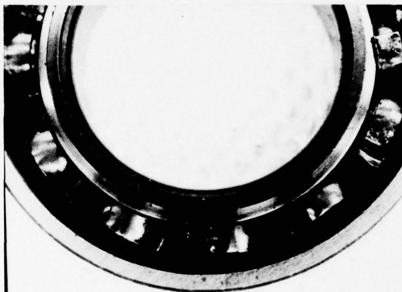
Figure 36. Bearing S/N TRL-11. Removed Position 6 With 4.8 Hours Time. 2.5x Enlarged View.
