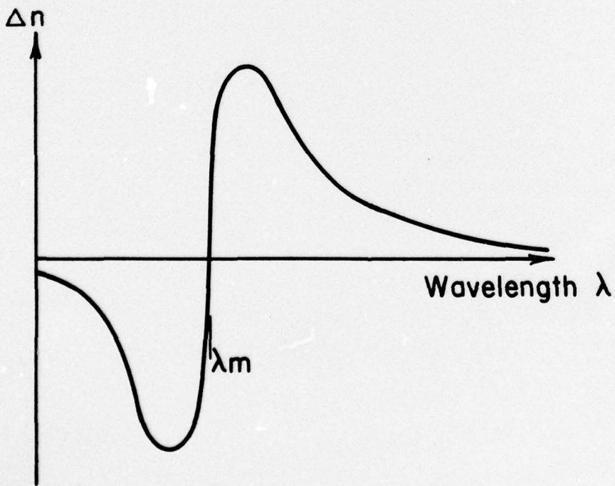
Fig. 2 Contribution of M-centers to optical properties of alkali-halide crystal.
