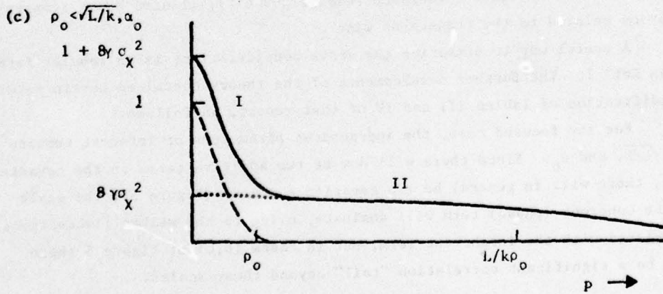
Figure 5. Covariance Curves
