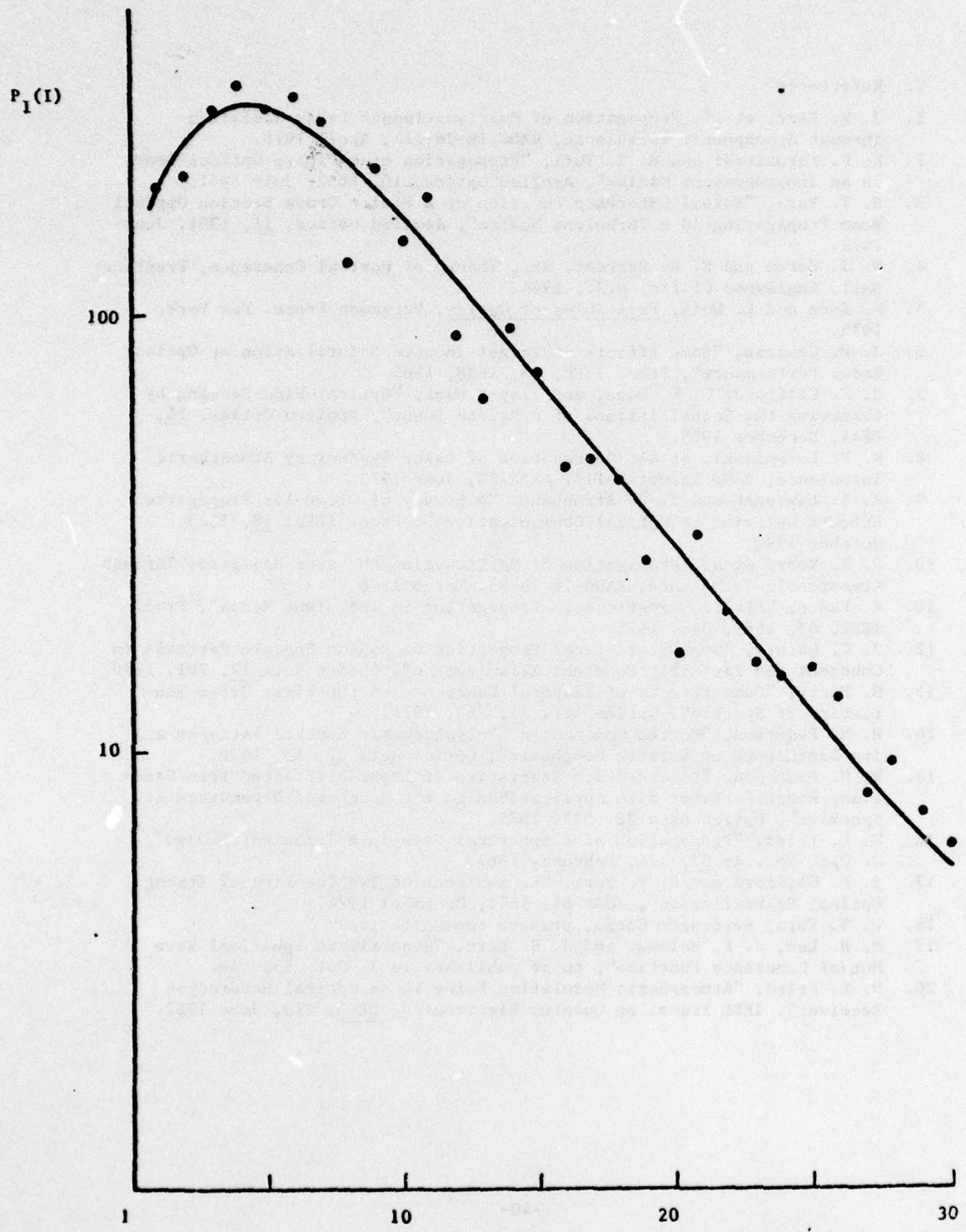
Figure 17. Measured Probability Distribution of Irradiance, Strong Turbulence ( L = 500m, \sigma_{I_N}^2 = 1.2 ).
