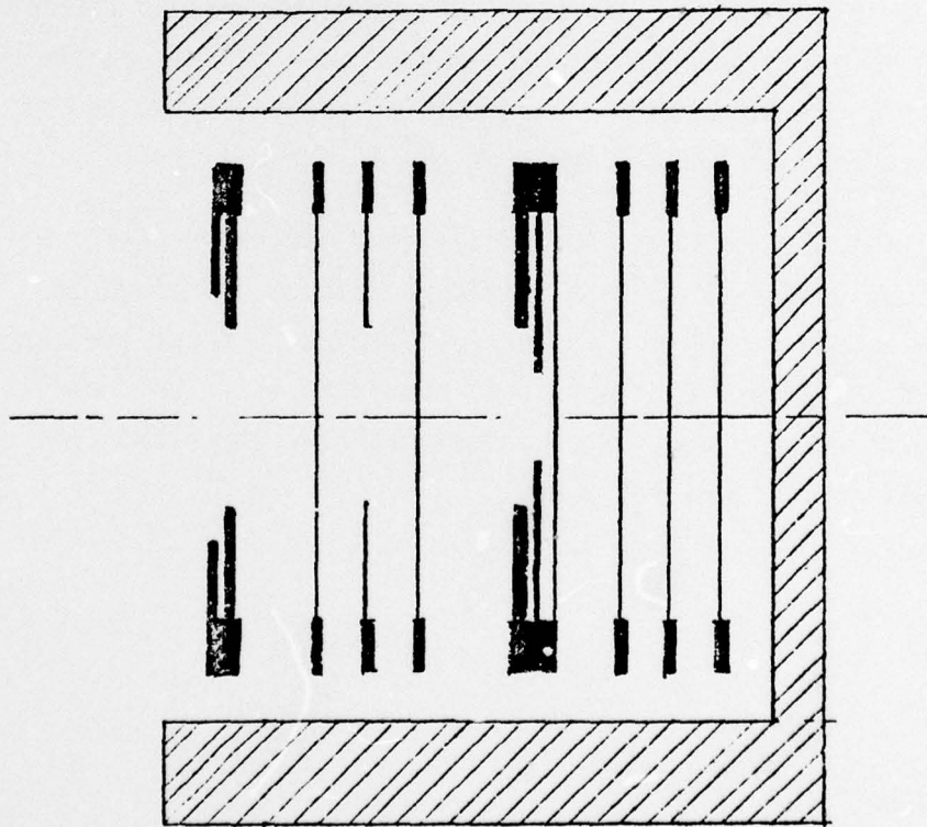
Figure 19. Schematic Plan of the Flat Diode.
