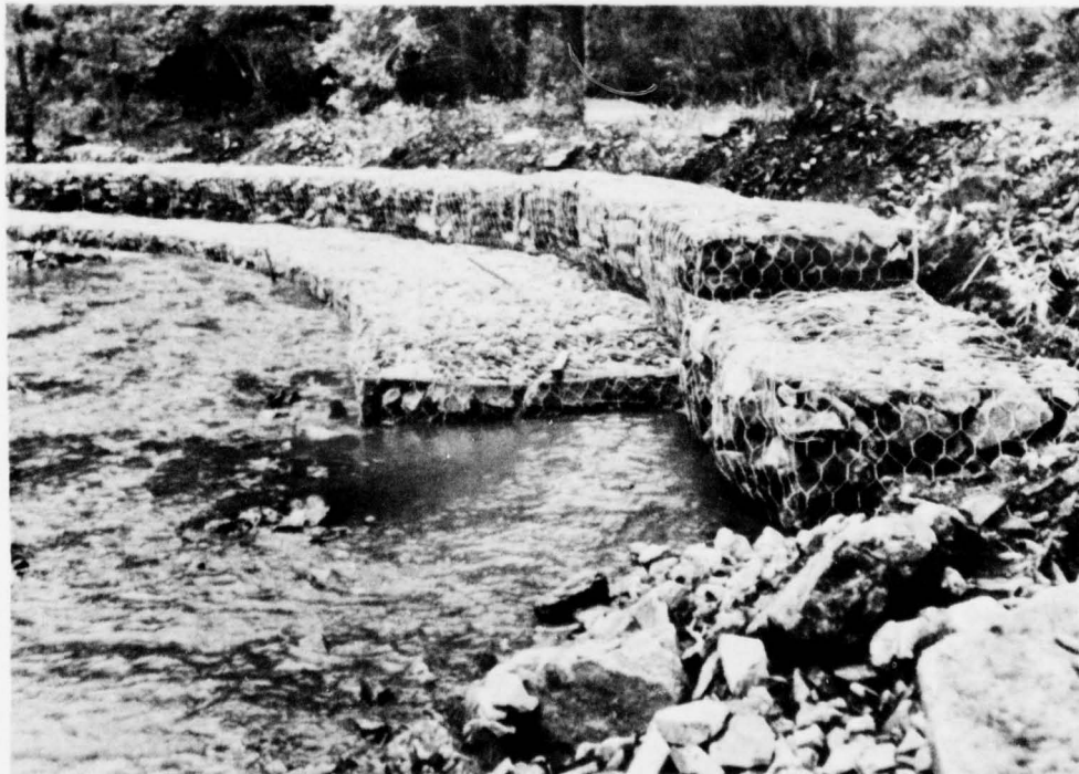
Wire and rock gabions are used to stabilize streambanks. (Forest Service)
