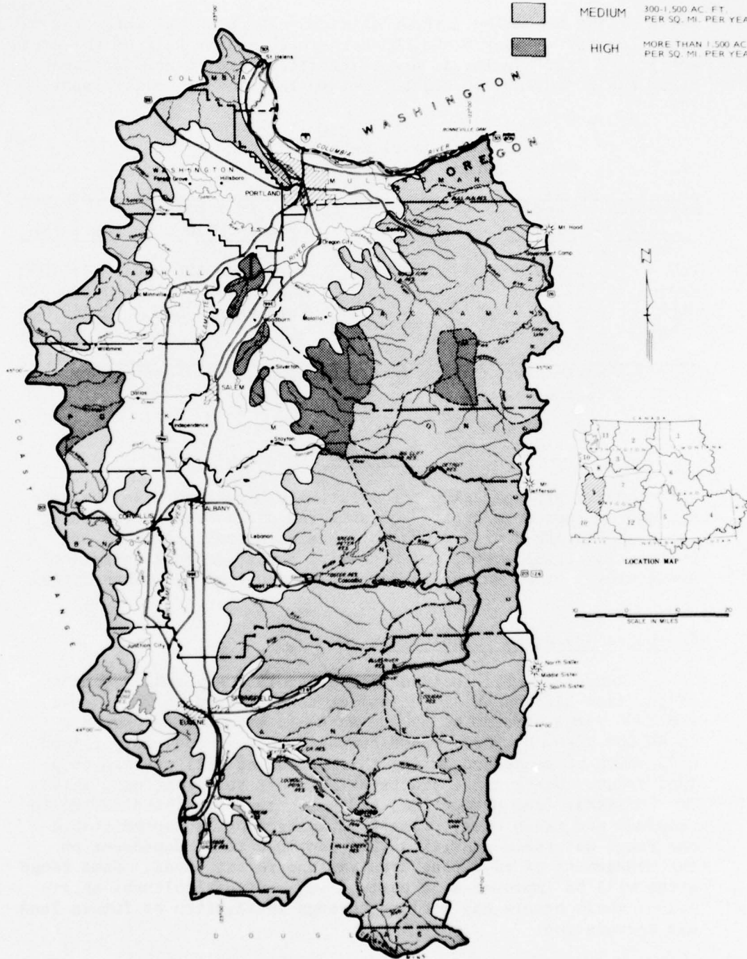
COLUMBIA-NORTH PACIFIC COMPREHENSIVE FRAMEWORK STUDY WATER RETENTION CAPACITY FOREST LAND WILLAMETTE, SUBREGION 9 1968
