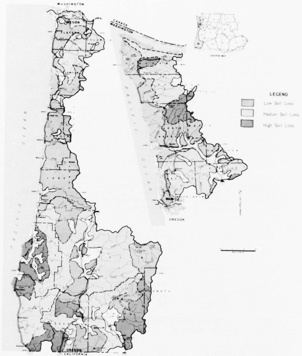
COLUMBIA-NORTH PACIFIC COMPREHENSIVE FRAMEWORK STUDY POTENTIAL EROSION HAZARD FOREST LAND COASTAL, SUBREGION 10 1968
