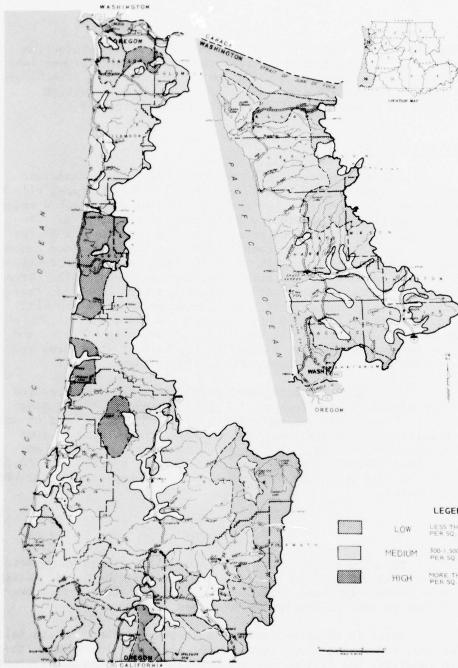
COLUMBIA-NORTH PACIFIC COMPREHENSIVE FRAMEWORK STUDY WATER RETENTION CAPACITY FOREST LAND COASTAL, SUBREGION 10
