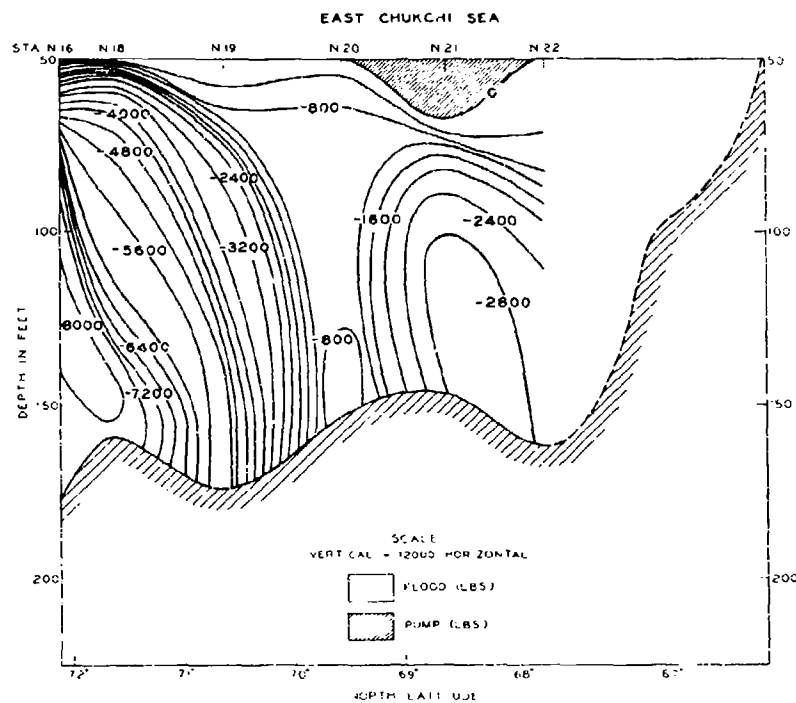
Figure 18-b. Computed buoyancy changes, 2100-ton submarine, section along approximate line from 72°N 170°W to Cape Lisburne, thence along shore to Kotzebue Sound.
