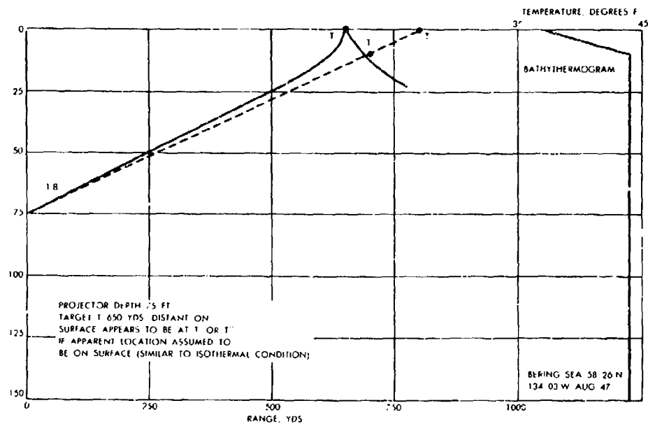
Figure 62. Ray diagram.
