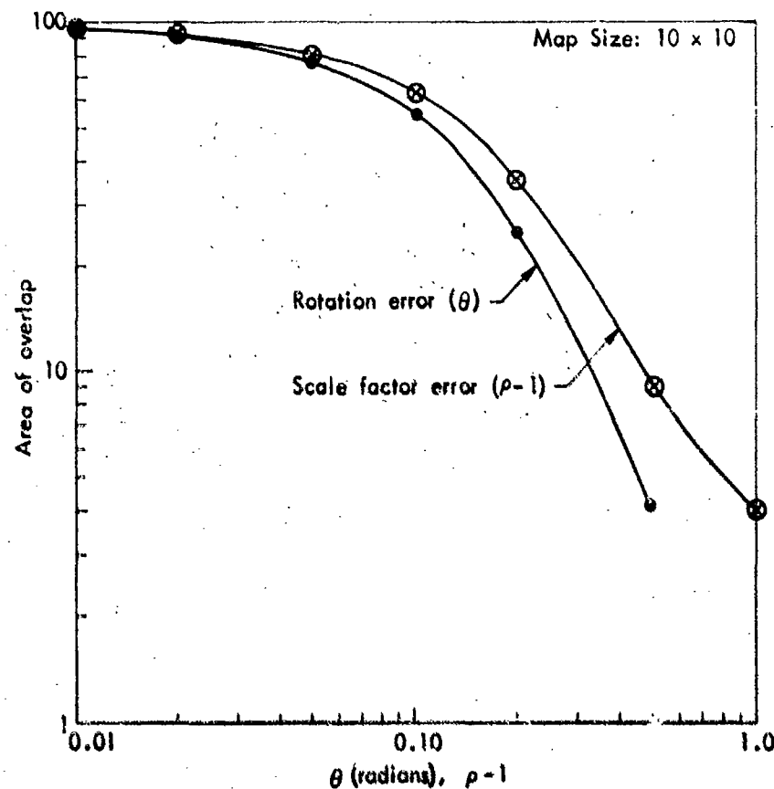
Fig. 15—Comparison of the relative magnitude of the correlation peak for scale factor and rotation errors
