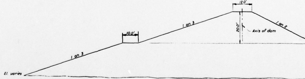
TYPICAL EMBANKMENT SECTION
