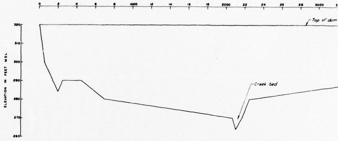
PROFILE OF DAM
