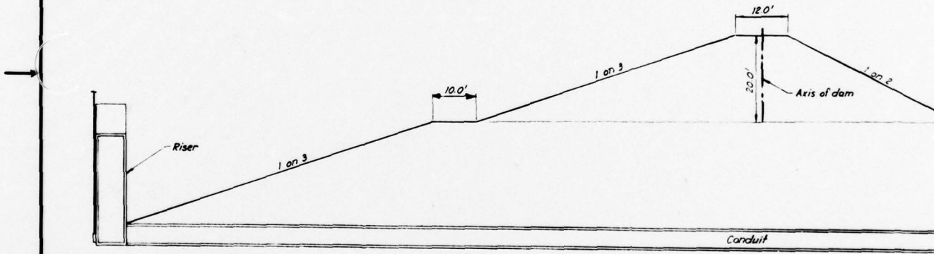
CULVERT SECTION
