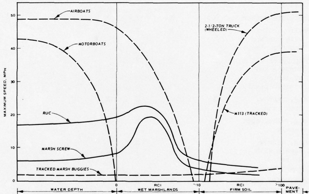
Figure 10. Comparison of relative performances of selected vehicles
