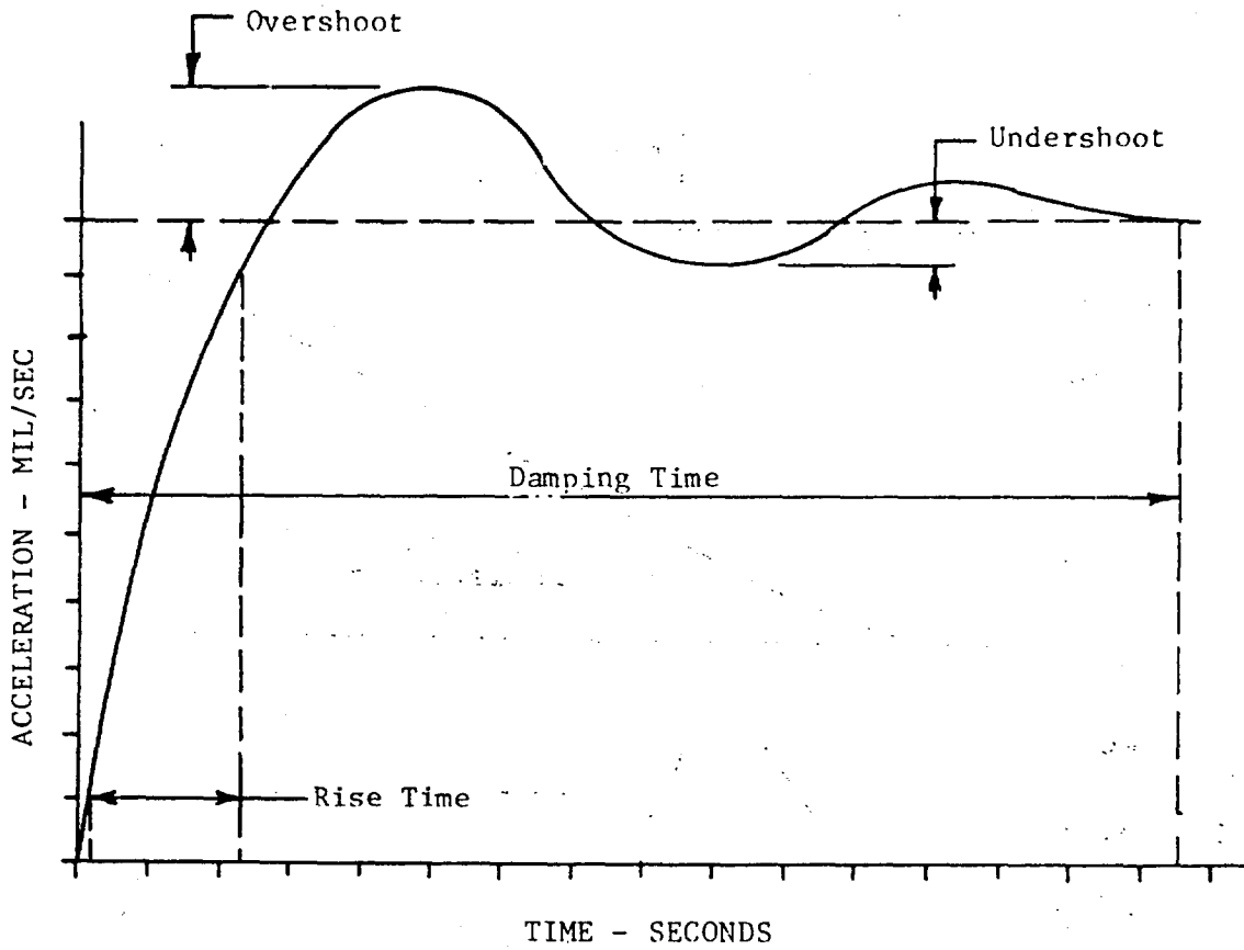
Figure 3. Acceleration Characteristics.
