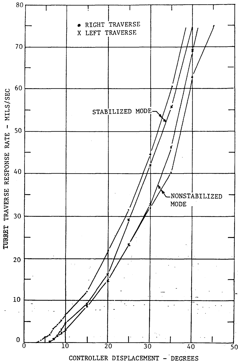
Figure 1. Turret Traverse Response Rate Characteristics, Commander's Control.
