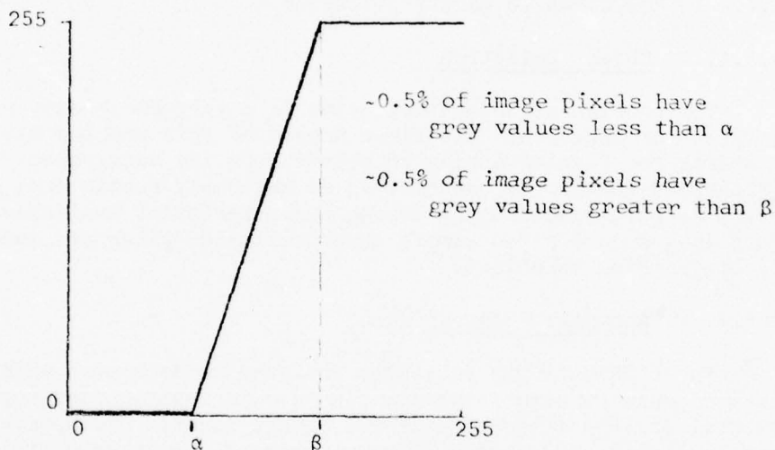
Figure 4-1. Transfer Function Used for Range Change
