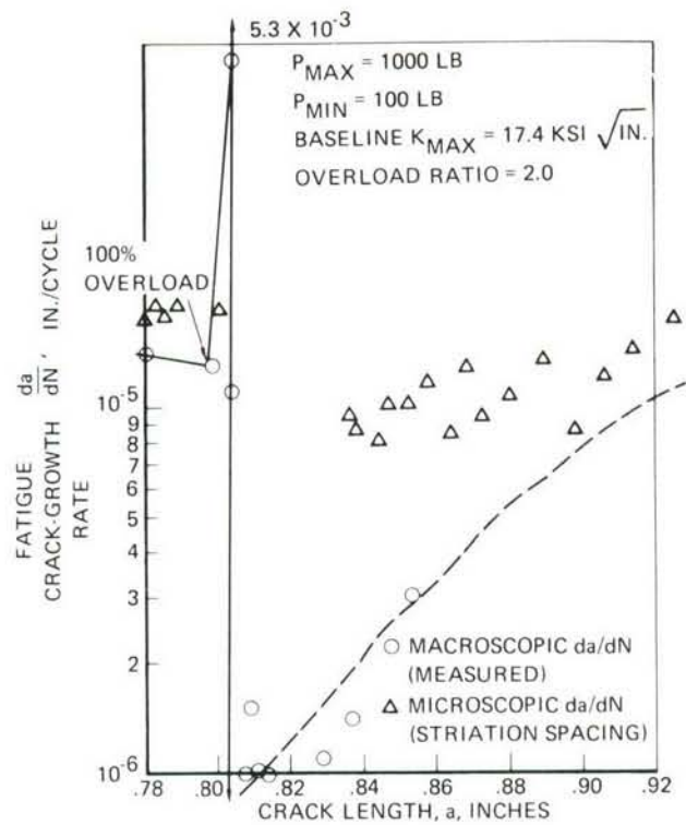
(a) 2024-T3
