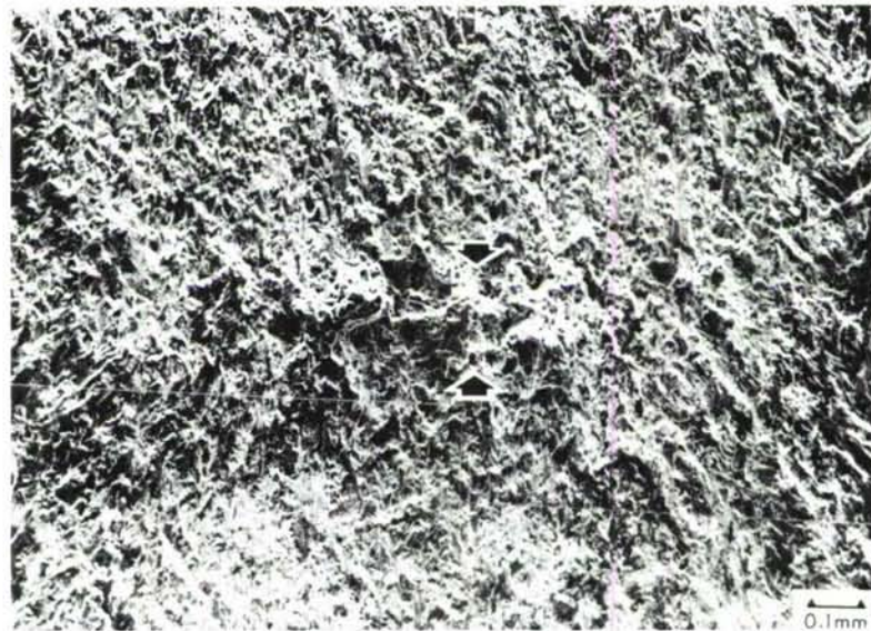
(c) K_{MAX} = 12.3 \text{ KSI } \sqrt{\text{IN.}} CRACK LENGTH AT OVERLOAD = 1.03 IN.
