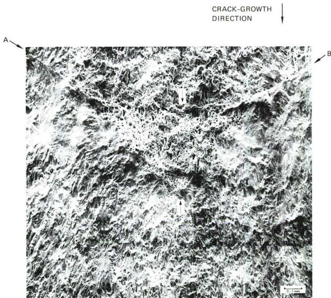
(b) 7075-T73
