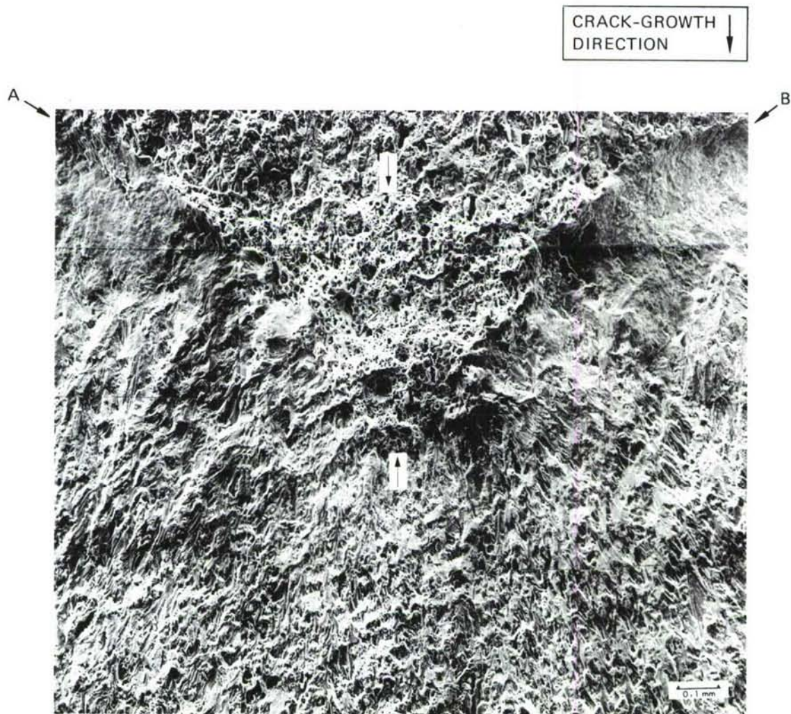
(a) 7075-T6
