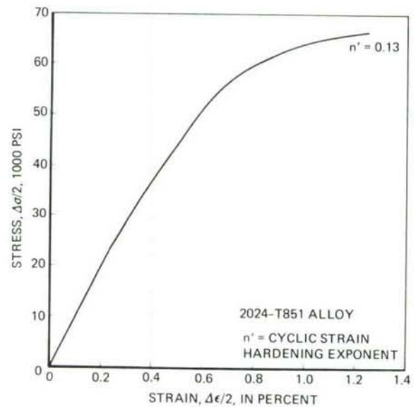
(b) 2024-T851
