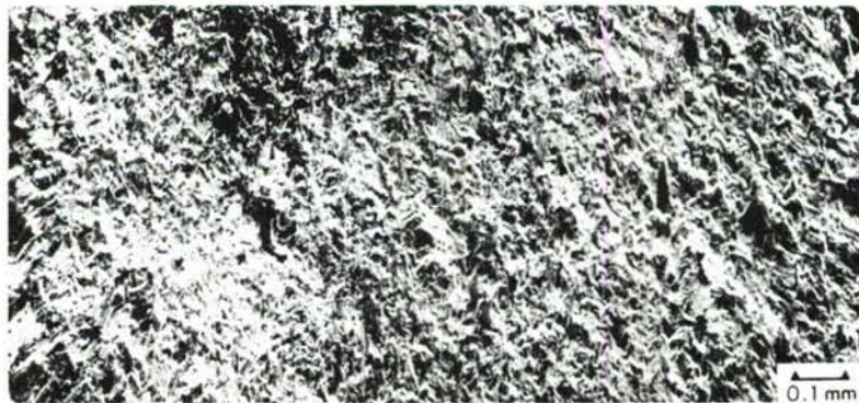
(b) K_{MAX} = 8.7 \text{ KSI } \sqrt{\text{IN.}} CRACK LENGTH AT OVERLOAD = 0.80 IN.
