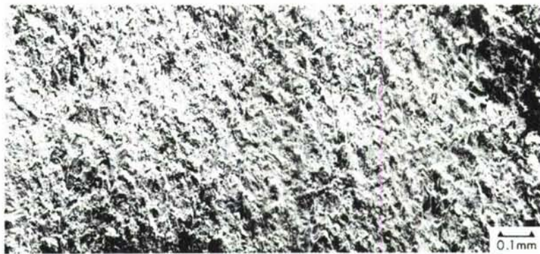
(a) K_{MAX} = 6.1 \text{ KSI } \sqrt{\text{IN.}} CRACK LENGTH AT OVERLOAD = 0.57 IN.
