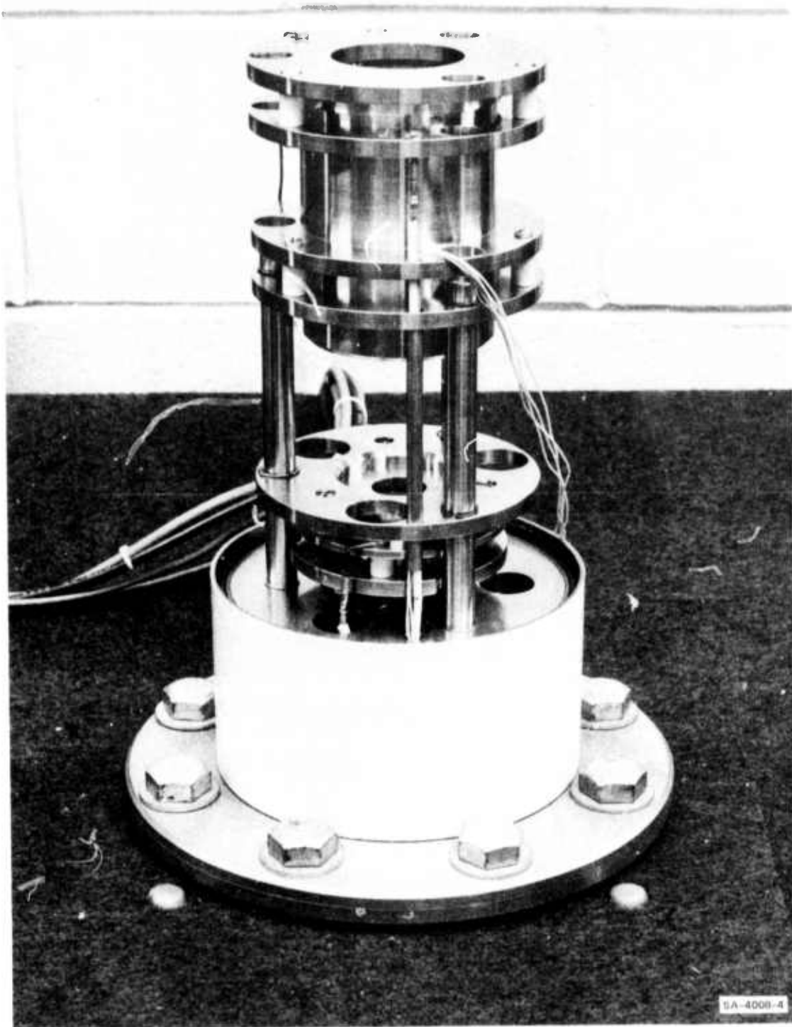
FIGURE 4 ELECTRON GUN
