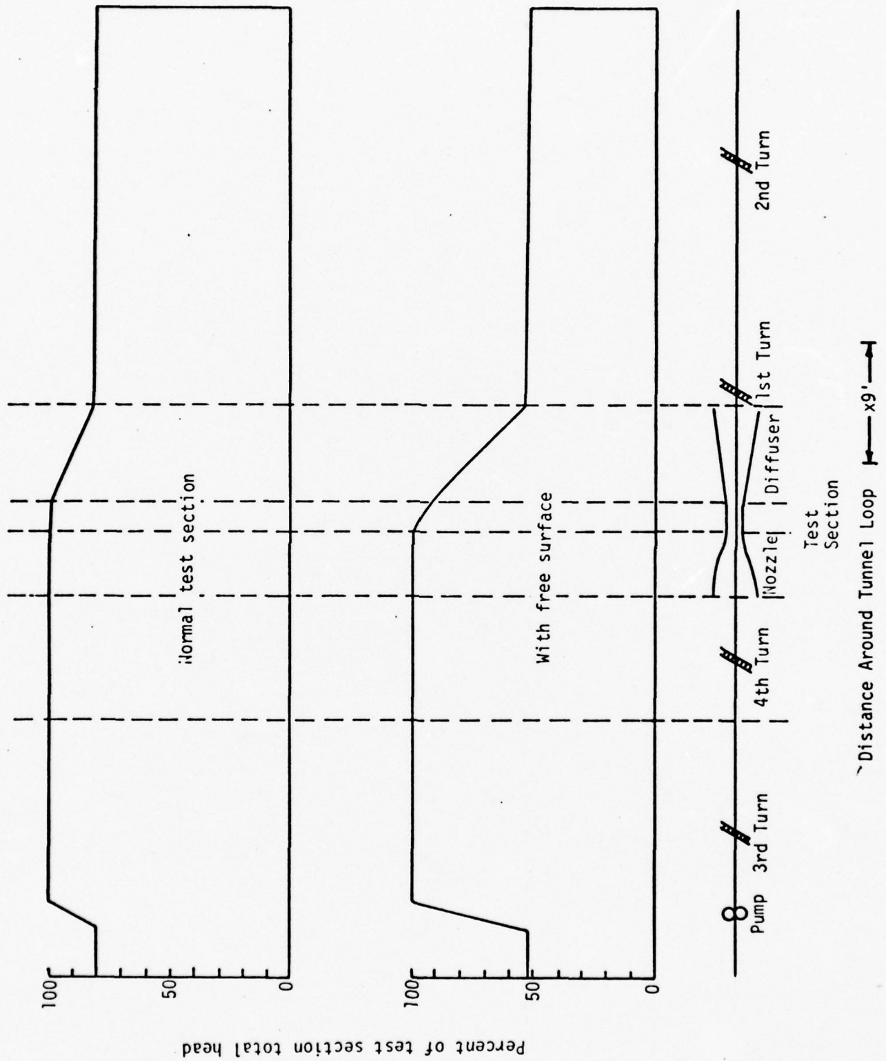
Figure 3 - Nondimensionalized Energy Lines Around the Tunnel Loop
