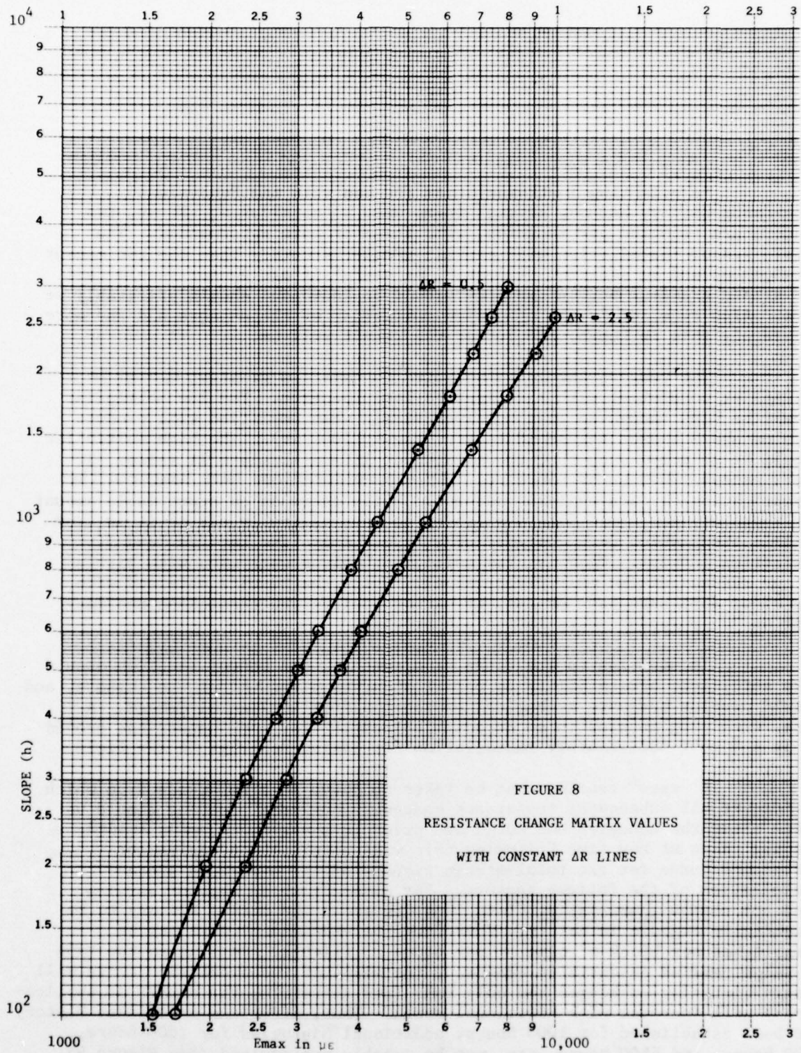
Figure 8 - Resistance Change Matrix Values with Constant Resistance Change ( \Delta R )
