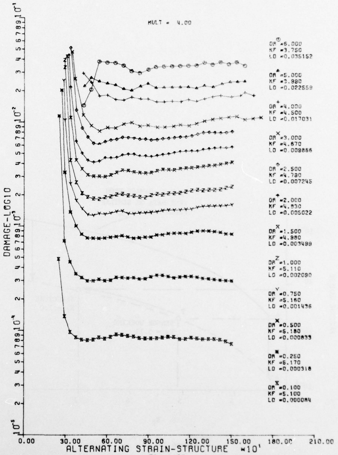
Figure 15 "Best Fit" Constant Damage Values
