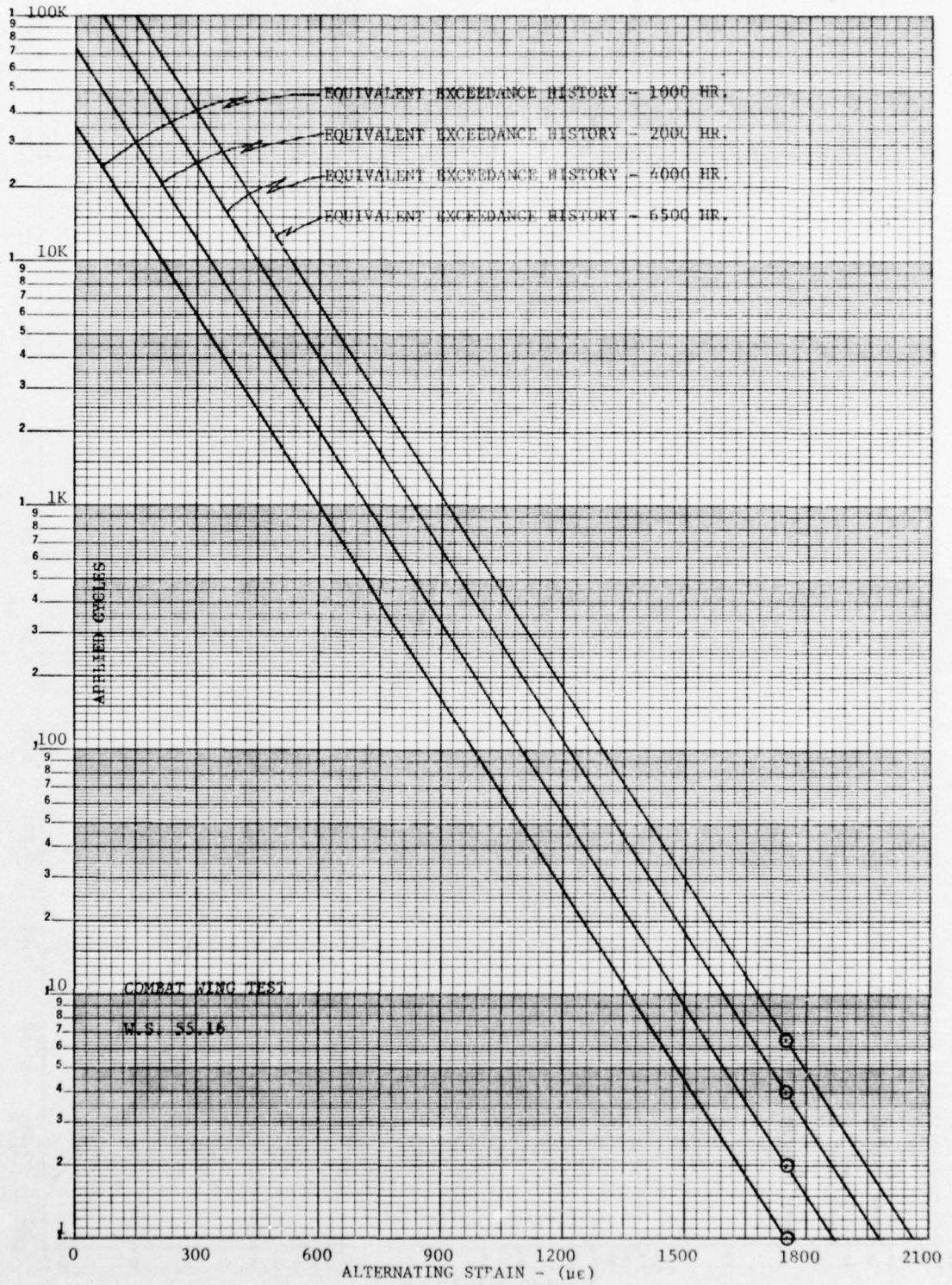
Figure 9 - Equivalent Exceedance History at Increments of Life
