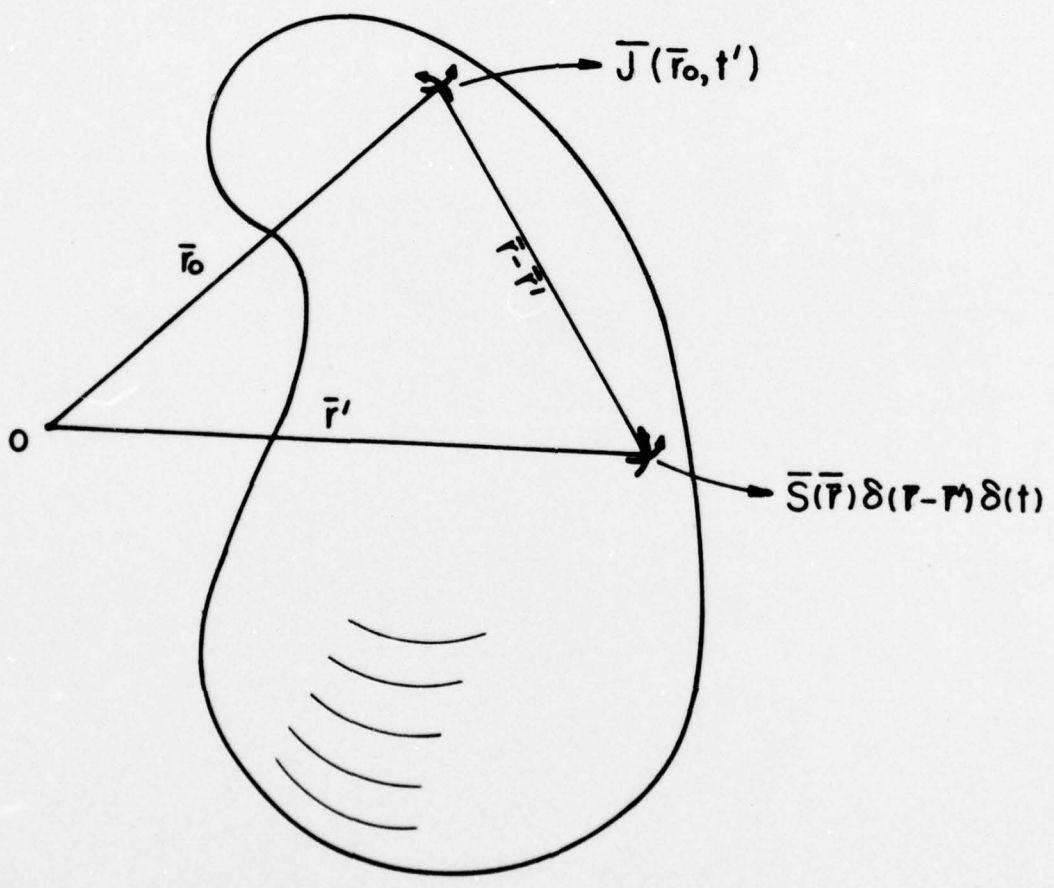
Figure 2.8. Geometry for discussion of asymptotic form of \bar{\Gamma}^{-1}(\bar{r}, \bar{r}', s) .
