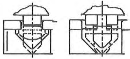
Standard Twist Locks
