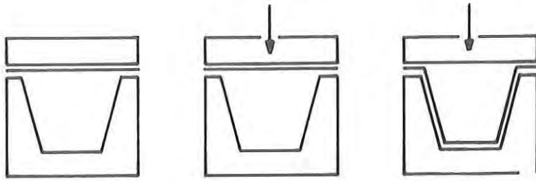
Figure 10. Trapped Sheet, Contact Heat, Pressure Forming
