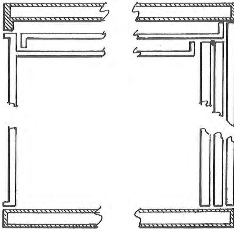
Figure 58. Longitudinal Section, Container Mode
