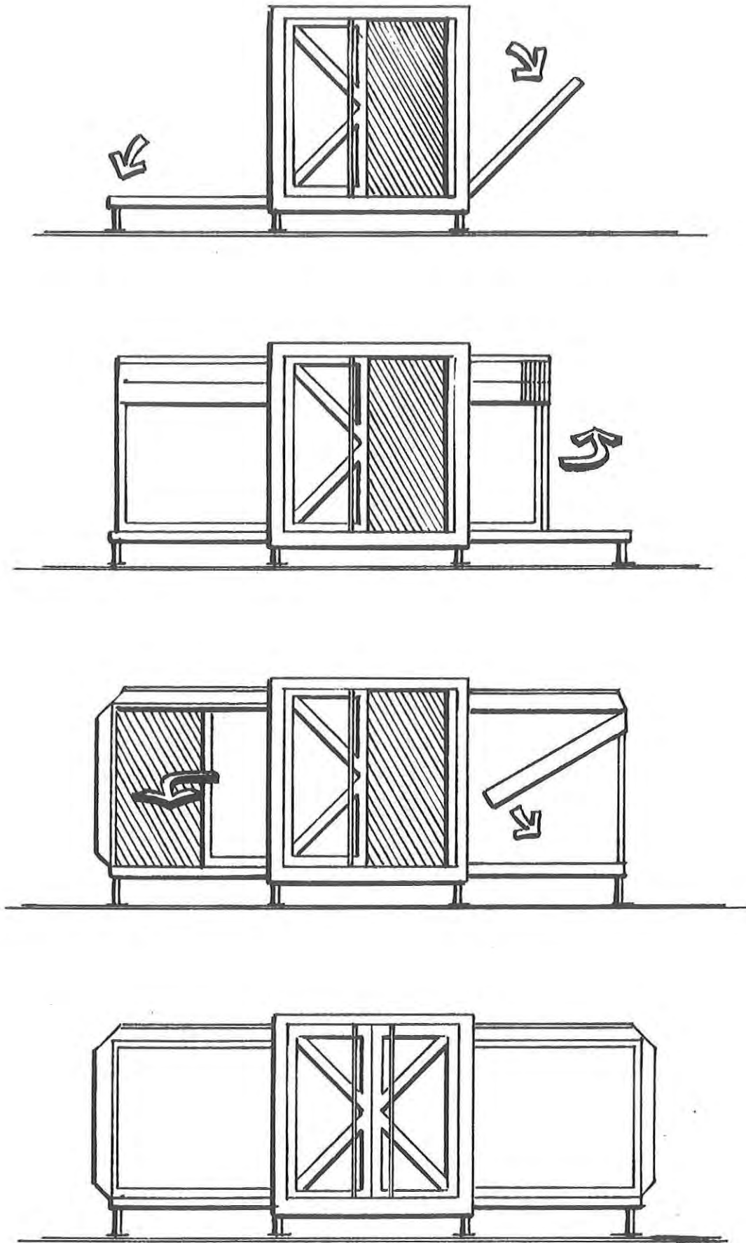
Figure 75. Expansion Procedure
