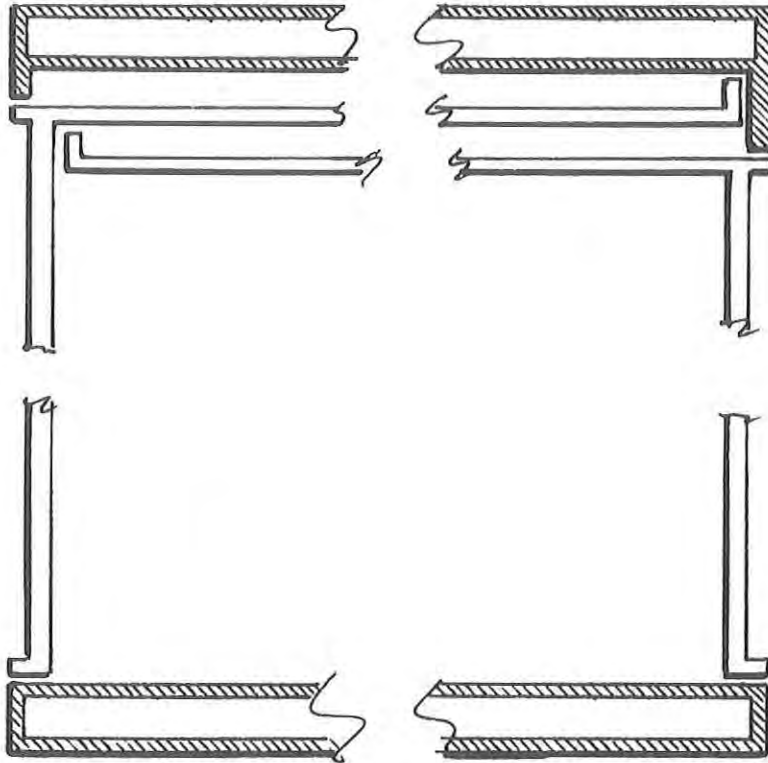
Figure 94. Longitudinal Section Container Mode
