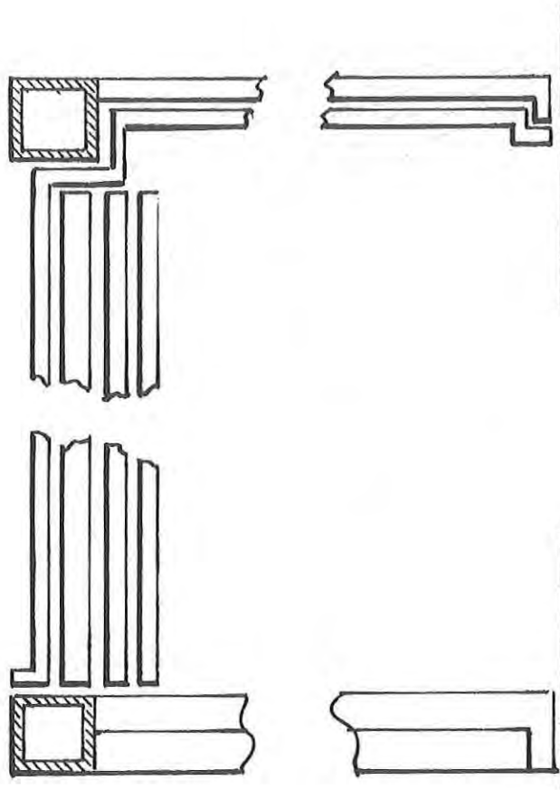
Figure 64. Longitudinal Section, Container Mode
