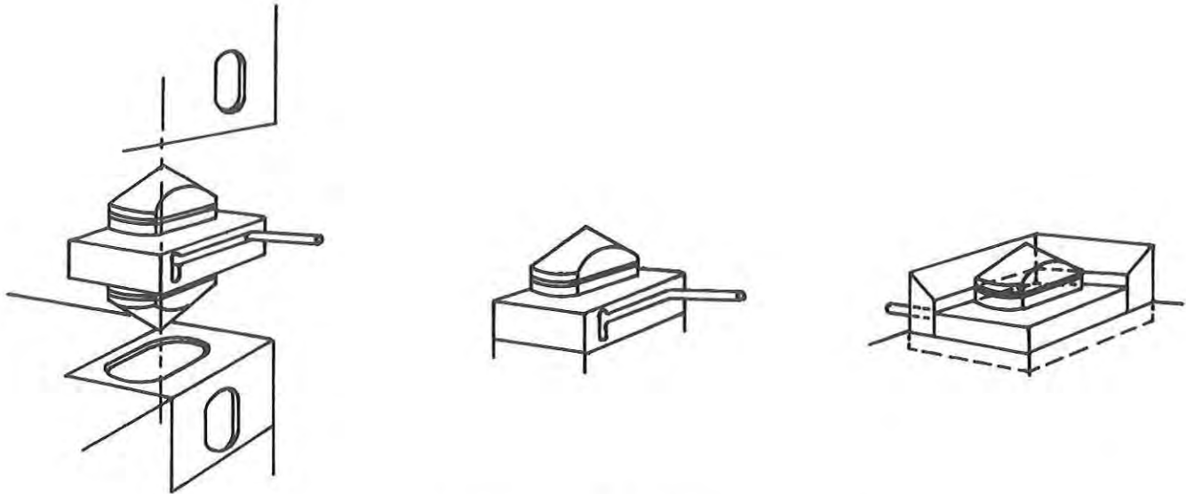
Twist Lock Types
