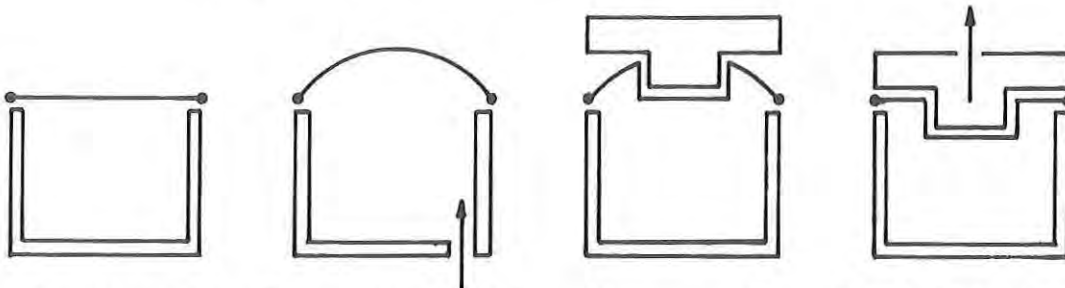
Figure 12. Pressure Bubble, Vacuum, Snap-Back Forming
