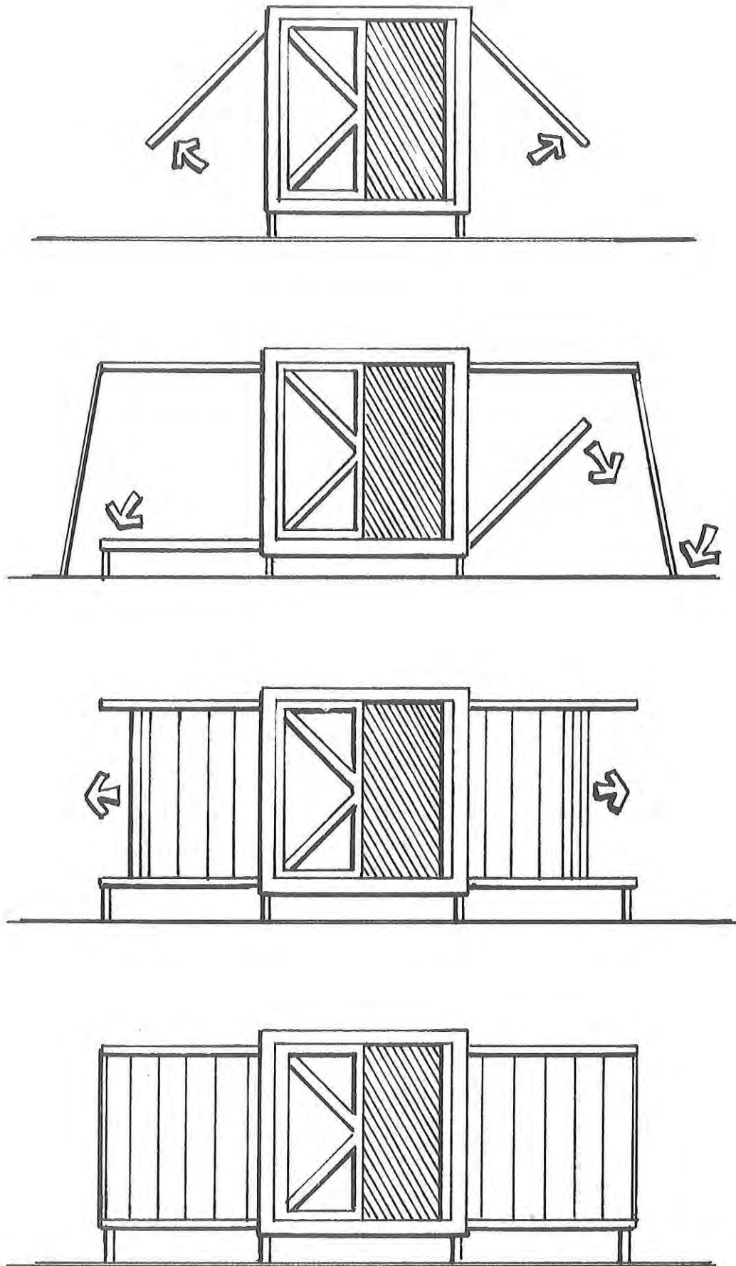
Figure 84. Expansion Procedure
