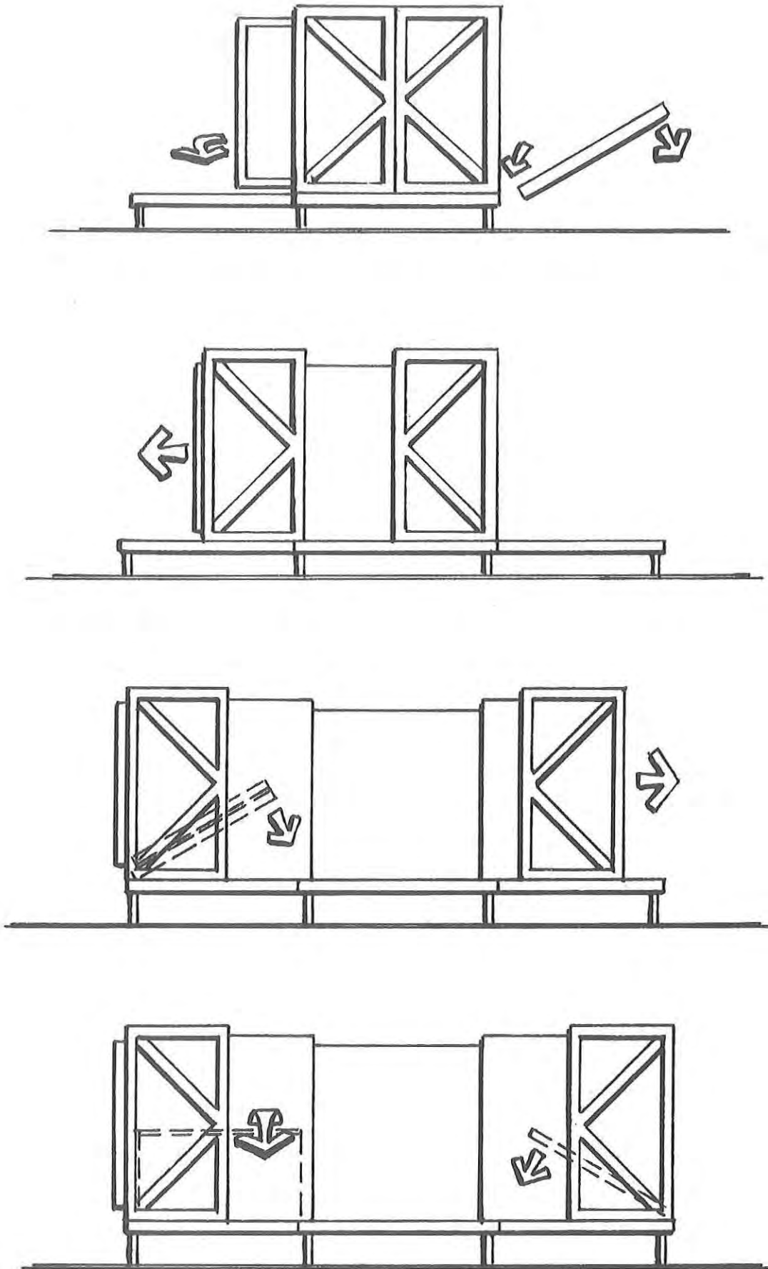
Figure 60. Expansion Procedure
