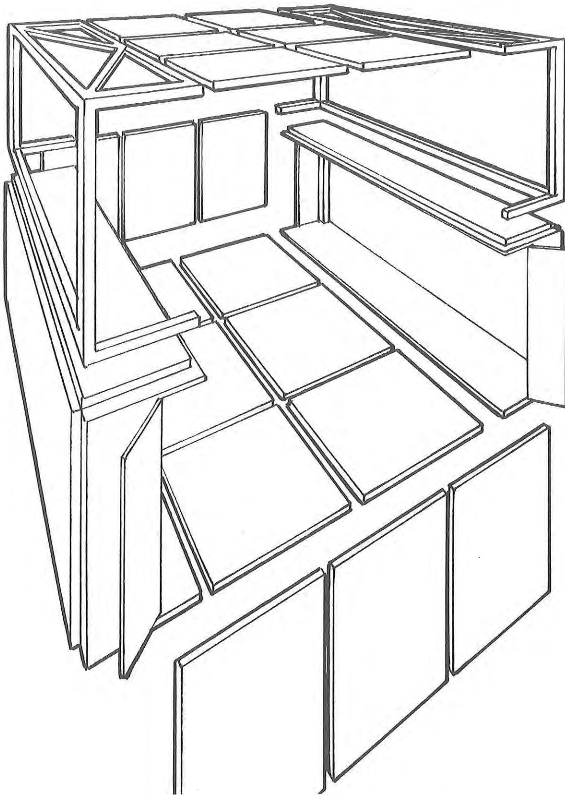
Figure 62. Configuration G
