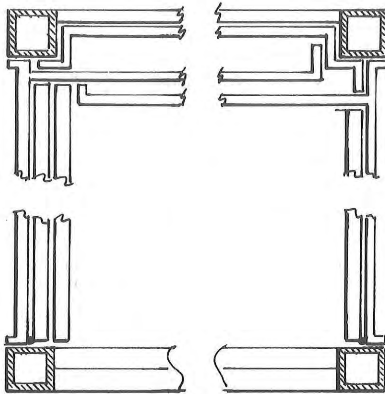
Figure 51. Longitudinal Section, Container Mode
