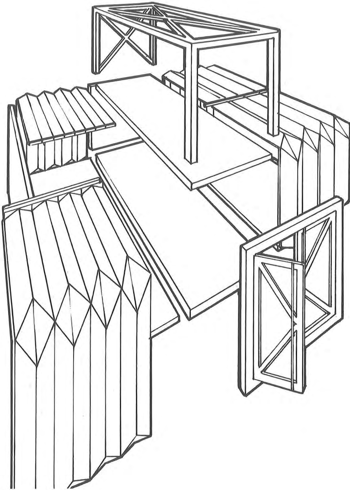
Figure 71. Configuration J
