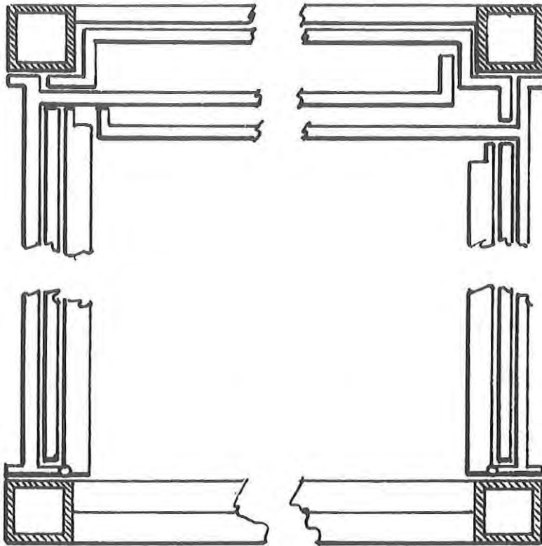
Figure 47. Longitudinal Section, Container Mode
