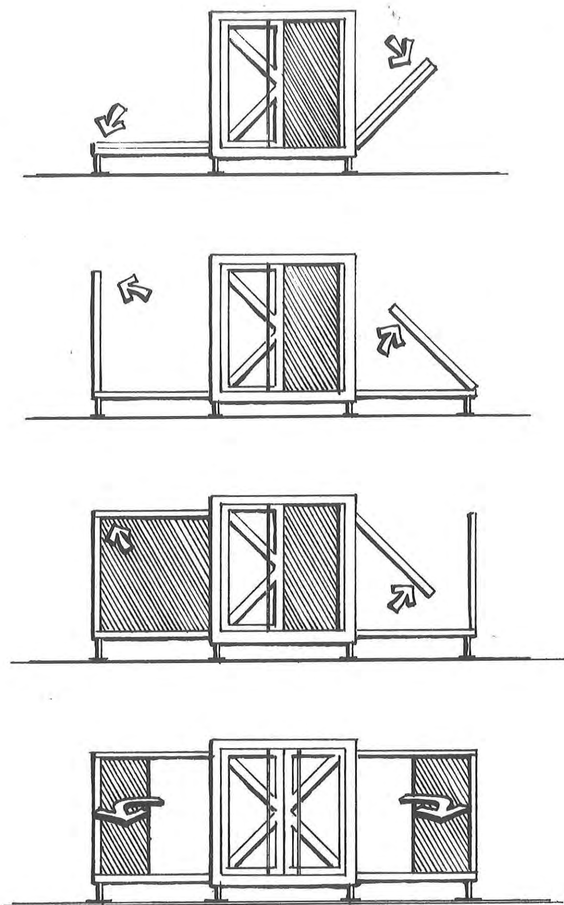
Figure 43. Expansion Procedure
