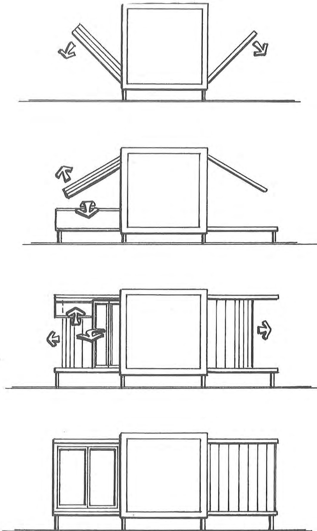
Figure 81. Expansion Procedure
