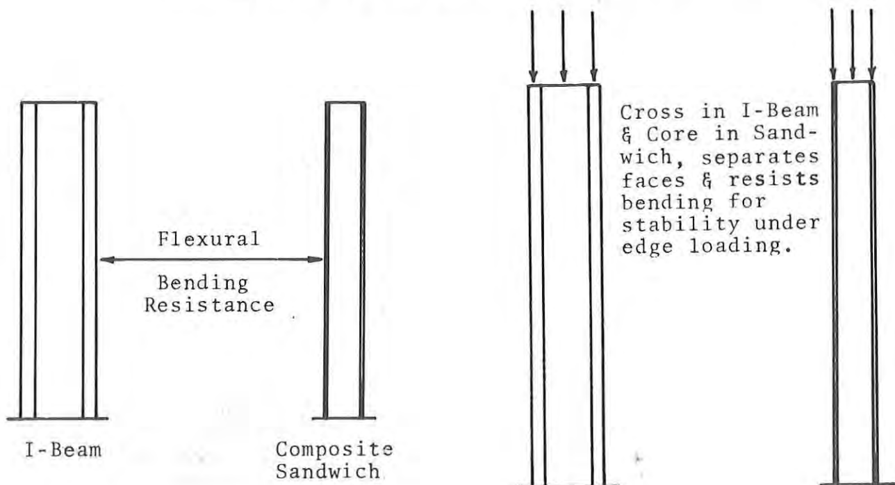
Figure 25. Sandwich Panel Strength
