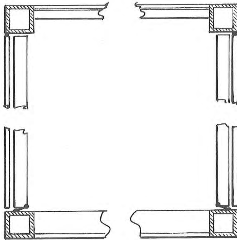
Figure 85. Longitudinal Section, Container Mode
