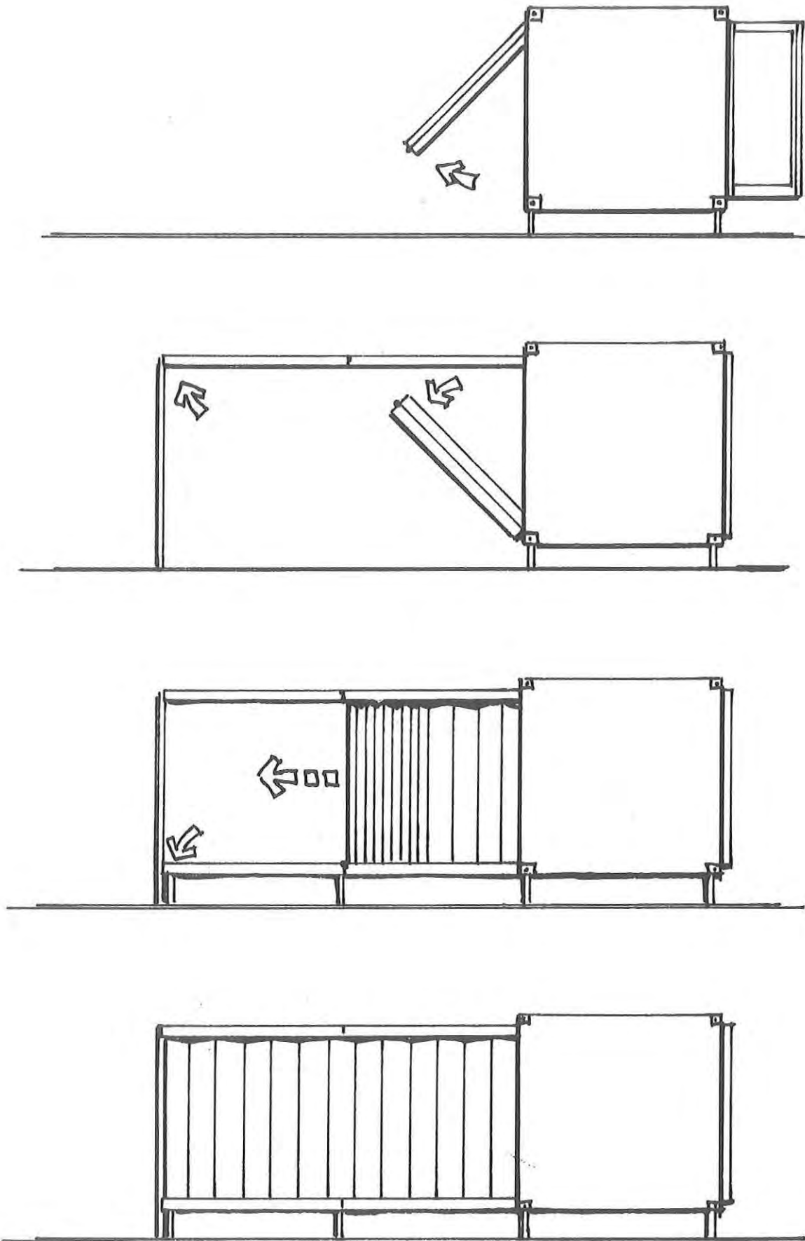
Figure 87. Expansion Procedure
