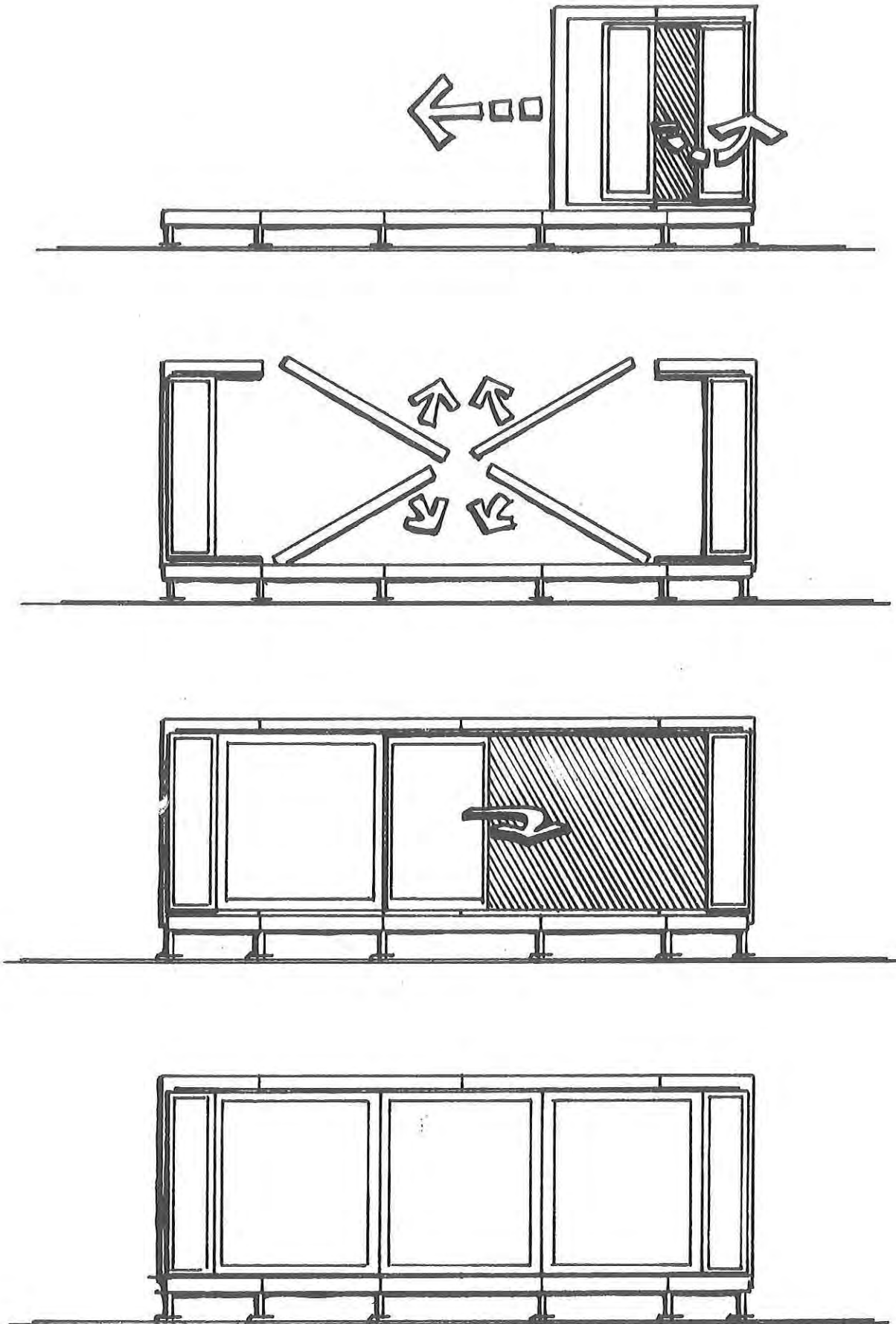
Figure 63. Expansion Procedure
