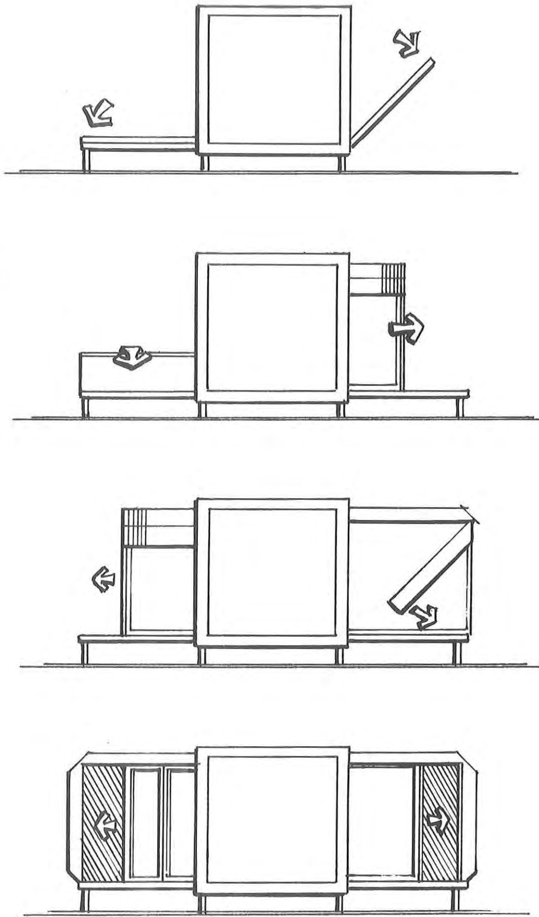
Figure 78. Expansion Procedure
