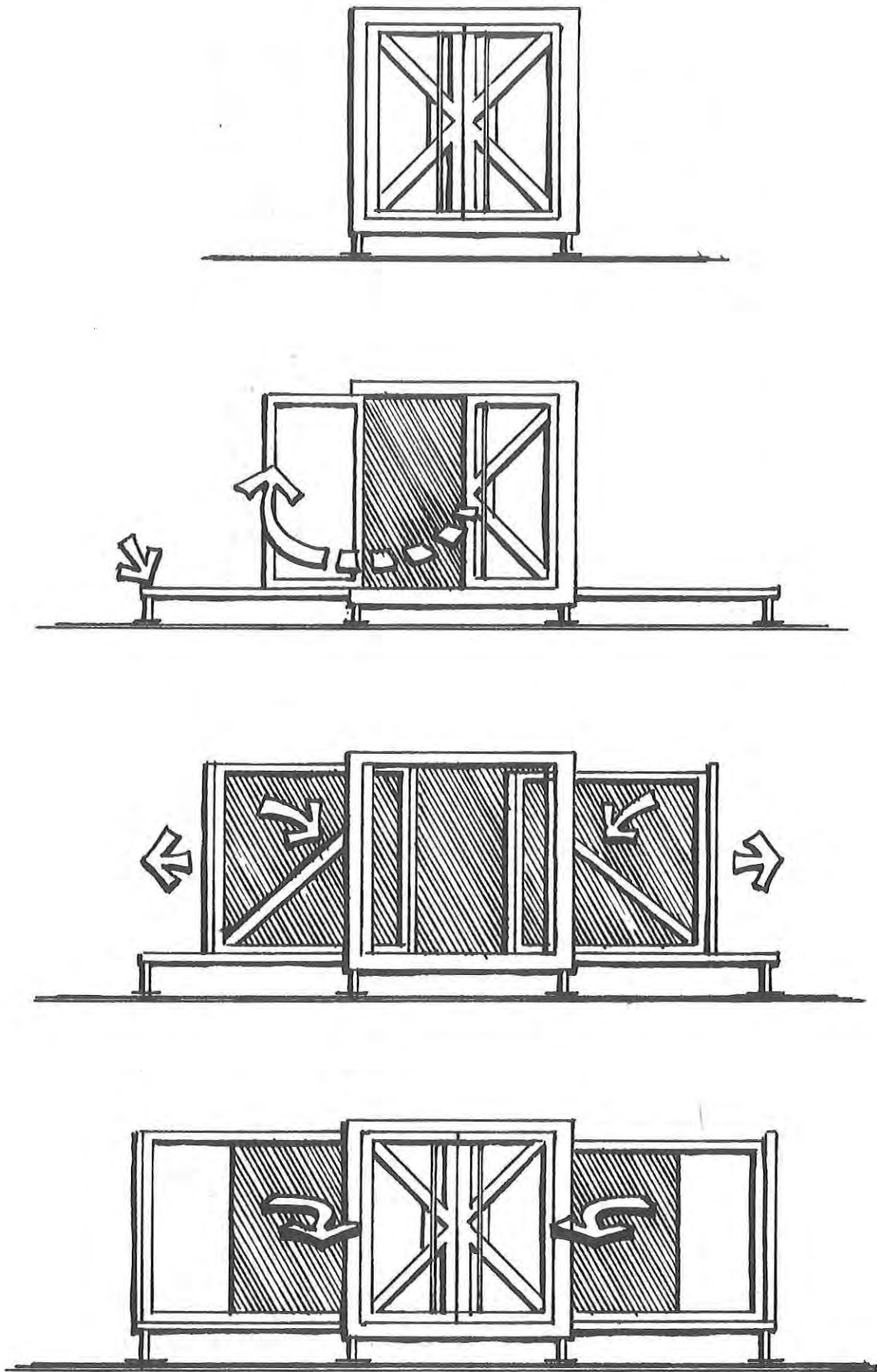
Figure 46. Expansion Procedure
