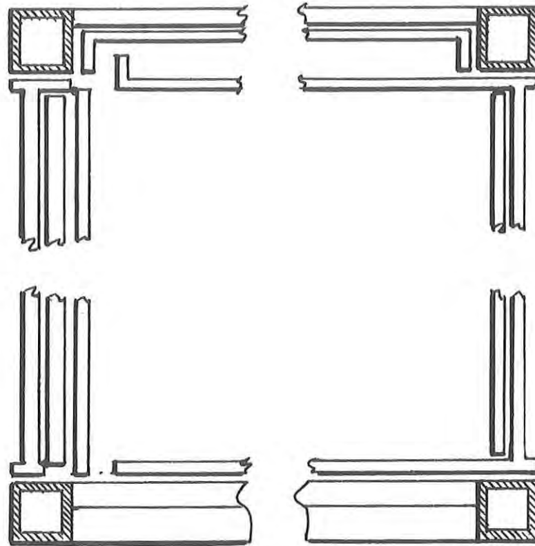
Figure 91. Longitudinal Section, Container Mode
