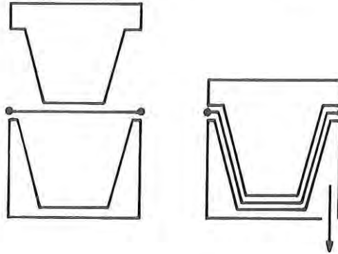
Figure 6. Matched Mold Forming
