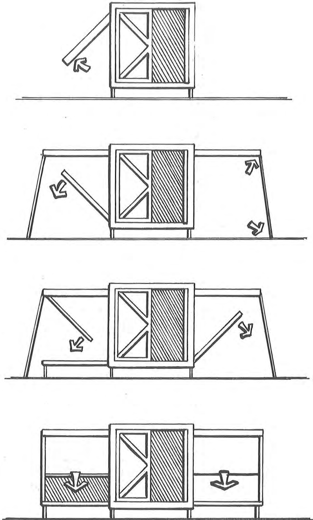
Figure 69. Expansion Procedure
