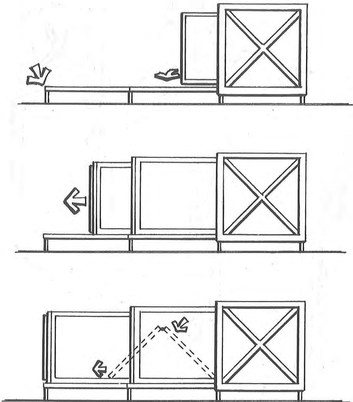
Figure 57. Expansion Procedure
