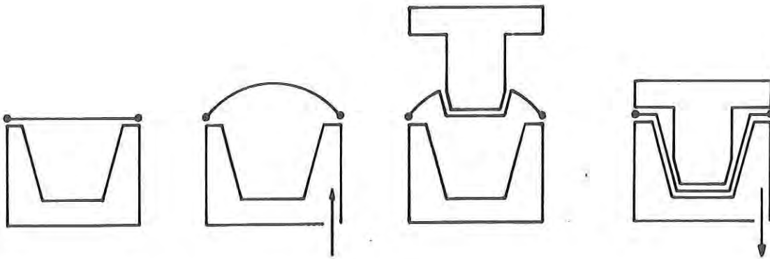
Figure 7. Pressure Bubble, Plug Assist Forming
