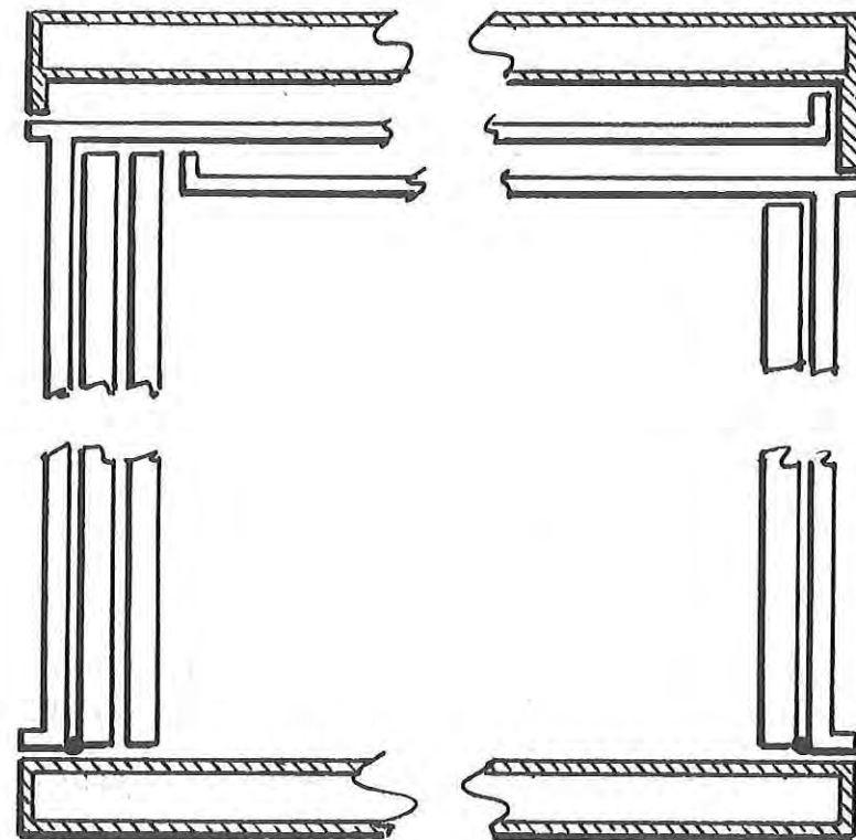
Figure 52. Longitudinal Section, Container Mode
