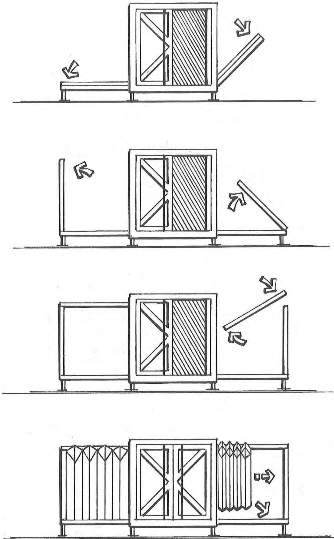
Figure 72. Expansion Procedure
