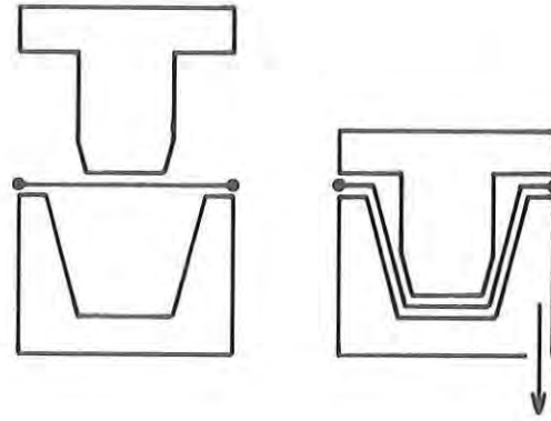
Figure 8. Plug Assist Vacuum Forming
