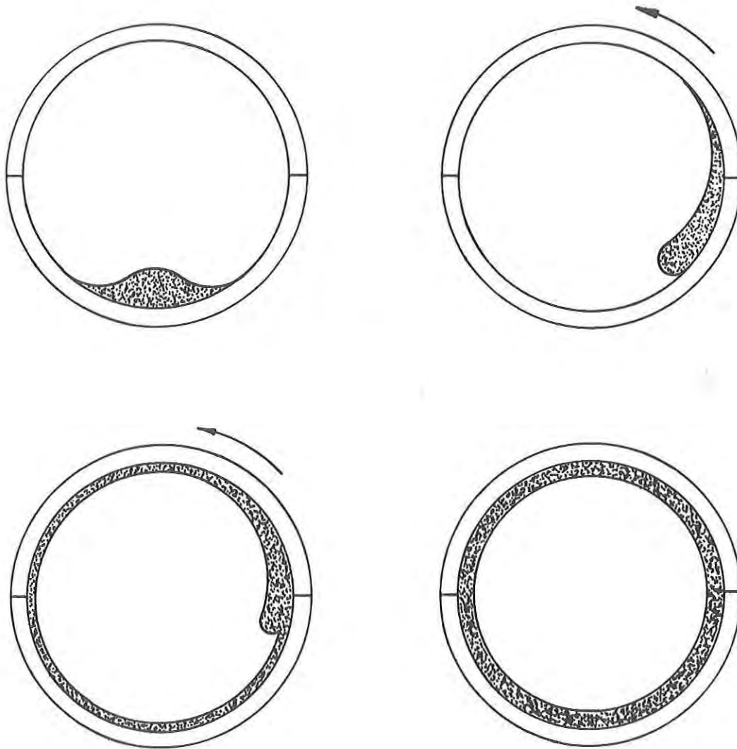
Figure 16. Rotation Molding Laminar Flow
