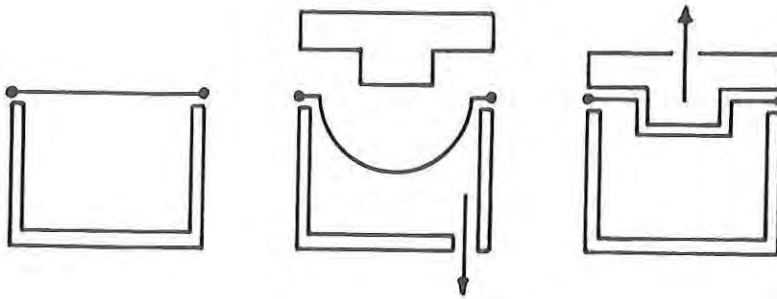
Figure 11. Vacuum Snap-Back Forming
