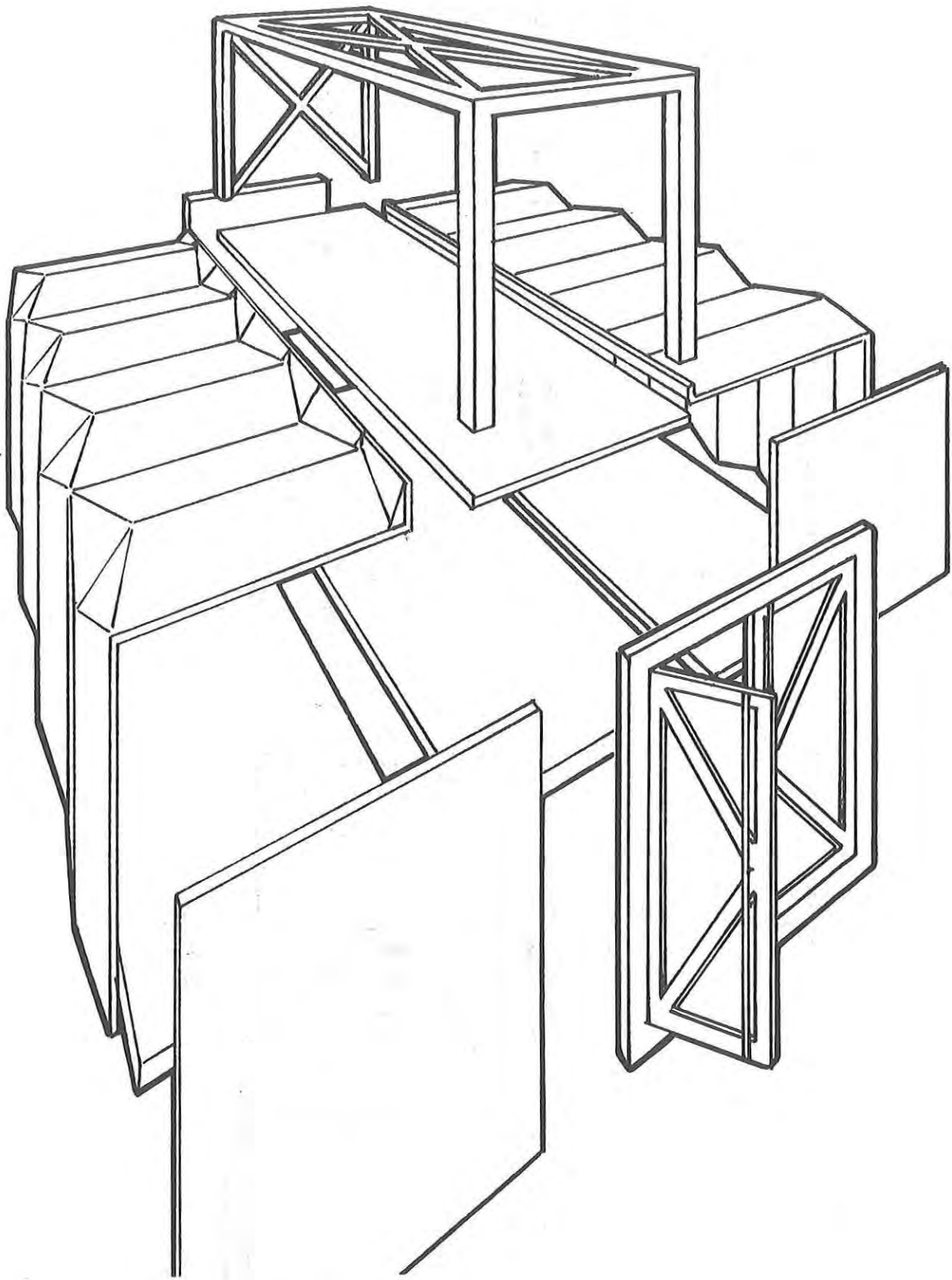
Figure 74. Configuration K
