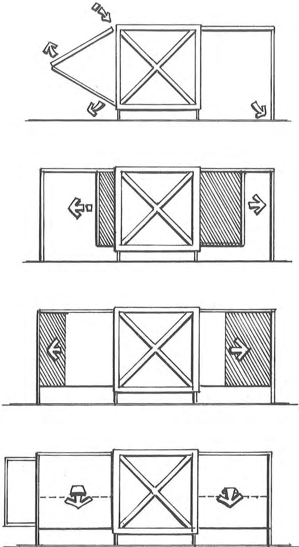
Figure 93. Expansion Procedure
