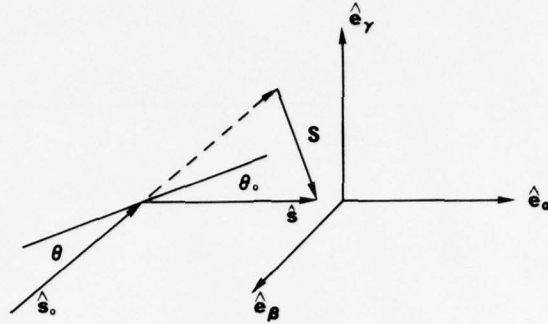
Fig. 1 — The relationship between the (\hat{e}_\gamma, \hat{e}_\beta, \hat{e}_\alpha) coordinate system and the incident and diffracted direction vectors. For appreciable intensity in the diffracted beam, \theta \approx \theta_0 . Note that \mathbf{S} = \sin(\theta + \theta_0)\hat{e}_\gamma + \cos(\theta + \theta_0)\hat{e}_\alpha .
