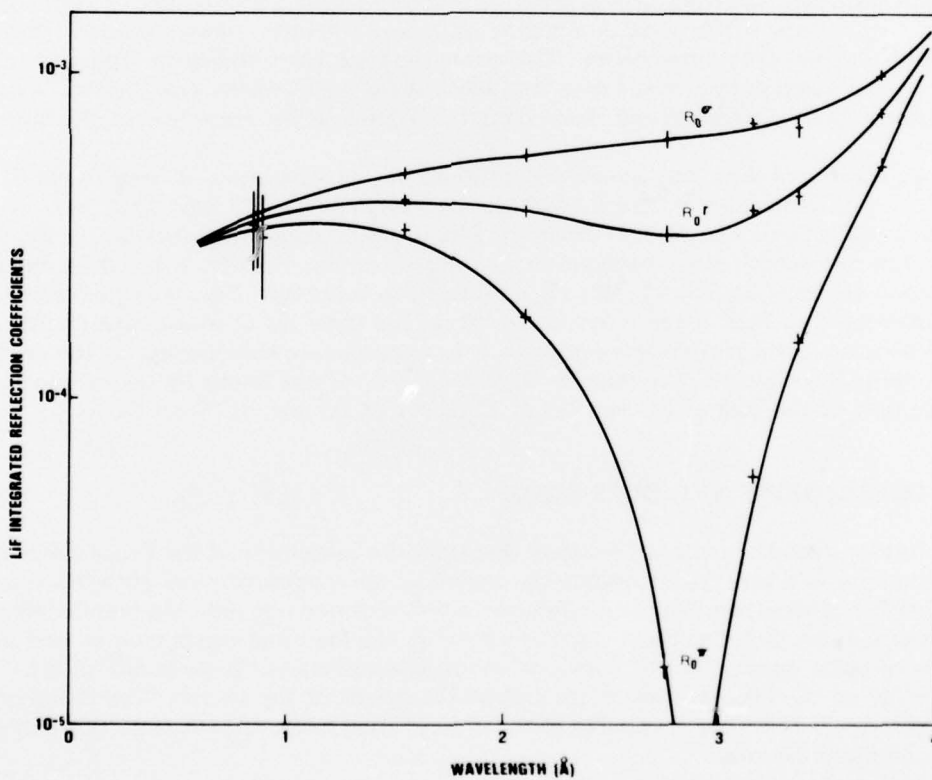
Fig. 9 — First-order integrated reflection coefficients for a lithium fluoride crystal (200 cut) as a function of diffracted wavelength. Two of the data points at 0.877 \text{\AA} are displaced in wavelength for clarity.
