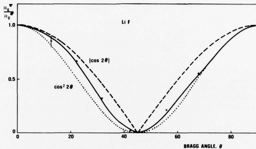
Fig. 8 — The ratio of the polarization factor, R_0^\pi/R_0^0 , for a lithium fluoride crystal (200 cut). Note that this ratio conforms to neither the perfect crystal diffraction theory ( |\cos 2\theta| ) nor the ideally imperfect crystal diffraction theory ( \cos^2 2\theta ).
