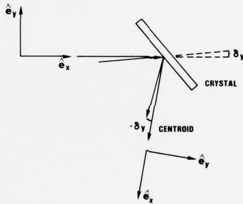
Fig. 7 — Incident and diffracted reference frames. The divergence angle becomes negative on reflection.
