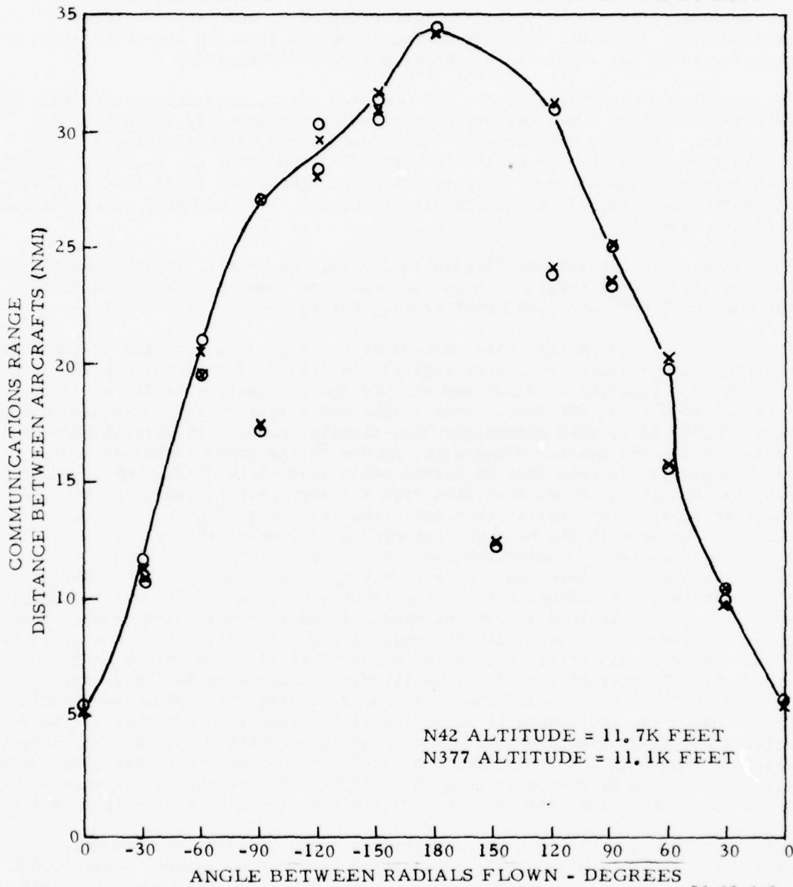
Figure 6-5. COMMUNICATIONS RANGE FLIGHTS, N377 (CAU) VS. N42 (CAU)
