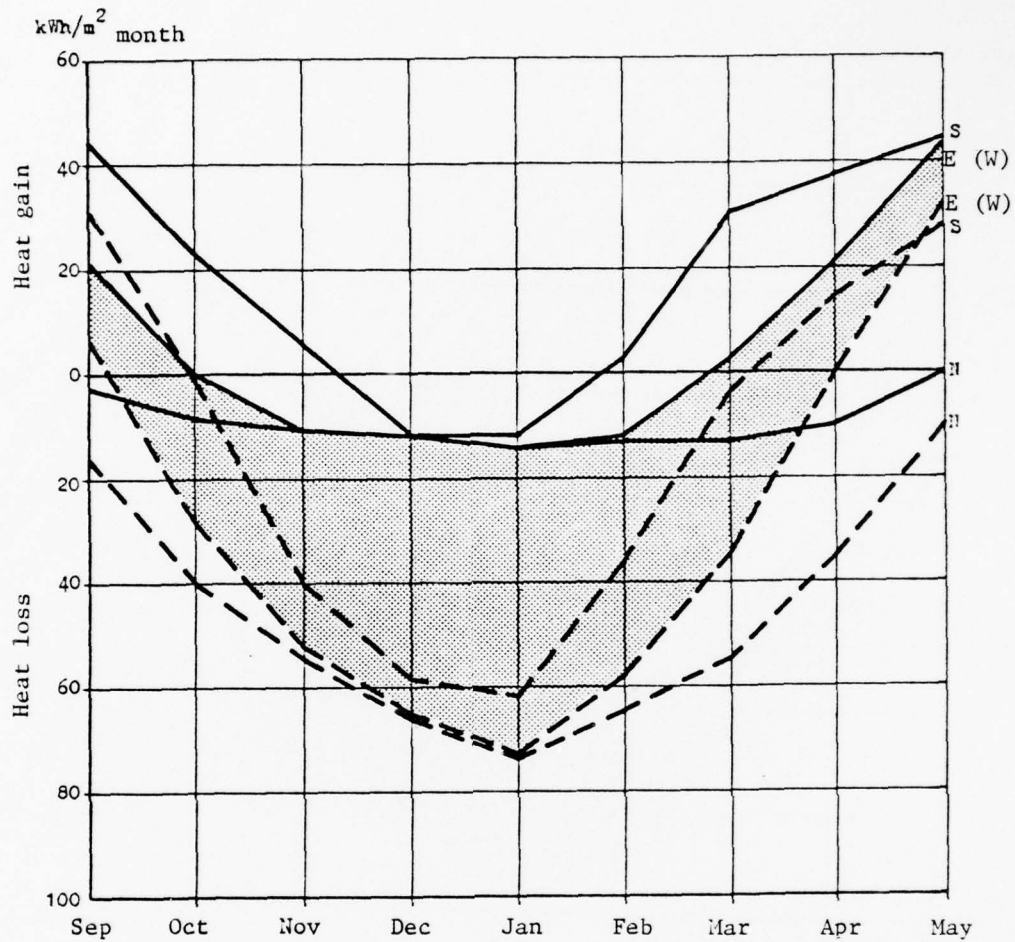
Figure 8. Energy balance for 2-pane windows, including transmission, air leakage and incoming radiation ( E_{t,l,s} ), from computer calculations. Solid curves: with shutters (optimum utilization = alt. 4) Broken curves: without shutters (alt. 2). The values apply to Stockholm (latitude 59°). Compass points N, S, E (W). Shaded area = energy gain with shutters, facing E (W).
