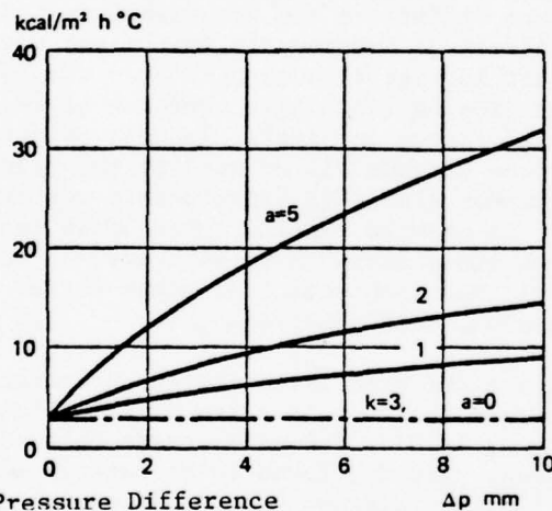
Fig. 2 Calculated heat transfer coefficient k_{t,1} (kcal/m 2 h°C) for windows with respect to transmission and air leakage as function of the pressure difference \Delta p (mm water column). Joint permeability a = 1, 2 and 5 Nm 3 /h.
