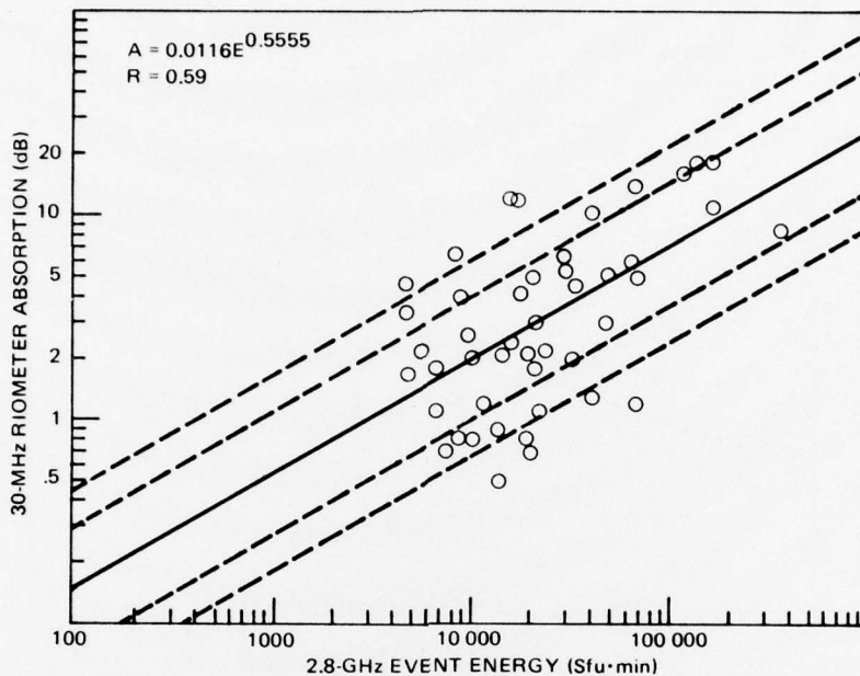
Figure 3. Riometer absorption versus event energy (table 2 events with E \geq 3000 Sfu · min).
