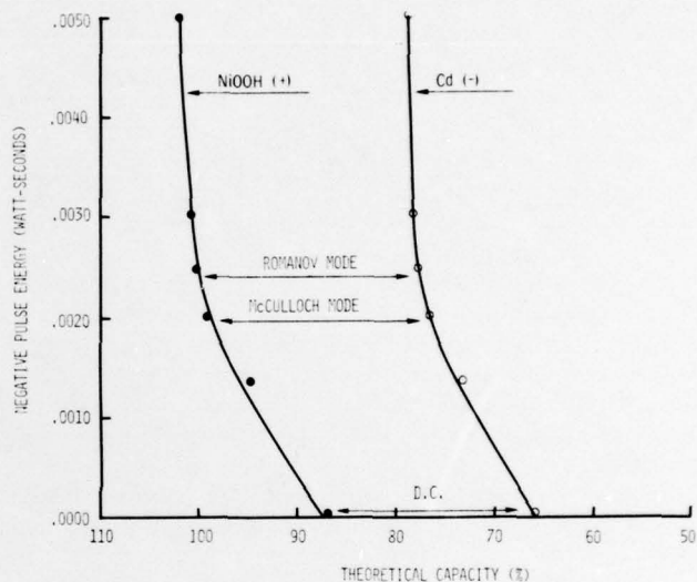
Figure 4. Capacity of the NiOOH and Cd Electrodes as a Function of Negative Pulse Energy.
