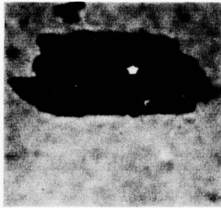
Bi-Cubic Spline Approximation by Subpartitioning
