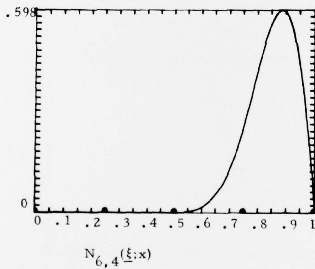
Figure A.1 (continued) Normalized 4th Order B-Splines For Knot Vector \xi = (0, 0, 0, 0, .25, .5, .75, 1, 1, 1, 1)
