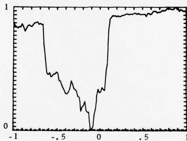
40 Knots Placed Uniformly
