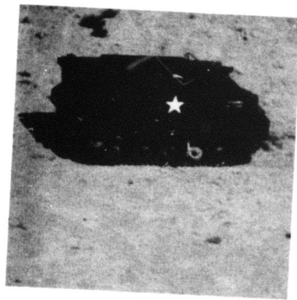
Figure 6.8 Original 256 by 256 APC Image.
