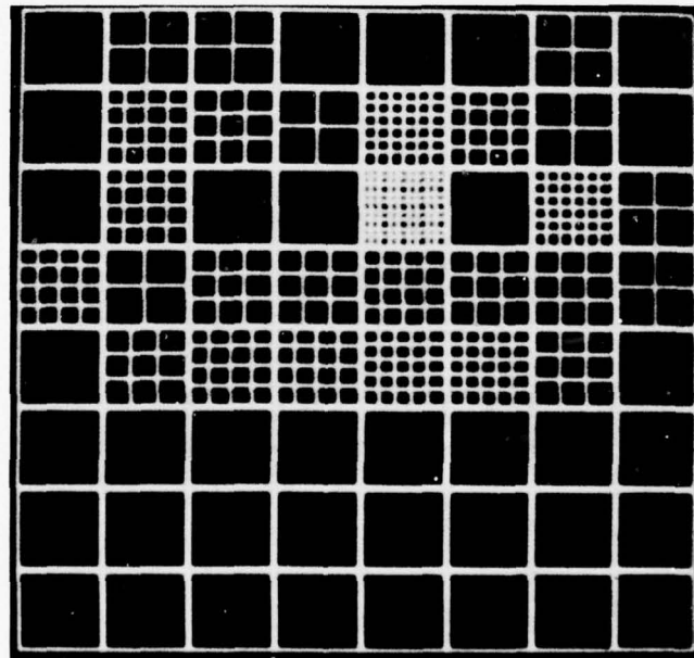
Associated Knot Density
