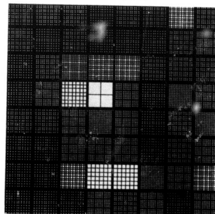
Figure 6.13. Bicubic Spline Reconstructions and Associated Knot Densities for LAX Photograph Using Subregions of Size 32 \times 32 .
