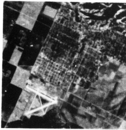
Figure 6.12 Original 256 by 256 Reconnaissance Image.
