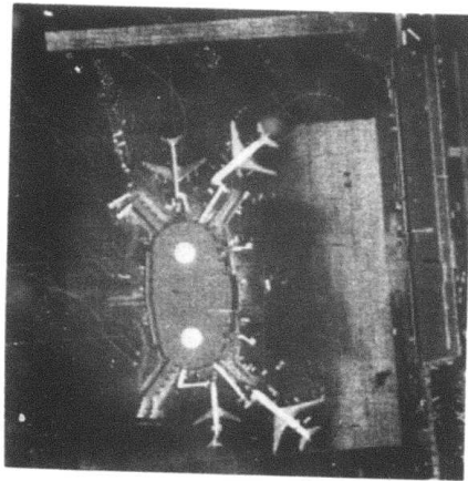
Figure 6.16. Original 256 x 256 LAX Image.
