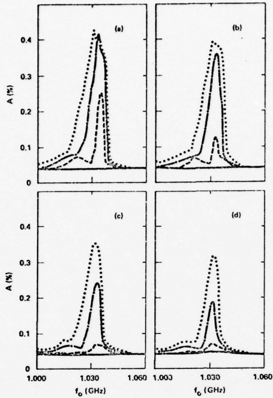
Fig. 8 Saturated density fluctuation level A as a function of pump power and center frequency for the noise phase-modulated pump. The noise bandwidth \Delta\omega/2\pi is < 10 kHz for (a), 3 MHz for (b), 6 MHz for (c), and 12 MHz for (d). Pump power is varied from 0.5 to 2.0 W: —, 0.5 W; ---, 1.0 W; -.-, 1.5 W; and ... , 2.0 W.
