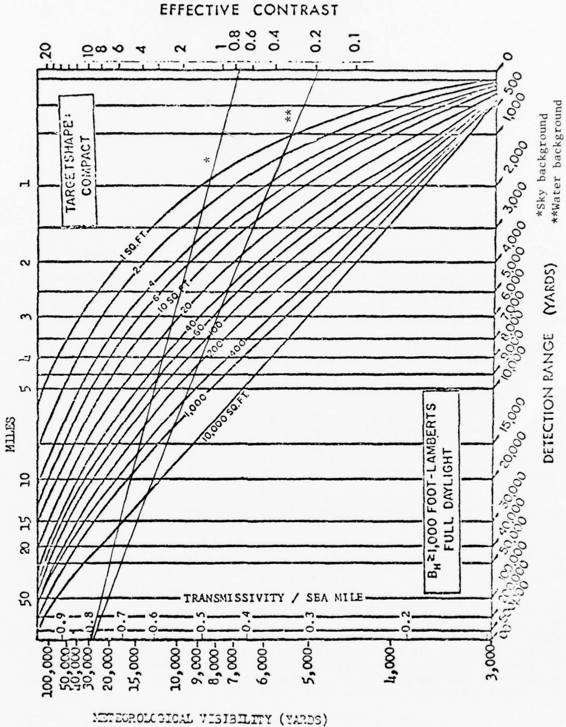
FIGURE 17 DUNTLEY'S NOMOGRAM
