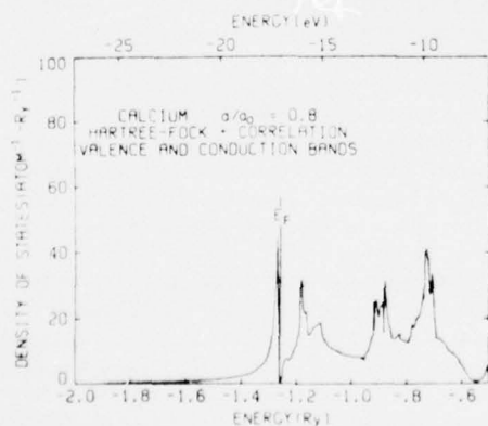
Fig. 7. Density of states of valence and conduction bands derived from the Hartree-Fock results corrected for electron correlation.
