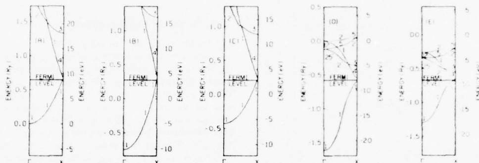
FIG. 3. The relationship between free-electron bands and Hartree-Fock bands ( a/a_0 = 1.0 ) with and without correlation corrections. Panel (A): free-exchange bands for an electron gas with the density of calcium and m^* = 0.533m . Panel (B): free electron bands with exchange energy E_x . Panel (C): free-electron bands with exchange-correlation energy E_x + E_c . Panel (D): Hartree-Fock bands. Panel (E): Hartree-Fock bands with correlation energy E_c .
