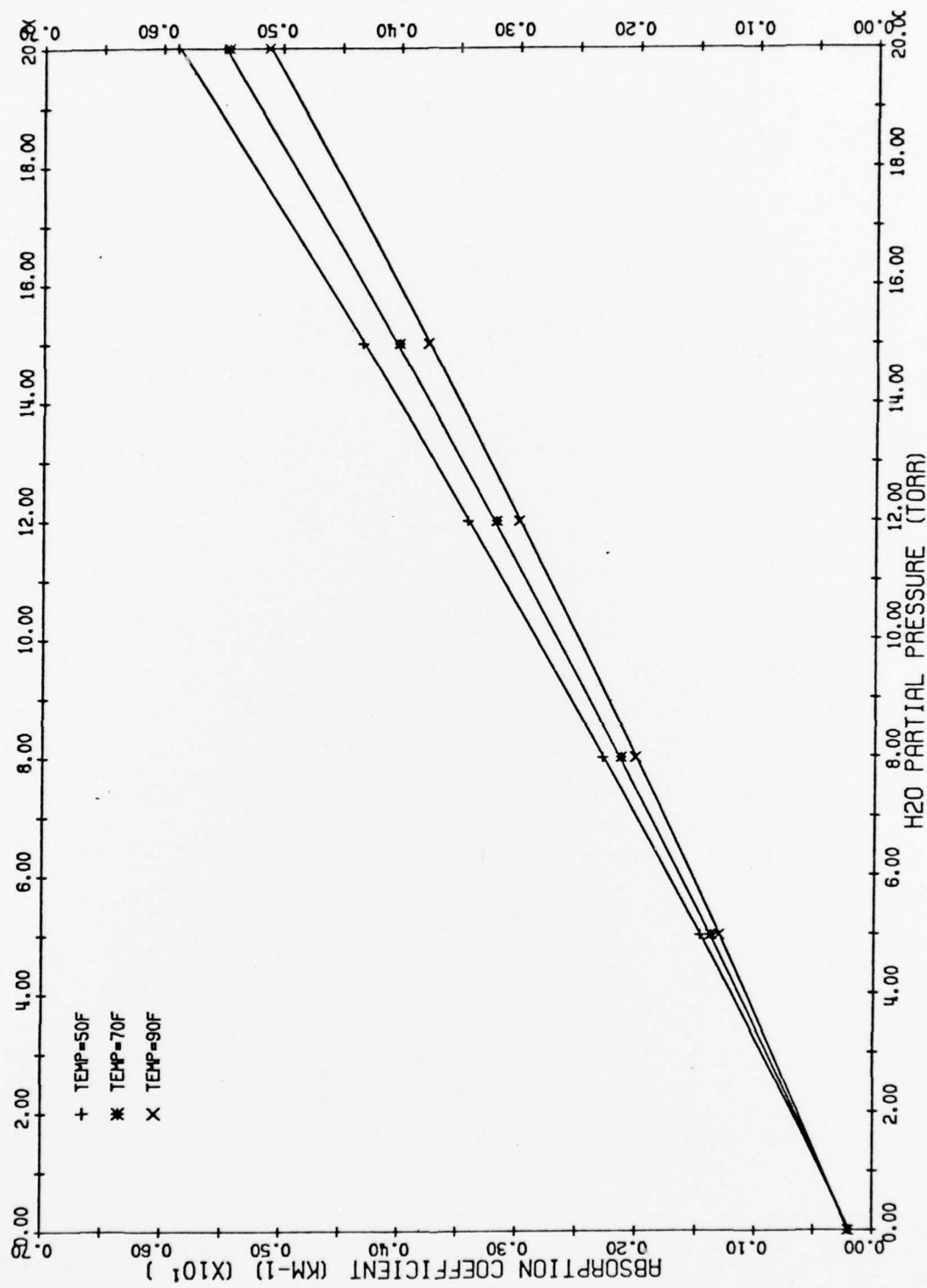
Figure 16. ABSORPTION COEFFICIENTS FOR THE P1(10) DF LINE AT 2665.218 WAVENUMBERS
