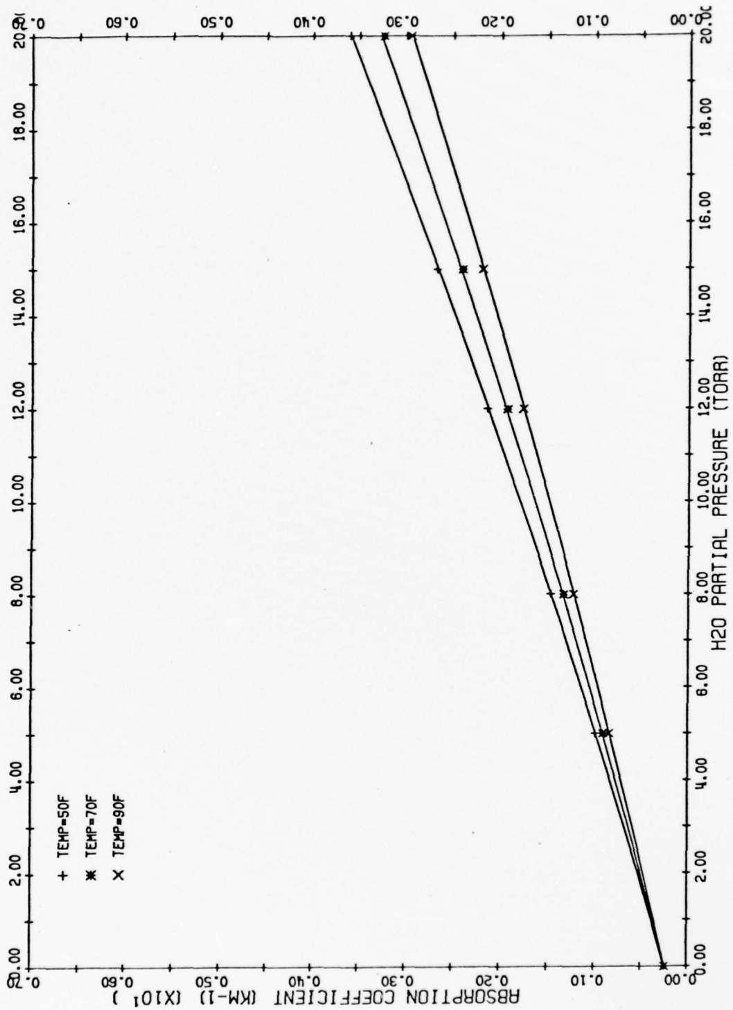
Figure 13. ABSORPTION COEFFICIENTS FOR THE P3(5) OF LINE AT 2617.389 WAVENUMBERS
