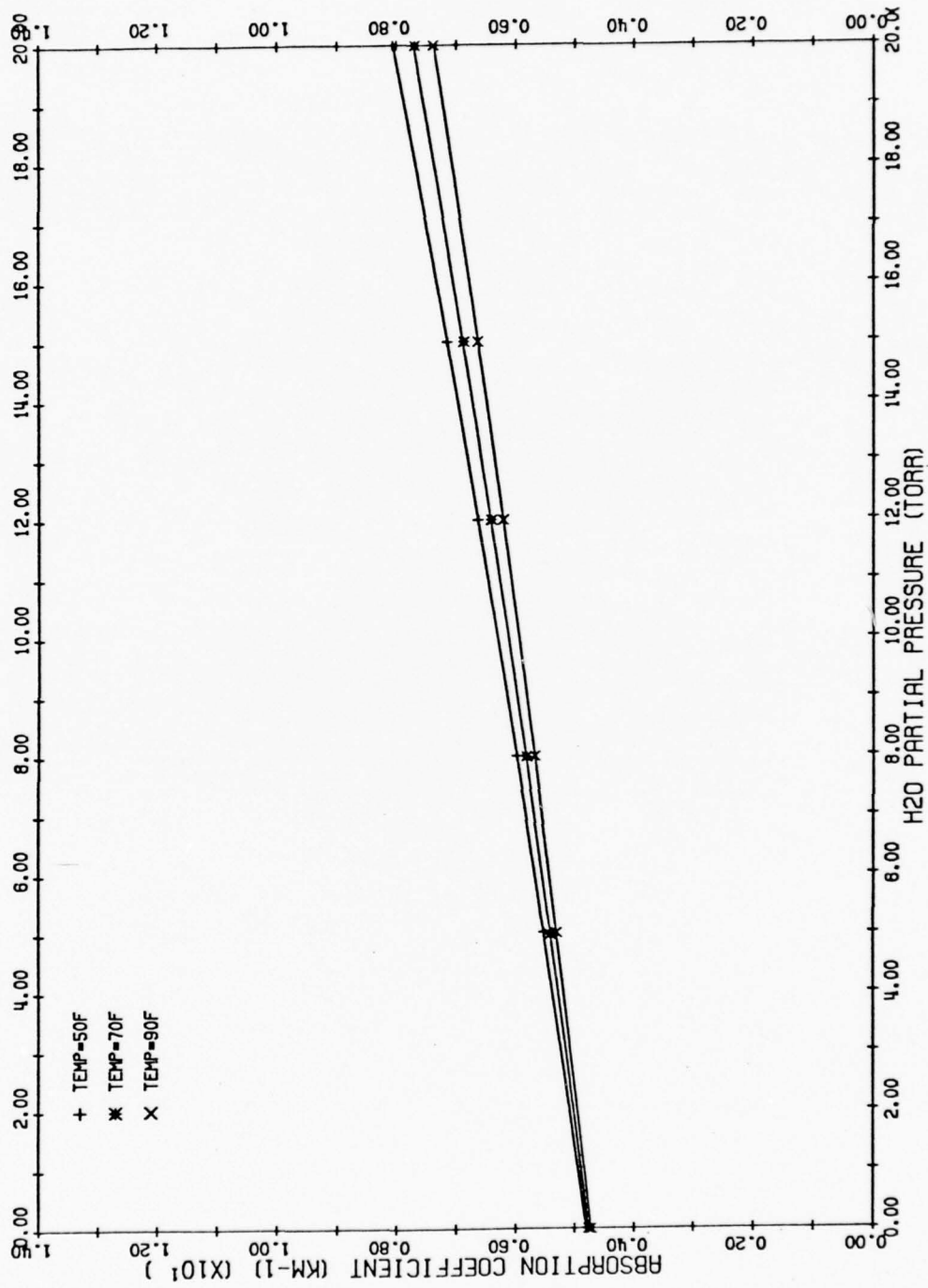
Figure 10. ABSORPTION COEFFICIENTS FOR THE P2(10) OF LINE AT 2580.102 WAVENUMBERS
