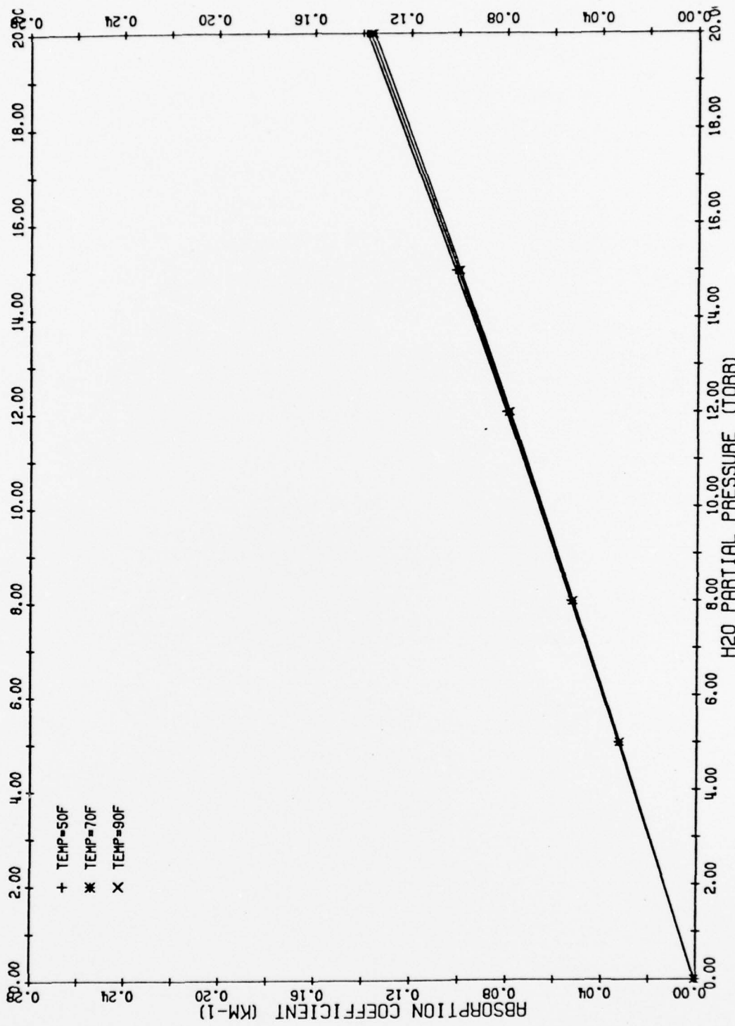
Figure 15. ABSORPTION COEFFICIENTS FOR THE P2(7) OF LINE AT 2655.861 WAVENUMBERS
