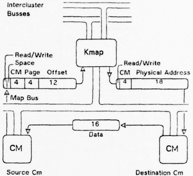
Figure 2.2 The Mechanism for Cluster-local References
