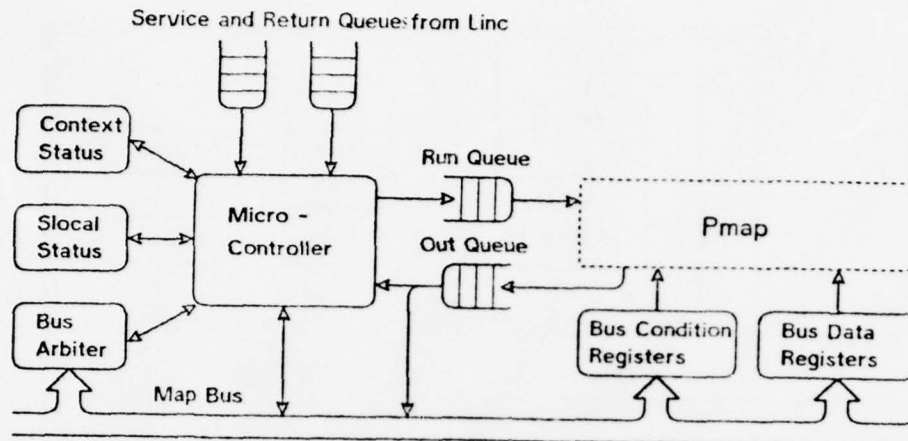
Figure 5.1 The Components of the Kbus
