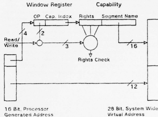
Figure 3.4 Conceptual Virtual Address Generation and Rights Checking
