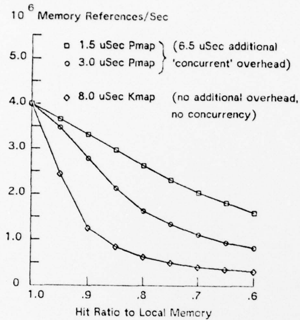
Figure 9.2 Cluster Performance with Slower Pmap or without Concurrency between Pmap and Map Bus
