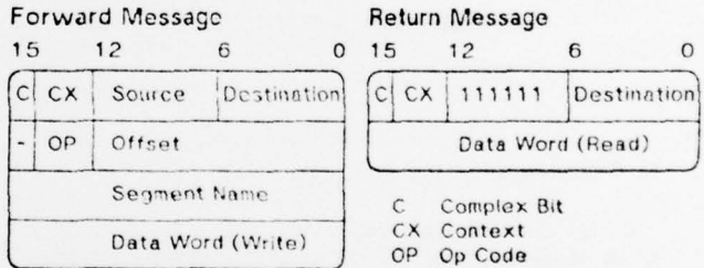
Figure 7.1 Standard Message Formats
