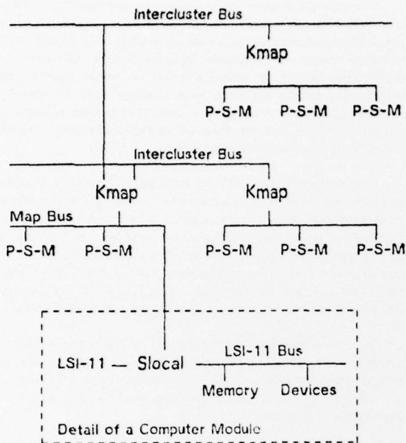
Figure 1. A Simple 3 Cluster Cm* System
