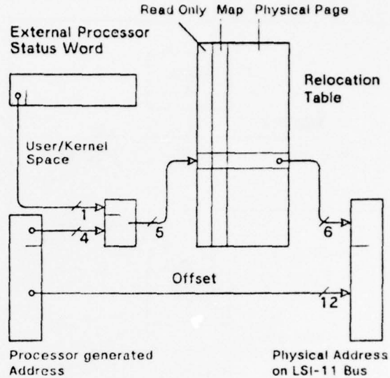
Figure 3.1 Addressing Mechanism for Local Memory References
