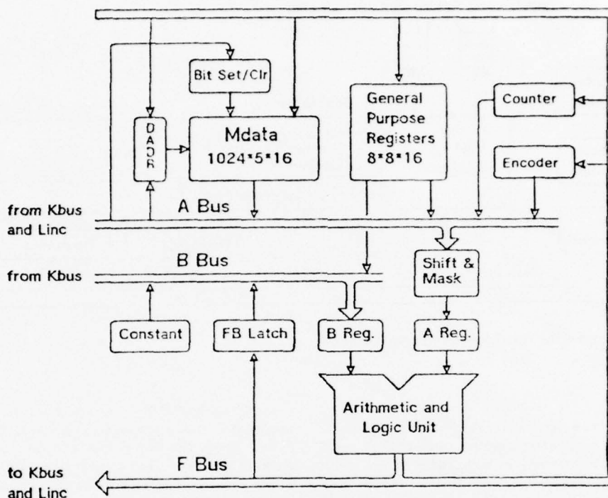
Figure 6.1 Data Paths in the Pmap
