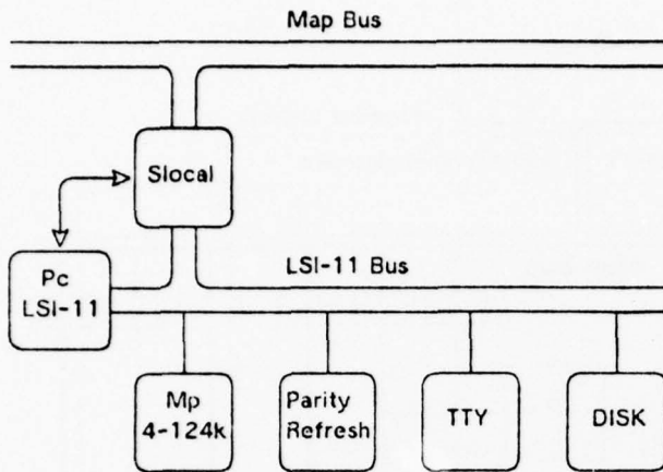
Figure 3.1 Details of a Computer Module
