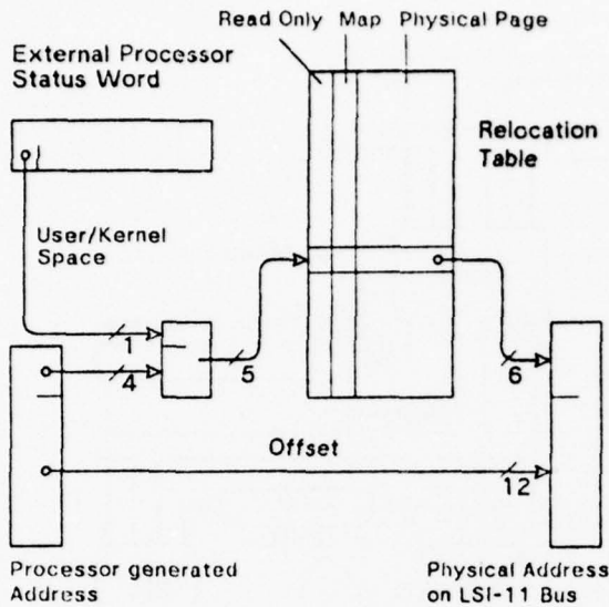
Figure 2.1 Addressing Mechanism for Local Memory References
