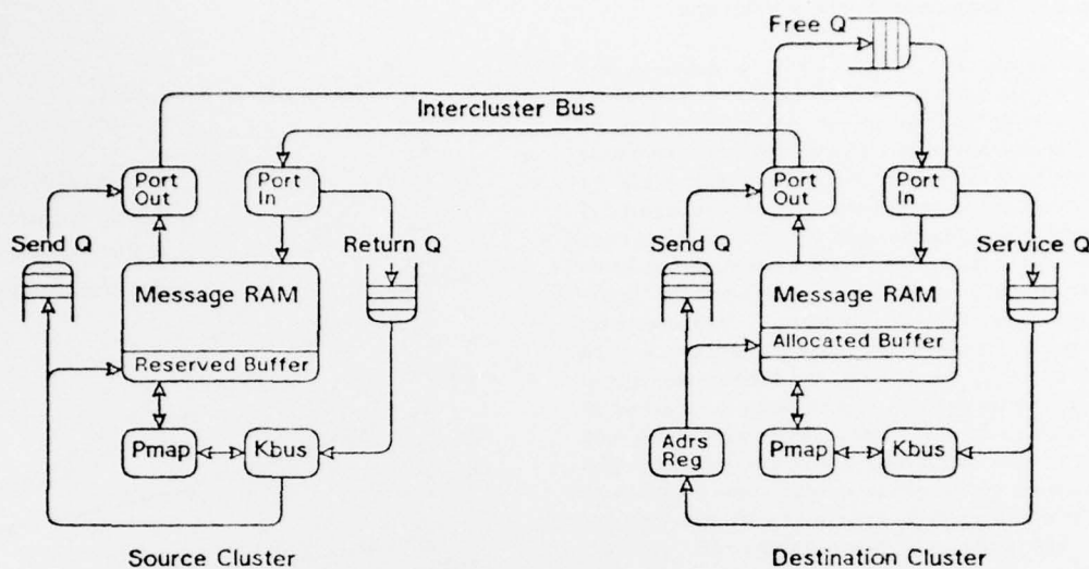
Figure 7.3 An Intercluster Message Transaction
