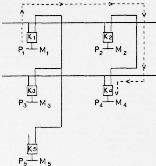
Figure 2.1 Canonical Computer Module Structure
