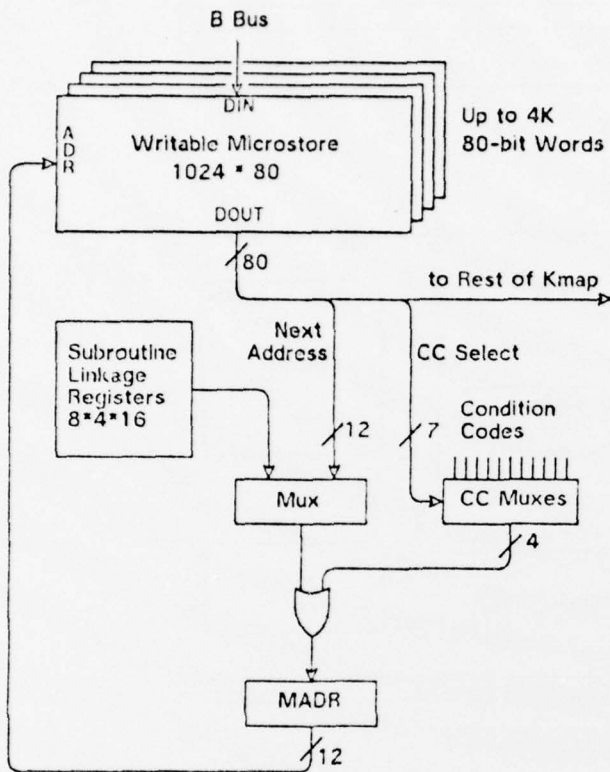
Figure 6.2 Microinstruction Address Generation Logic
