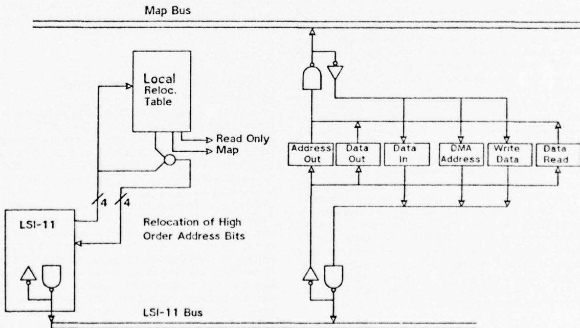
Figure 3.3 Simplified LSI-11 - Slocal Data Paths
