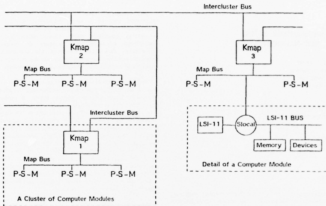
Figure 1.1 A Simple 3 Cluster Cm * System
