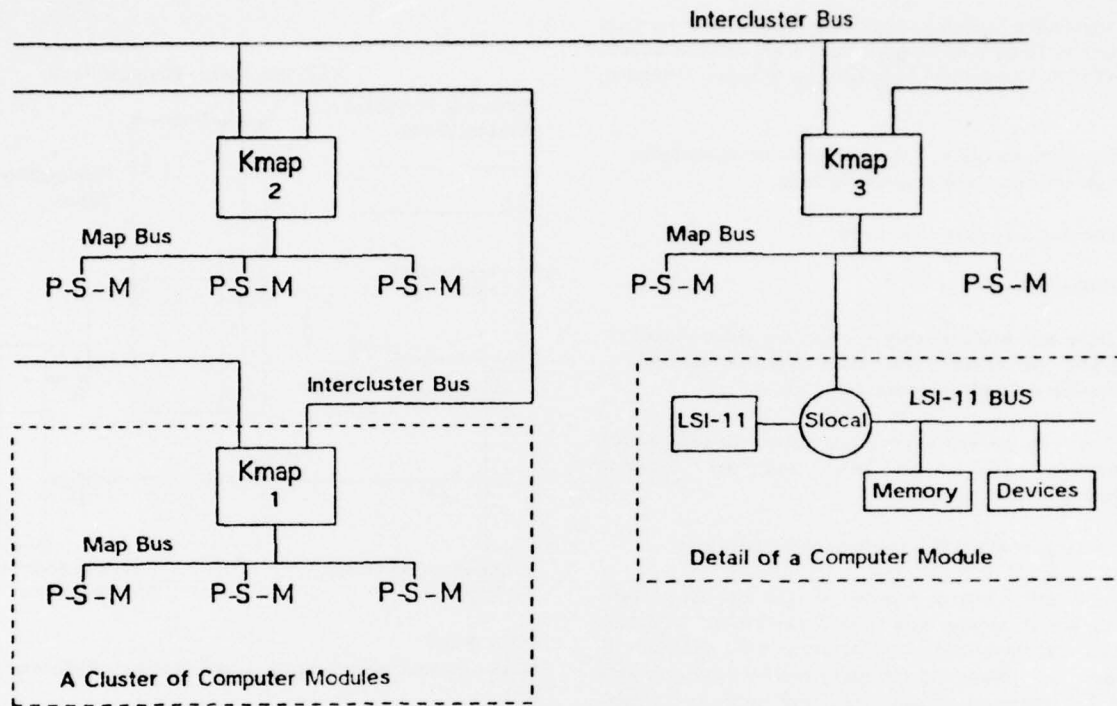
Figure 2.2 A Simple 3 Cluster Cm* System
