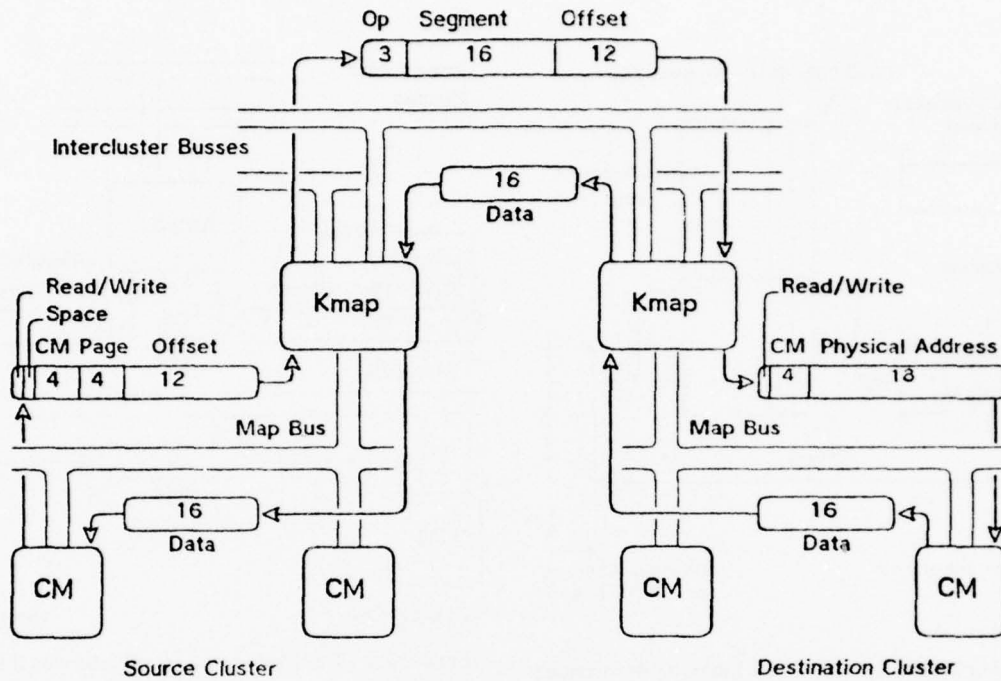
Figure 2.3 The Mechanism for Intercluster References
