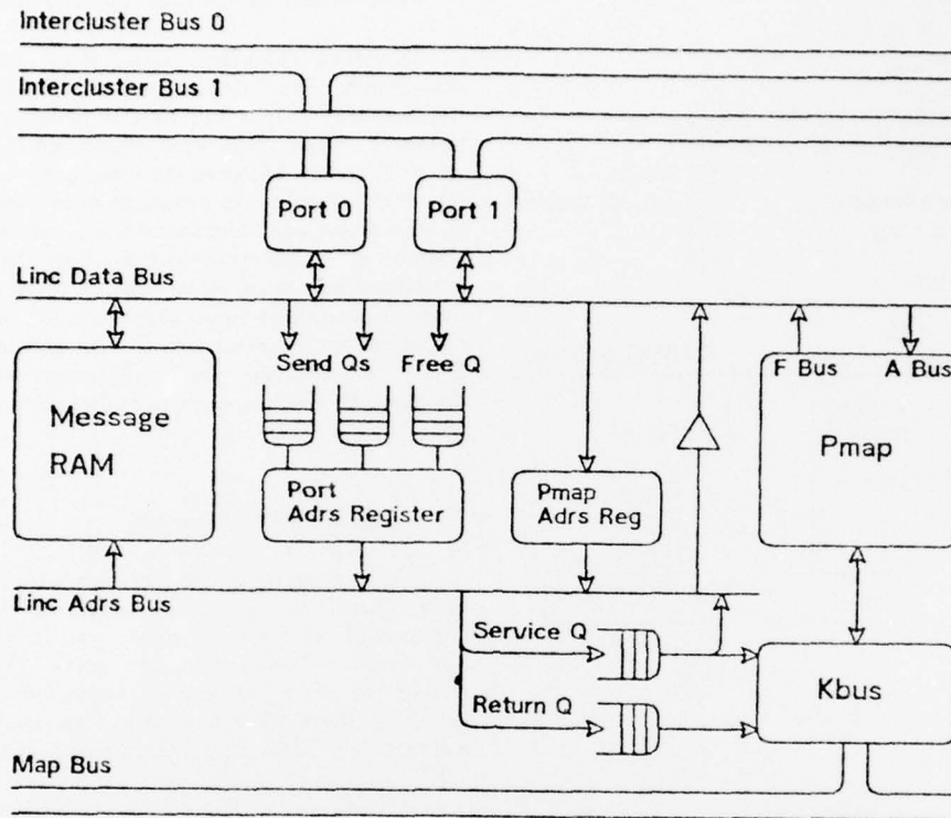
Figure 7.2 Components of the Linc
