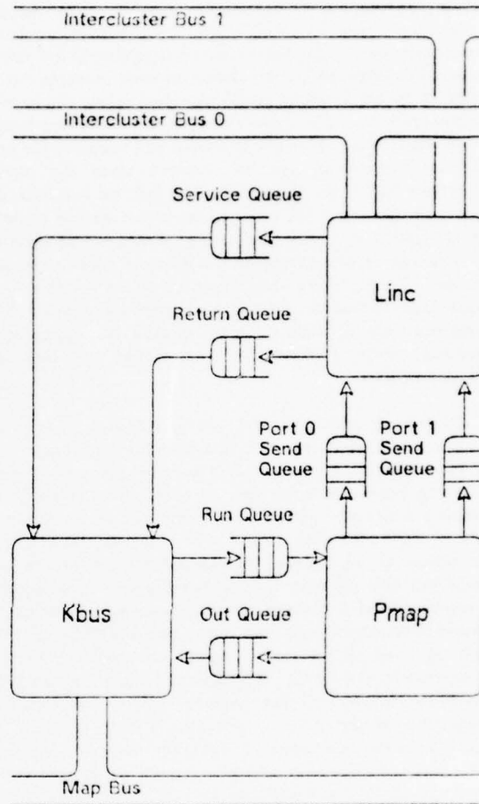
Figure 4.1 The Components of the Kmap
