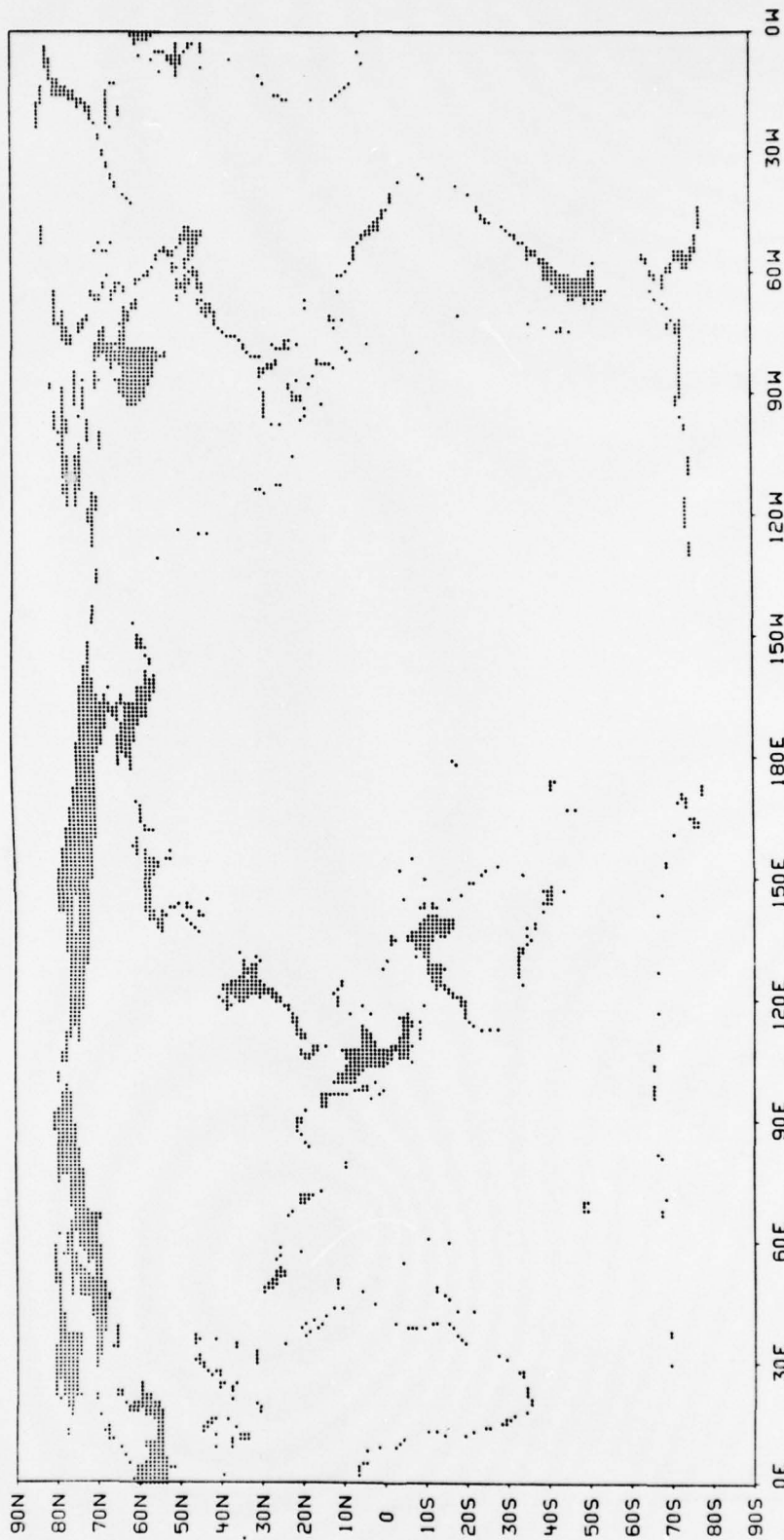
Fig. 4b LOCATIONS EXPOSED BY WATER LEVEL CHANGE
