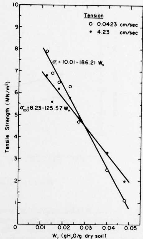
Figure 18. Correlation of uniaxial tensile strength and unfrozen water content.
