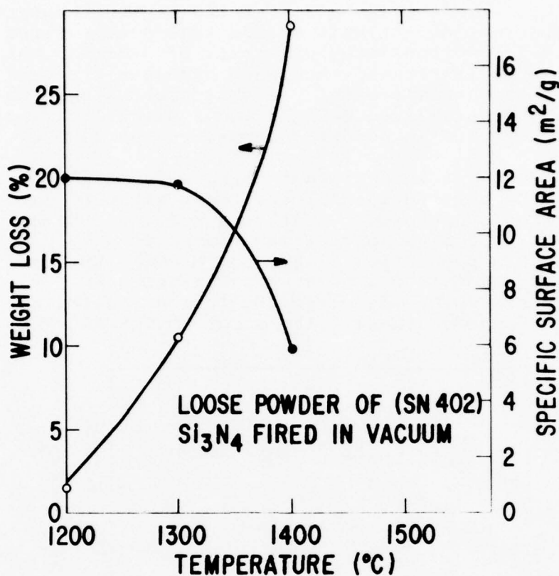
Figure 2. Weight Loss and Specific Surface Area as Function of Temp. for Loose Powder of SN-402 Si 3 N 4 Fired in Vacuum for 1 Hr
