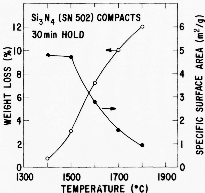
Figure 20. Weight Loss and Specific Surface Area as Function of Temp. for (SN-502) \text{Si}_3\text{N}_4 Compacts Fired for 30 Min in \text{N}_2
