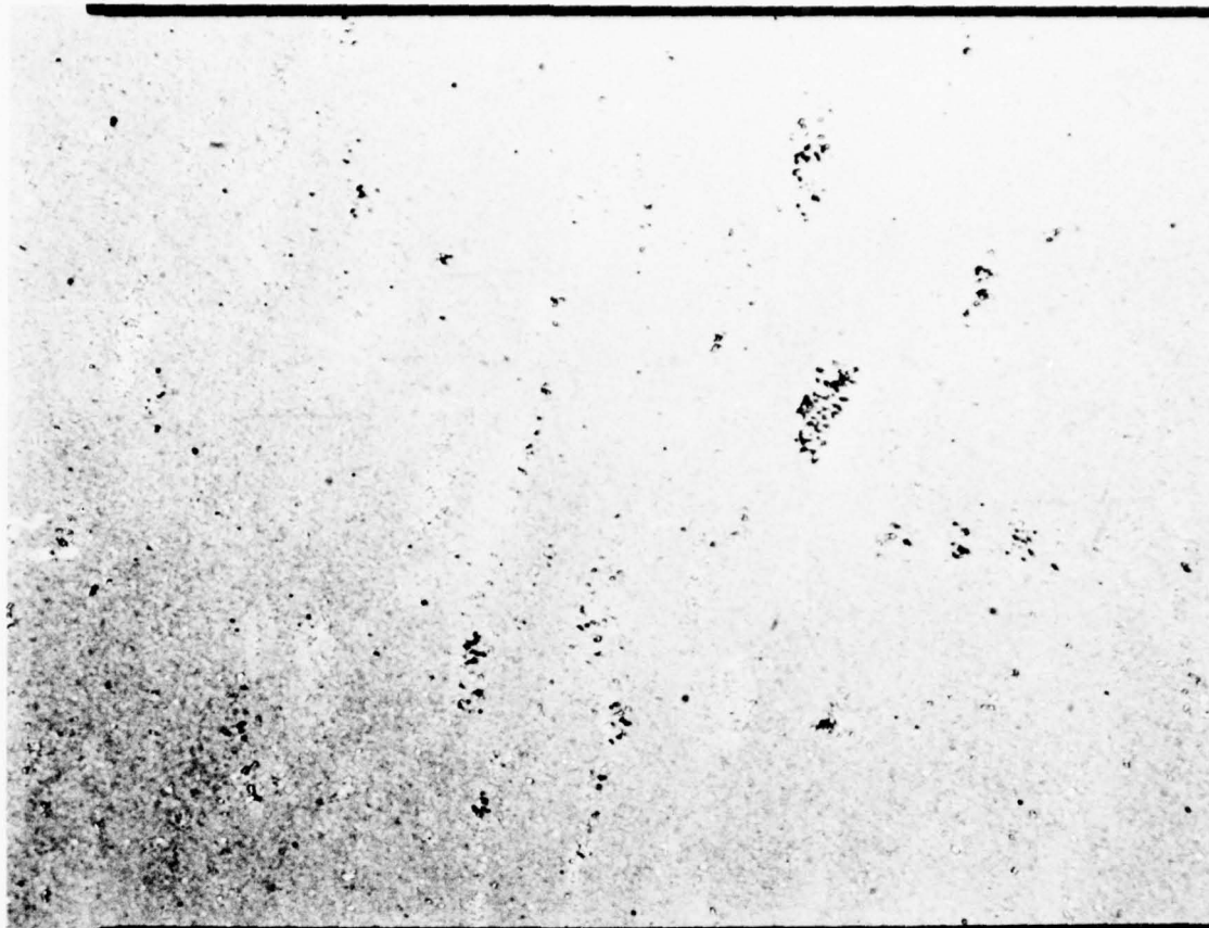
Figure 27. Microstructure of Hot-Pressed Si 3 N 4 Doped with 3 wt% Mg 2 Si Mag = 500 X
