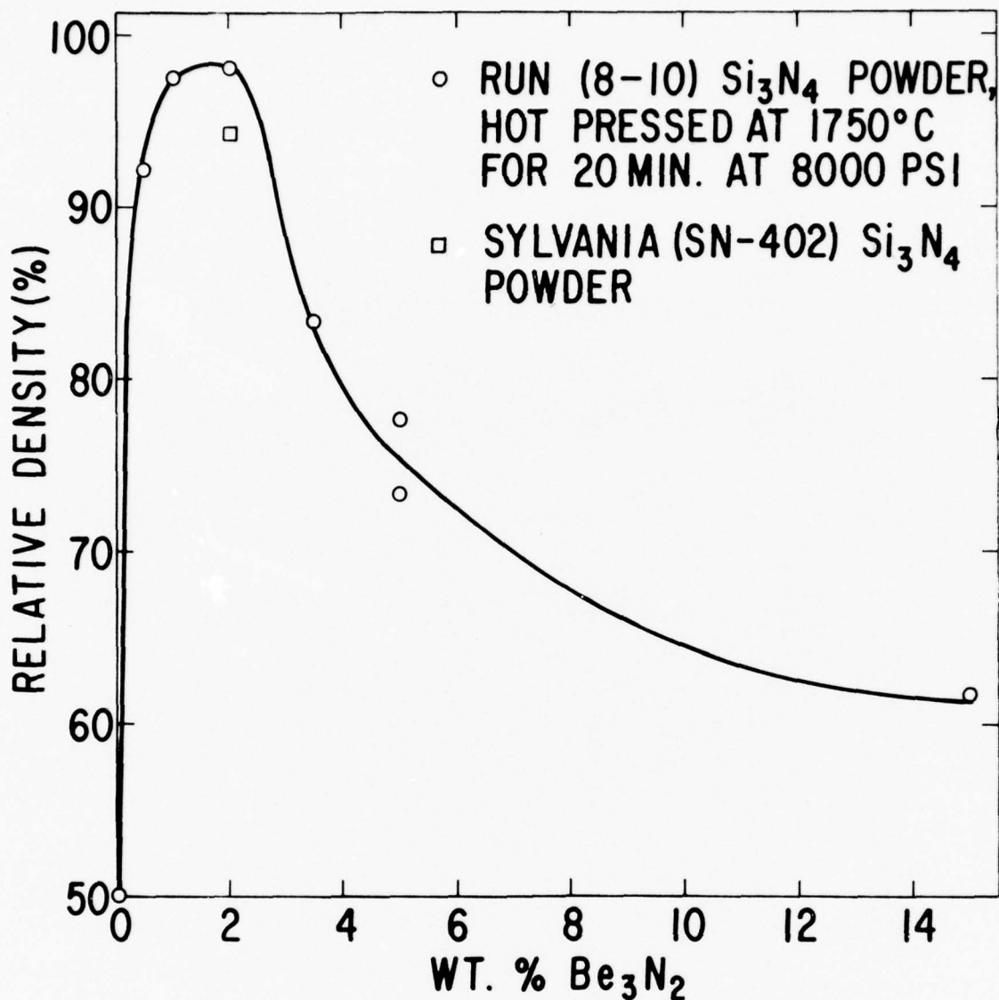
Figure 24. Relative Density of Hot-Pressed Si 3 N 4 as Function of Be 3 N 2 Content
