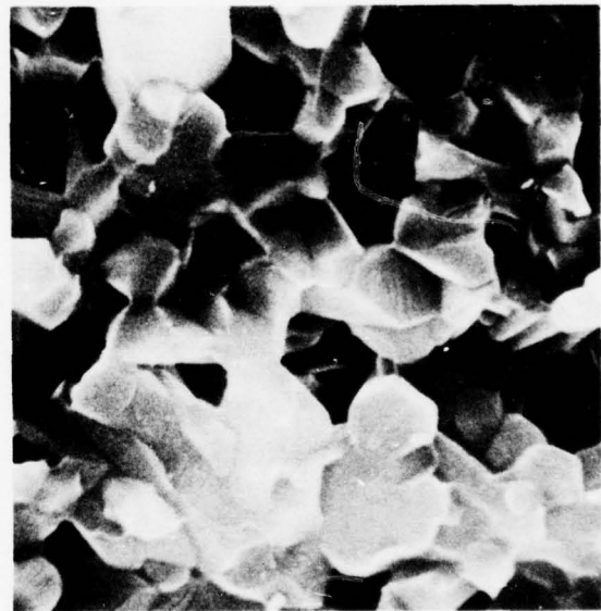
Figure 32(B). First \text{Si}_3\text{N}_4 Specimen Sintered to Appreciable Density (Exp. No. 6, Table 8) SEM of Fracture Surface 10,000 X
