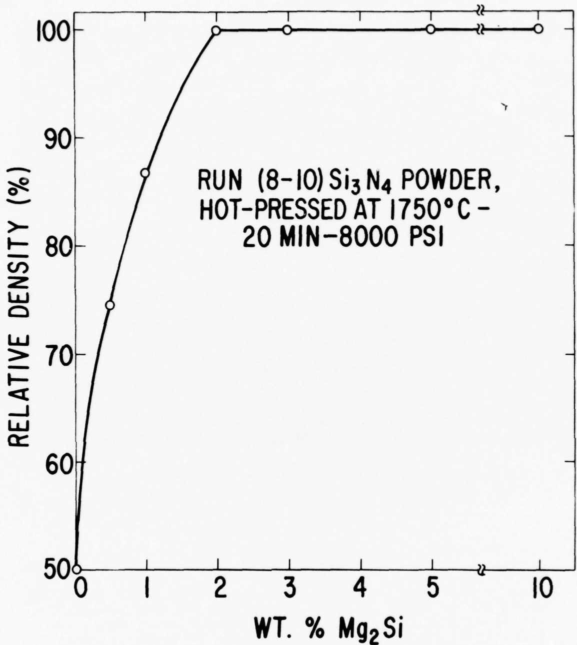
Figure 26. Relative Density of Hot-Pressed Si 3 N 4 as Function of Mg 2 Si Content
