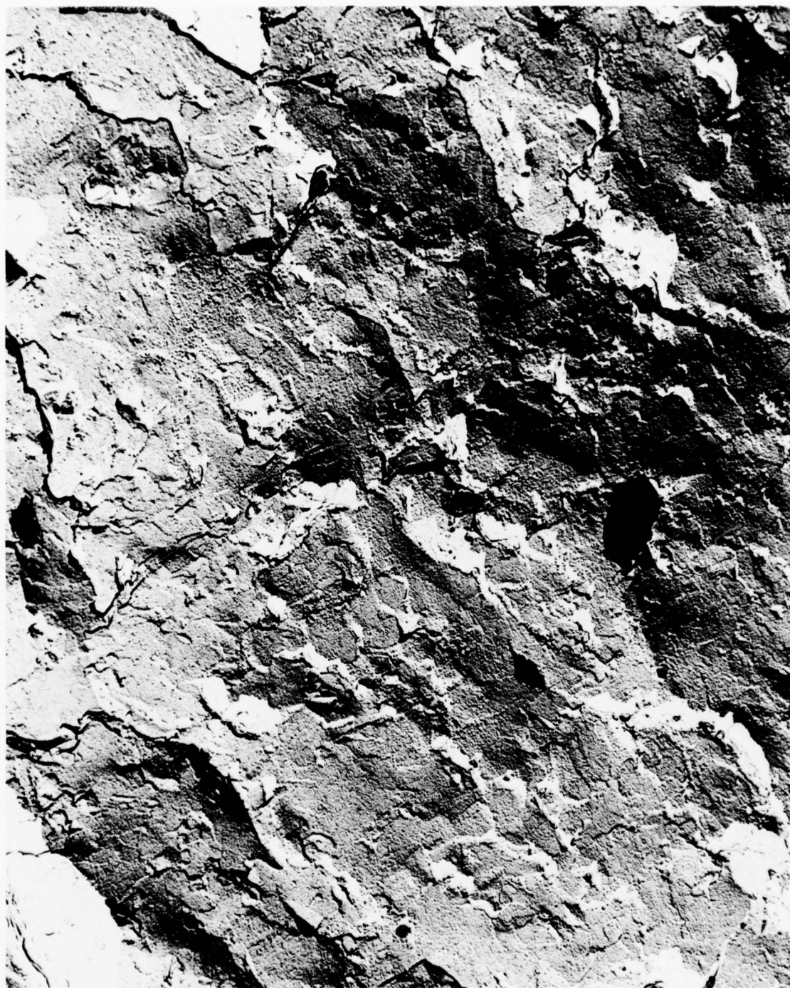
Figure 11. TEM of Replica of Fracture Surface of \text{Si}_3\text{N}_4 Compacted at 5 GPa at 1500^\circ\text{C} . Specimen No. 2 in Table 4. 30,000 X
