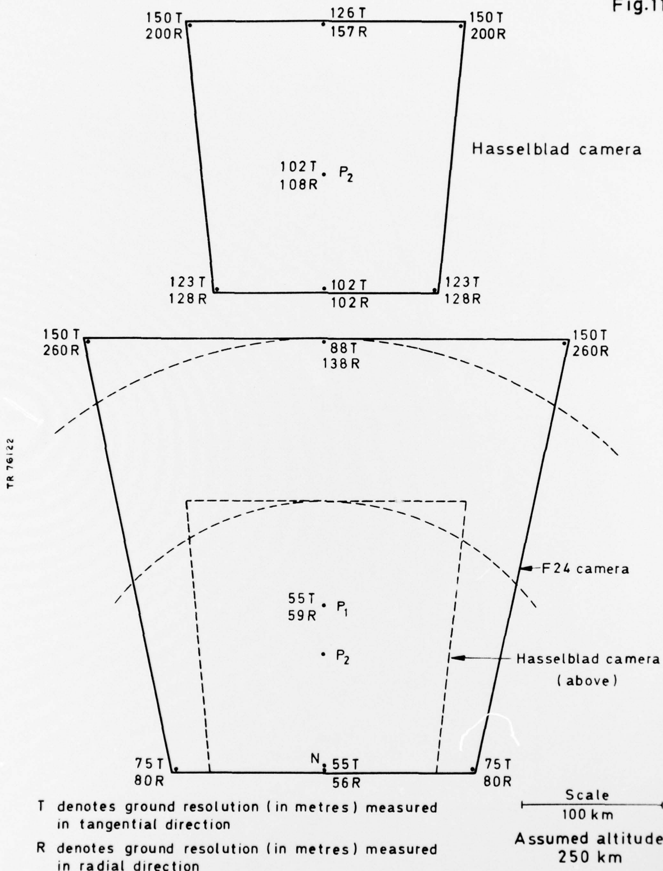
Fig.11 Calculated ground resolution of F24 and Hasselblad cameras: SL1081
