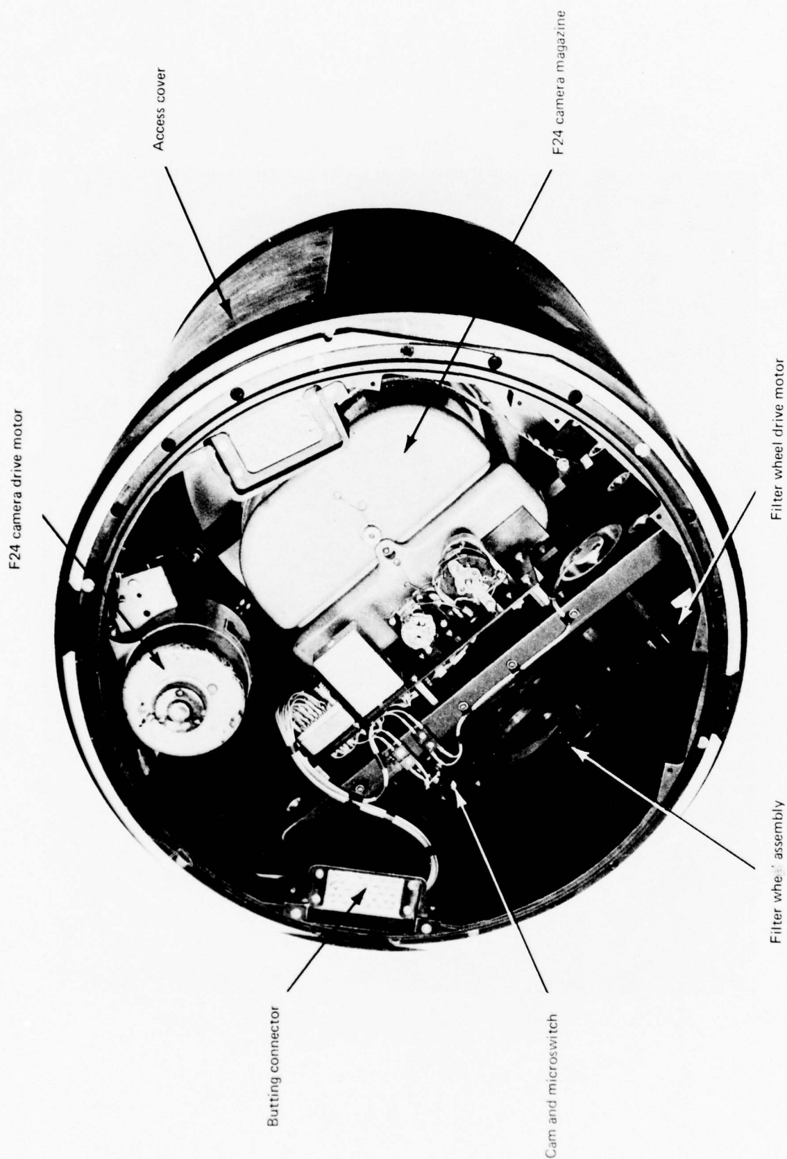
Fig.7 F24 camera system bay
