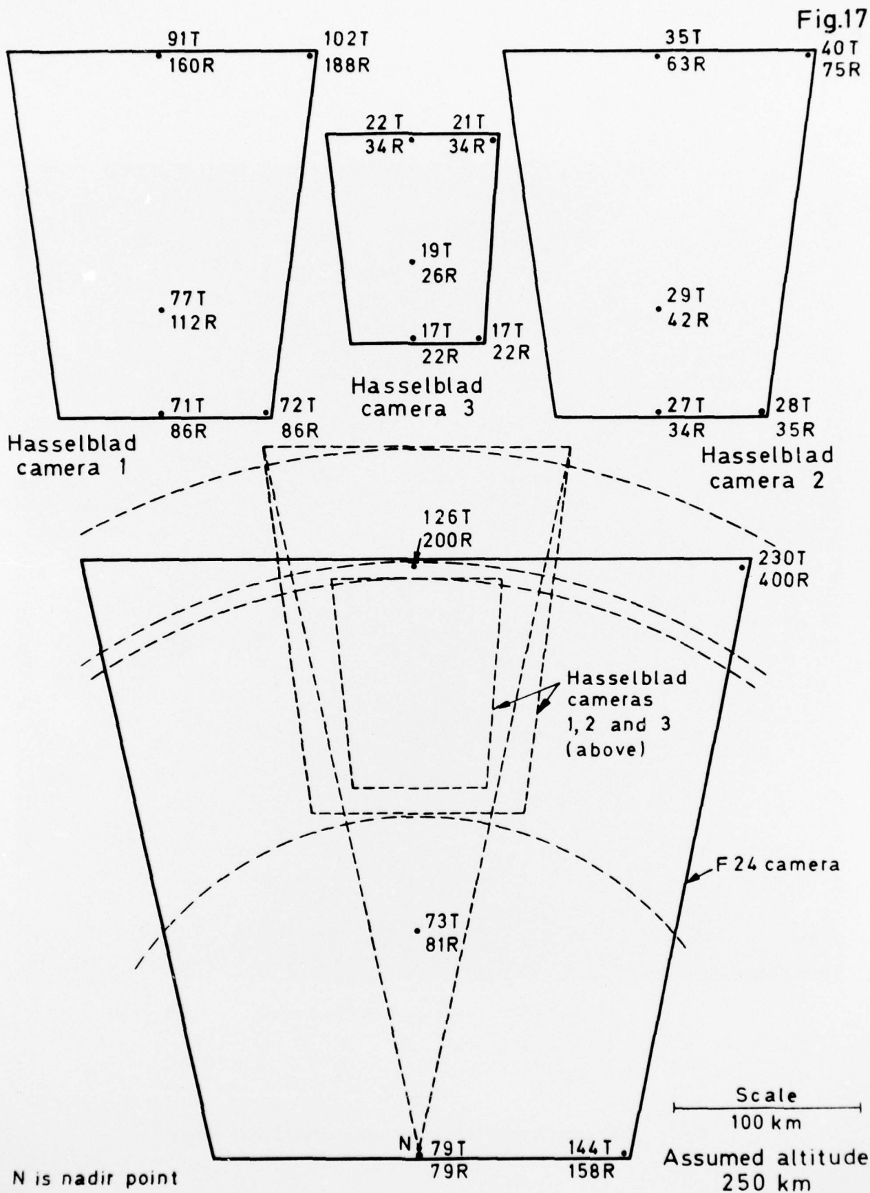
Fig.17 Calculated ground resolution of F24 and Hasselblad cameras: SL1181 and SL1182
