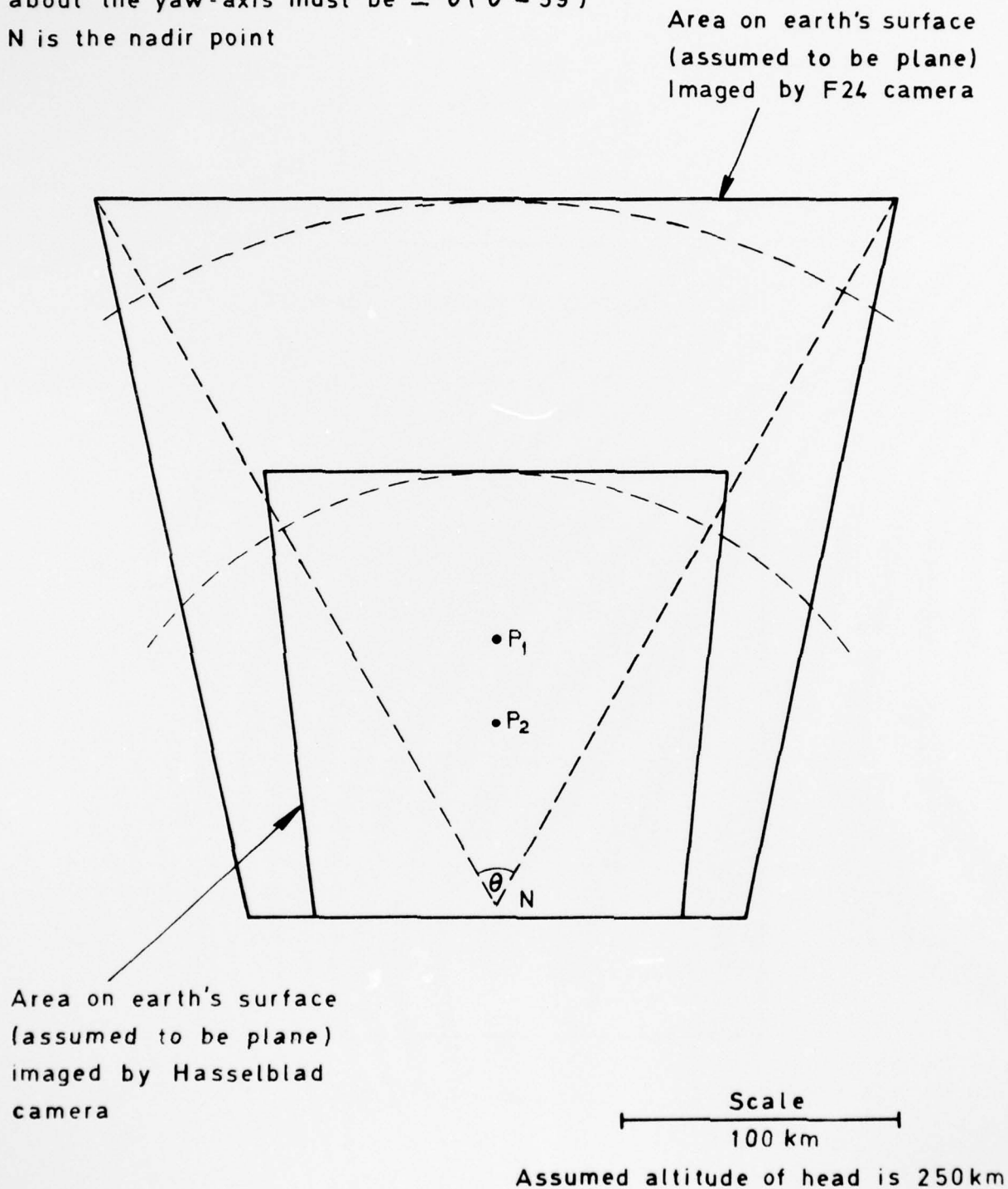
Fig.10 Calculated ground coverage of F24 and Hasselblad cameras: SL1081
