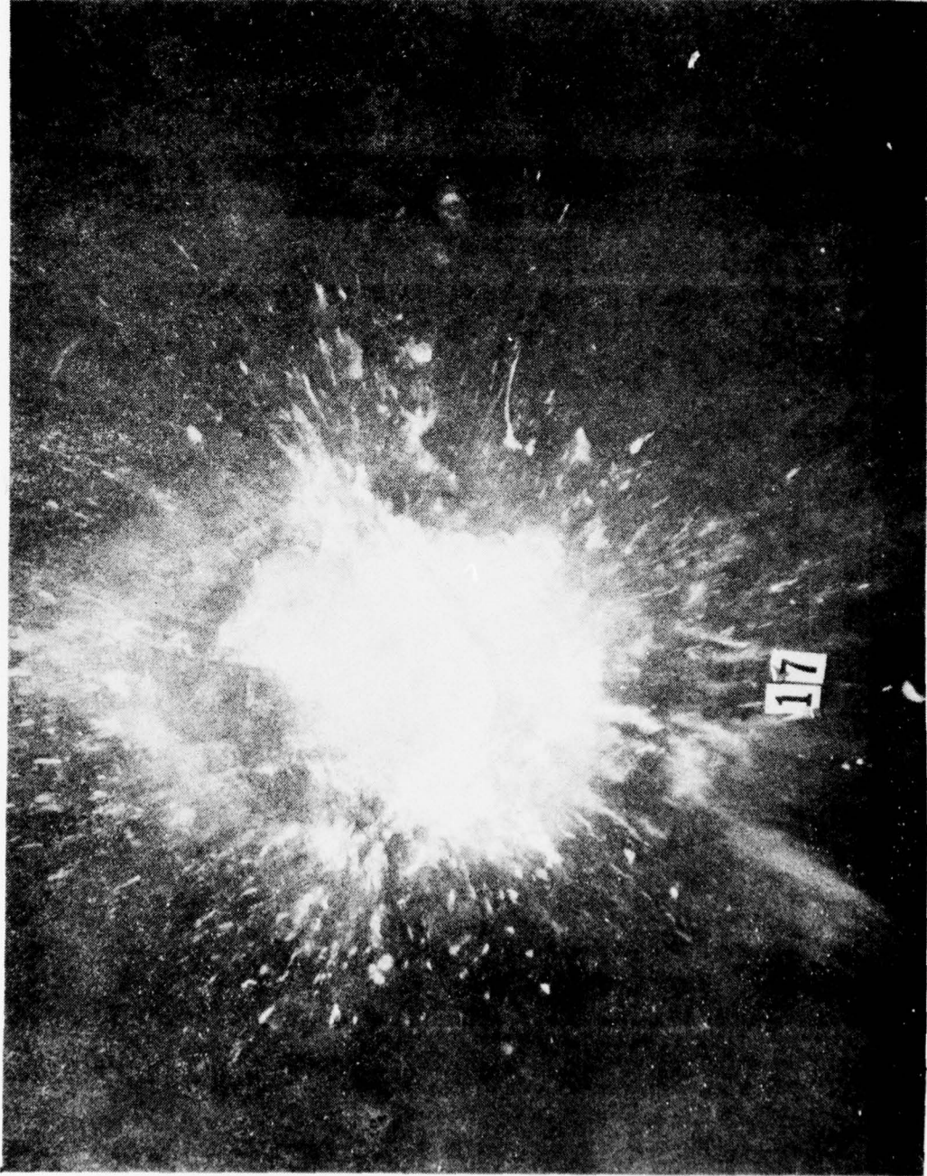
Figure 20. Test No. 17, Colorado Sandstone Versus Fiber Glass — Closeup
