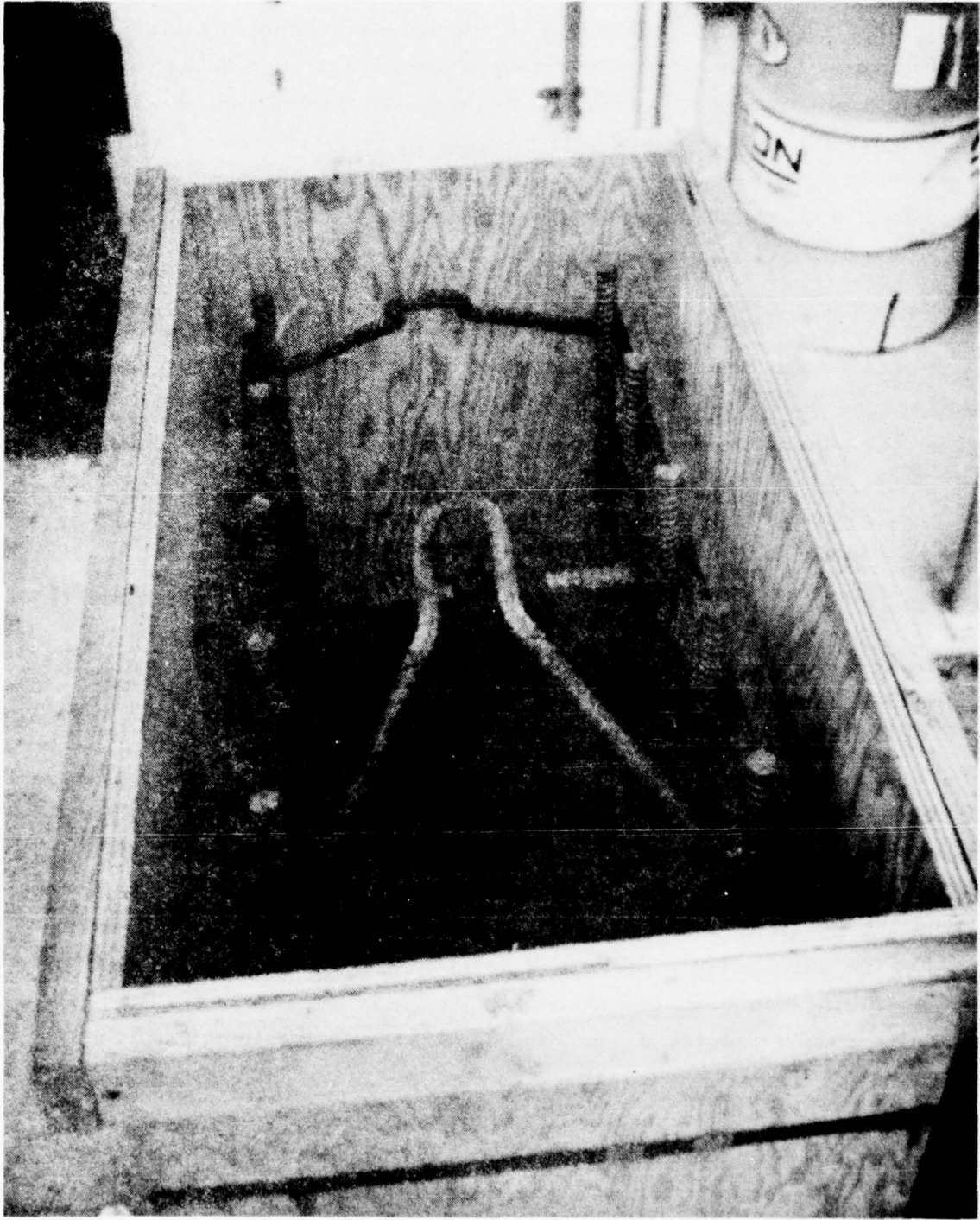
Figure 12. Concrete Target Form and Reinforcing Structure
