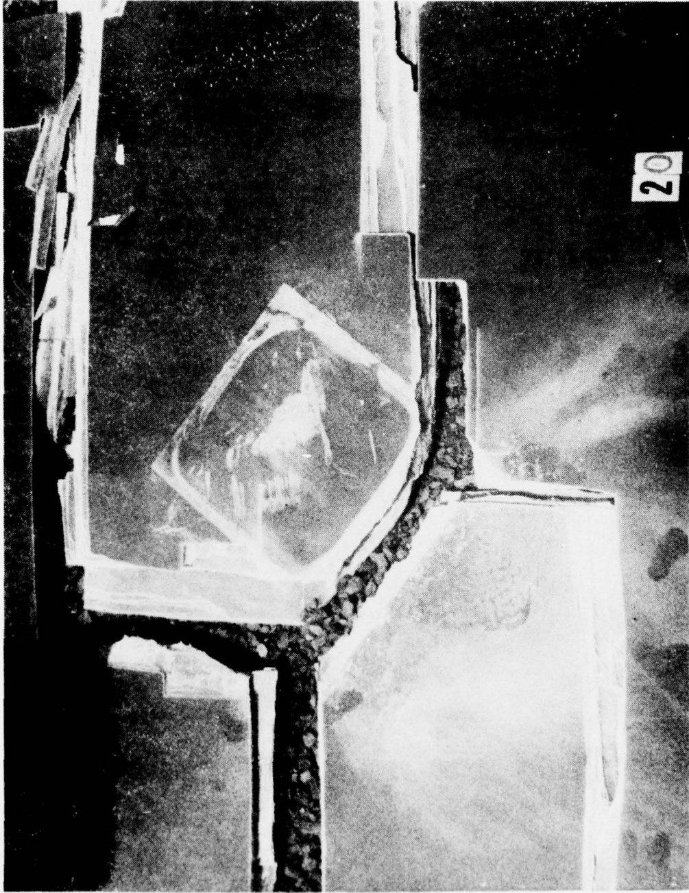
Figure 39. Test No. 20, 0.94-in. Thick Fiber Glass — Closeup
