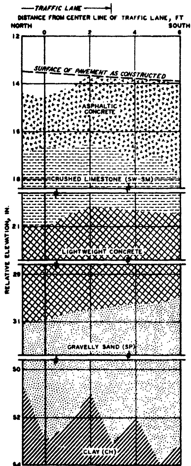
Figure 14. Test pit profile of sublayer 5c, flexible pavement test section. Station 1485 after 240 covers of 10-ton single-wheel assembly
