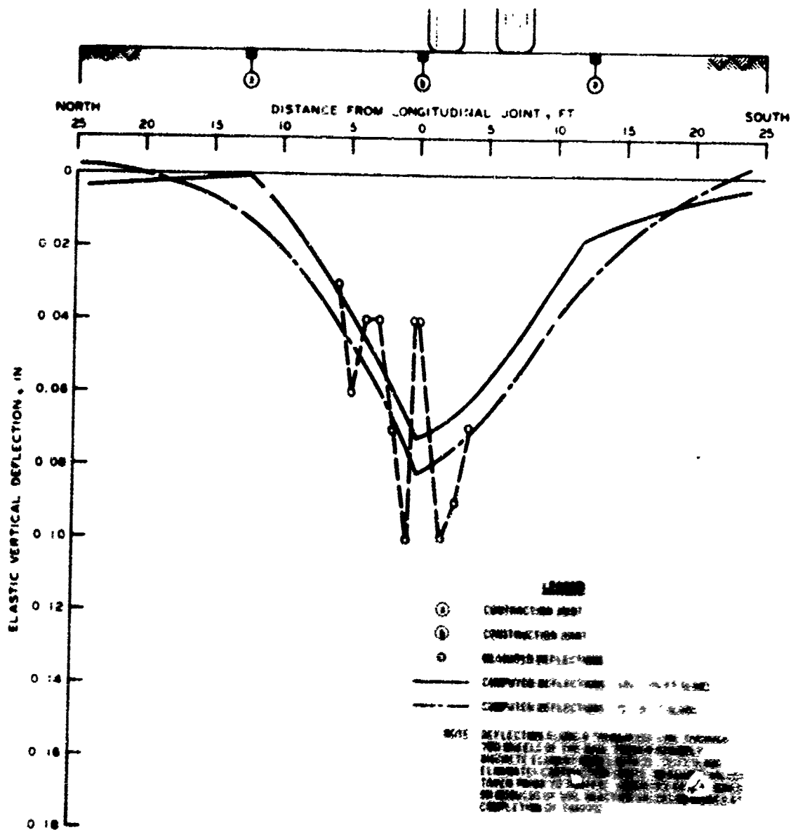
Figure 87. Deflections for rigid pavement sublayer, . . . . . showing a transverse line through two wheels
