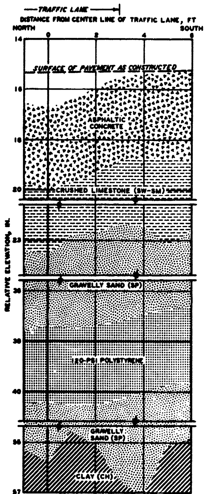
Figure 12. Test pit profile of subitem 4c, flexible pavement test section. Station 1+45 after 240 coverages of 50-k. single-wheel assembly
