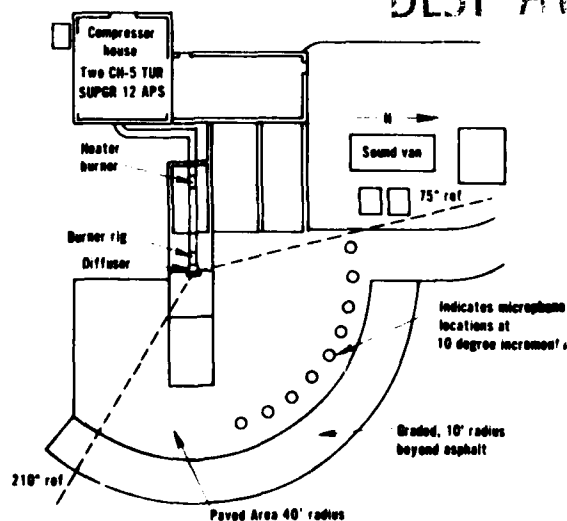
Figure 2.3-7 P&WA Outdoor Combustion Noise Facility, X-410 Stand
