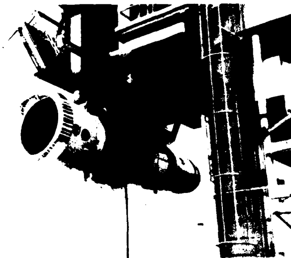
Figure 4.1-3 JT8D-109 Mounted At X-314 Stand
