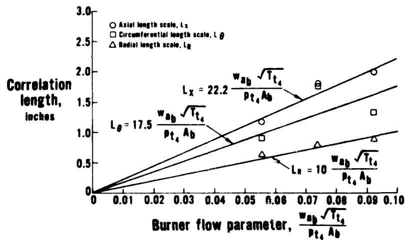
Figure 3.5-3 Correlation of Hot-Spot Length Scales At Exit of the JT8D-17 Burner
