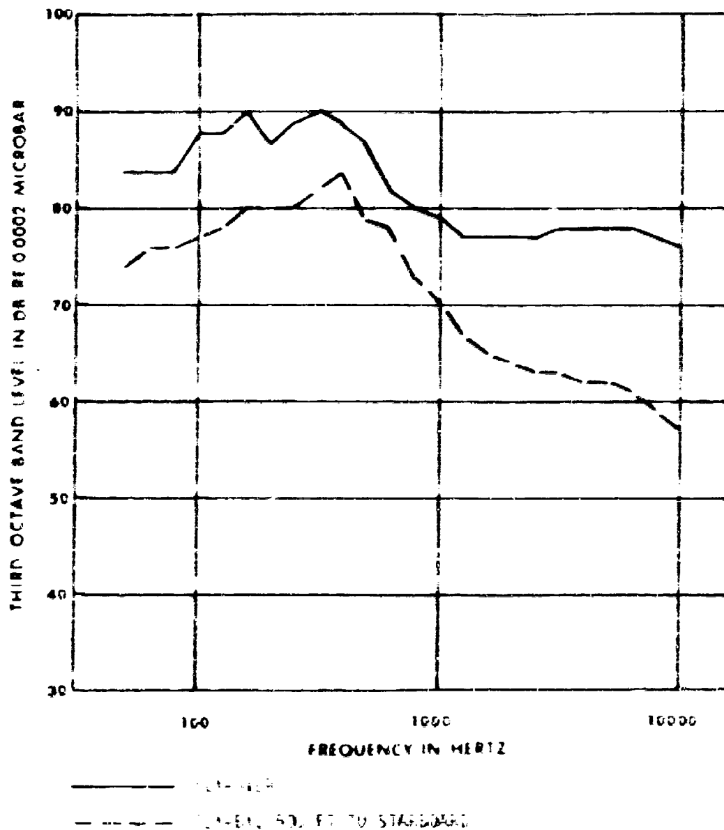
Figure 37. Calculated Baseline Noise Spectrum for Aircraft. Model S-67, 120 kts. Flight, 300 Ft. Altitude, at Time of Maximum PNL
