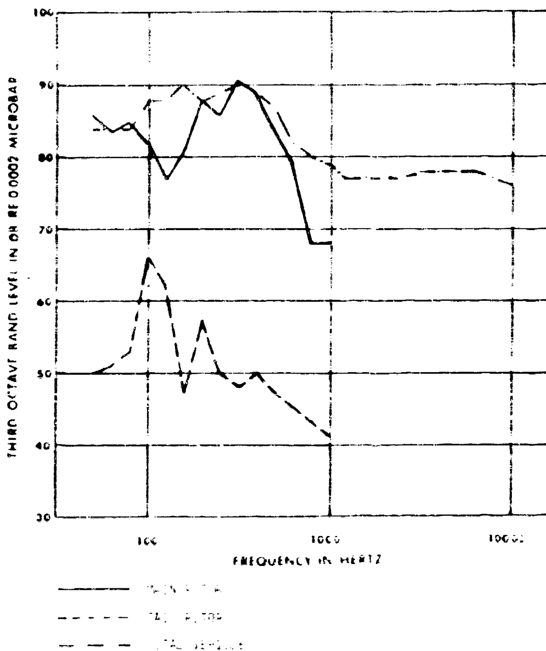
Figure 4. Calculated base line noise for quiet system noise field is compared to total vehicle noise spectrum. Frequency 300 Hz, 2000 Hz, 12000 Hz (1000 Hz) at time of maximum noise.
