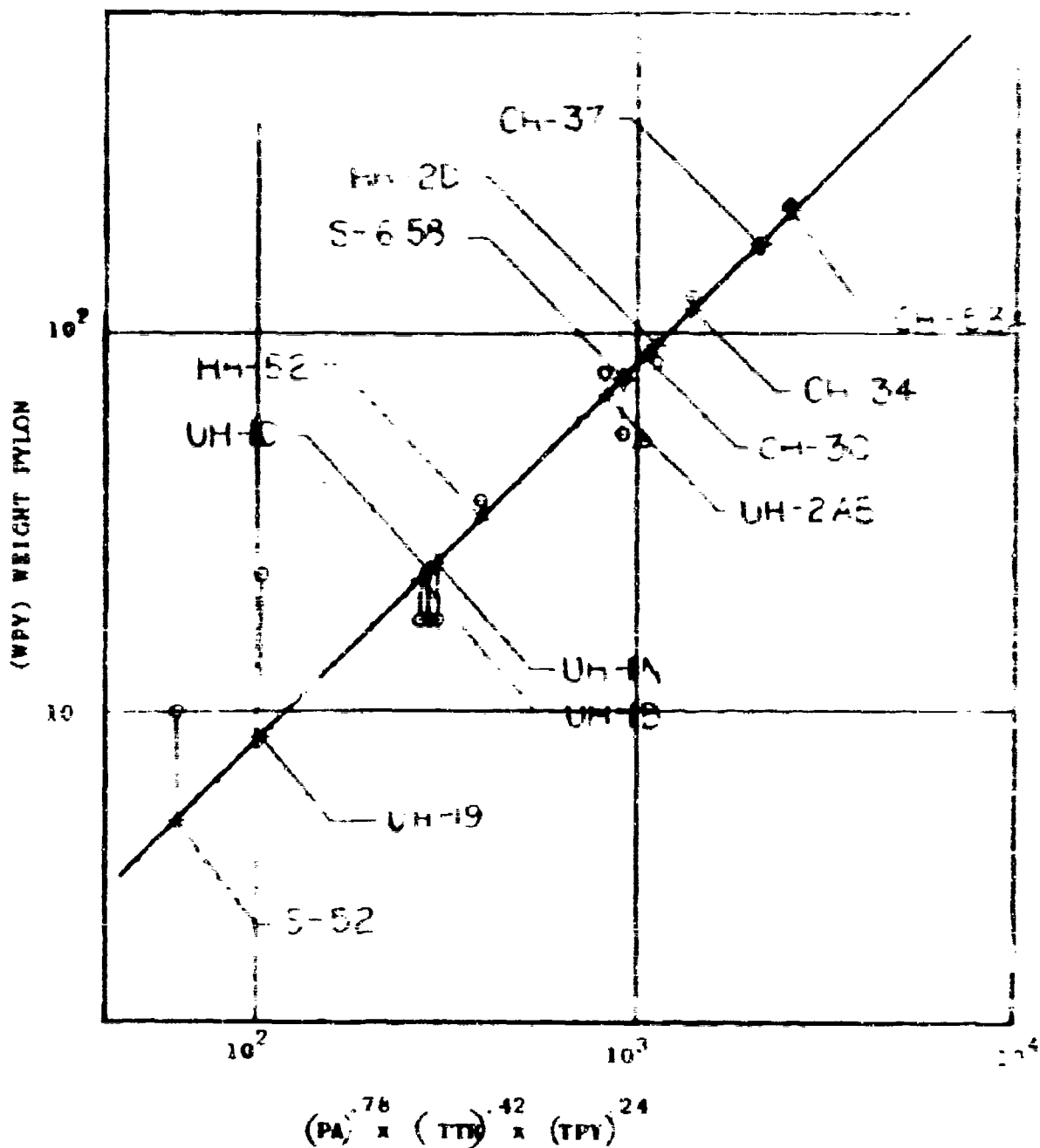
Figure 1-7. Pylon Weight
