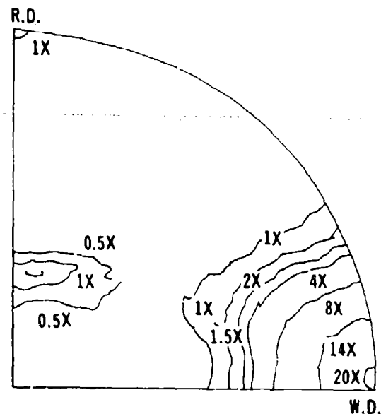
Figure 4: Material-6A1-4V Ti Standard Grade TMT Method 11
