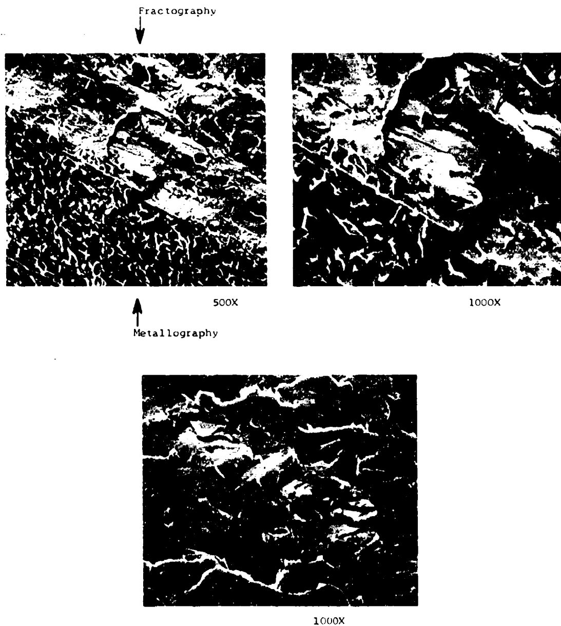
Figure 18 - Fractography/Metallography of Basal Transverse Textured 6Al-4V Ti ELI Grade; Condition - Rex'1 at 1700°F + Furnace Cool; da/dn Test in 3.5% NaCl in H 2 O at 20 cps; Orientation - TL; 10 Ksi \sqrt{In} < \Delta K < 12 Ksi \sqrt{in} ; da/dn ~ 3 \times 10^{-5} inches/cycle.
