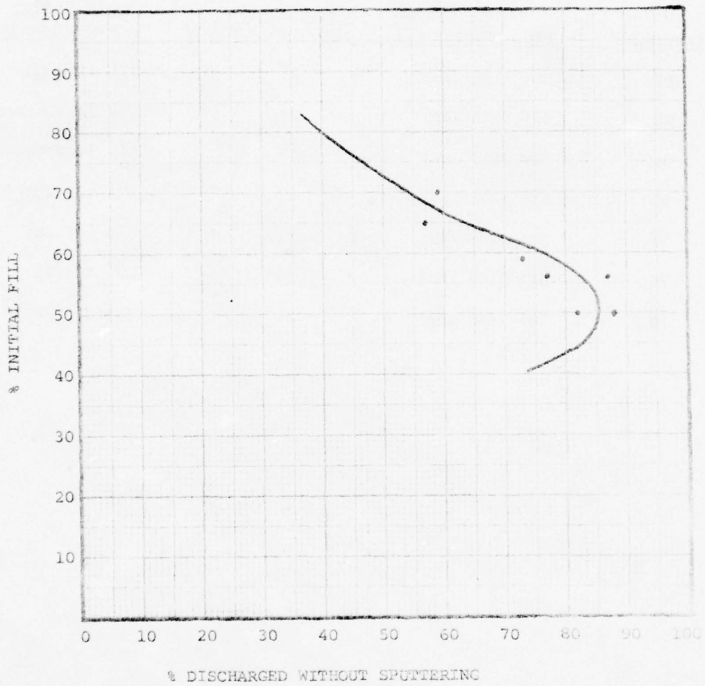
FIG. 11 PER CENT DISCHARGED WITHOUT SPUTTERING VERSUS FILL RATIO
