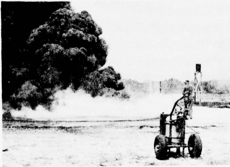
FIG. 33 NOVICE POOL FIRE #6 (AREA 840 FT 2 )
