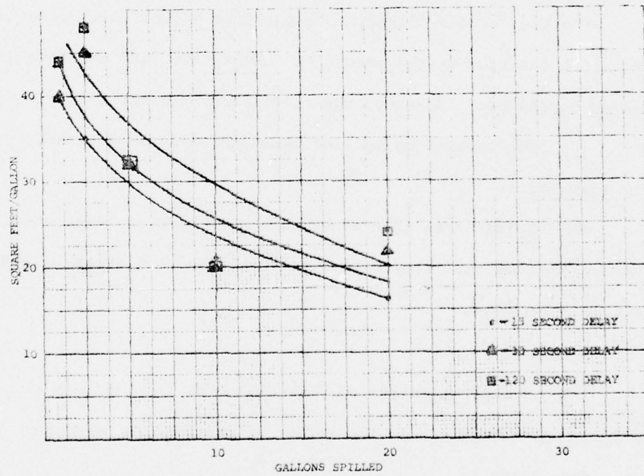
FIG. 17 AREA/GALLONS AFTER IGNITION
