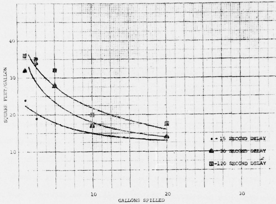
FIG. 16 AREA/GALLONS BEFORE IGNITION
