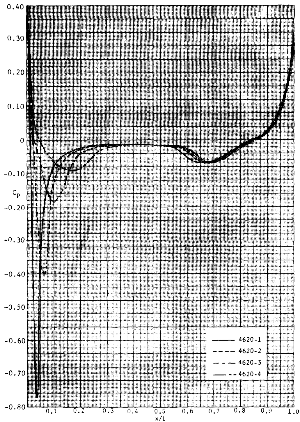
Figure 11A - Series 4620-1, 2, 3, 4 Pressure Distributions
