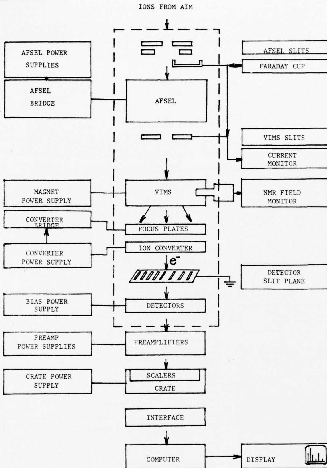
Figure 8b. Electrical Block Diagram of the AMS
