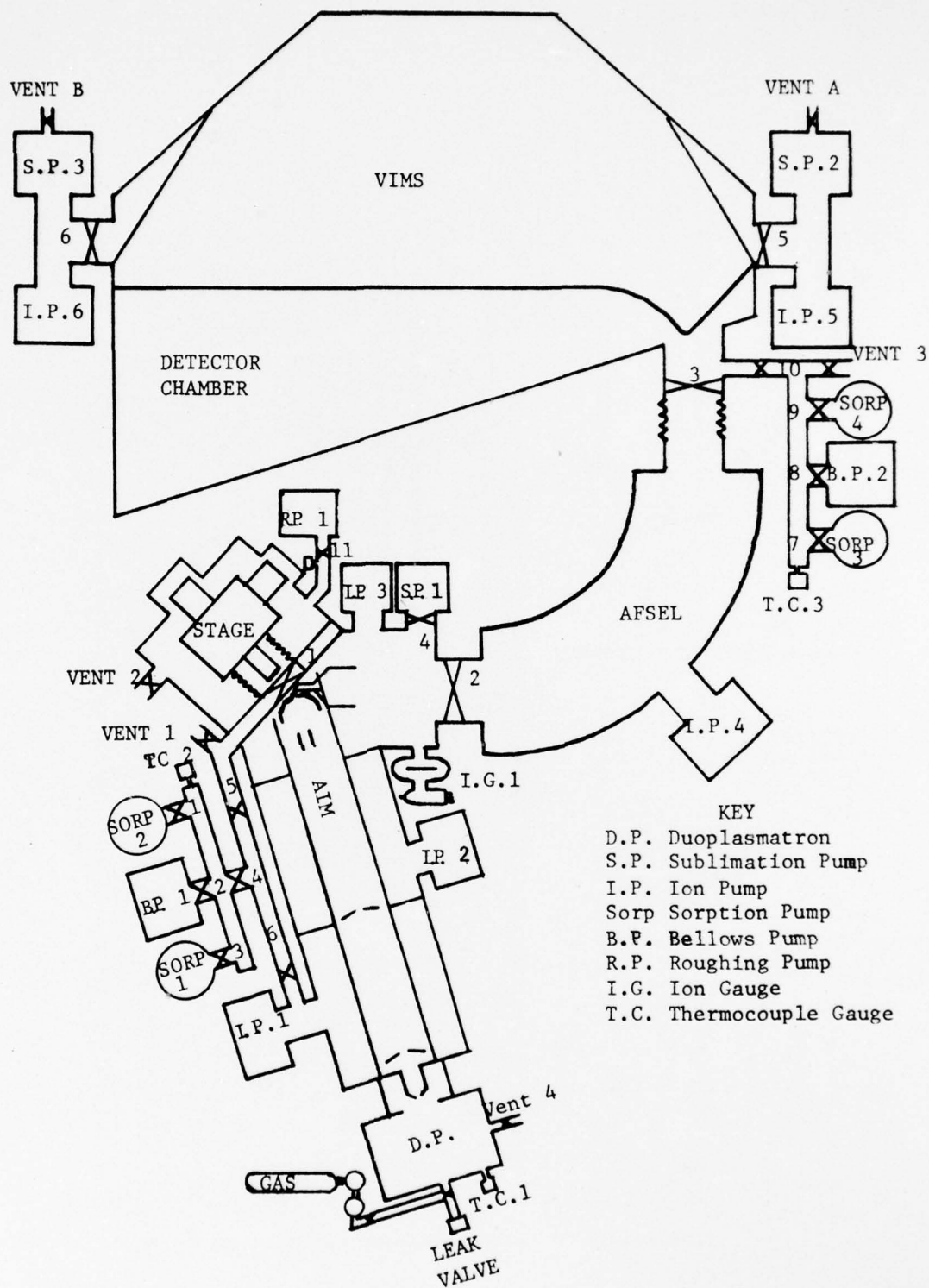
Figure 2. Vacuum System Diagram
