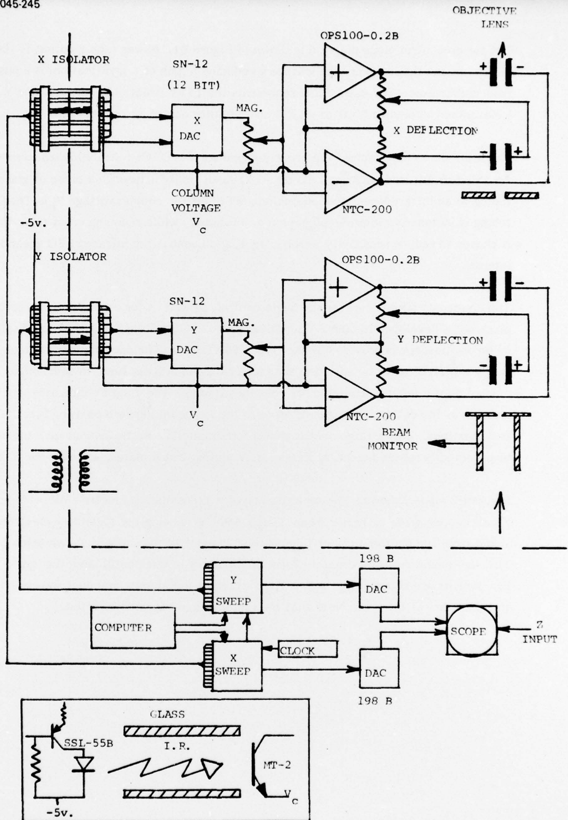
Figure E1 Primary Ion Beam Control
