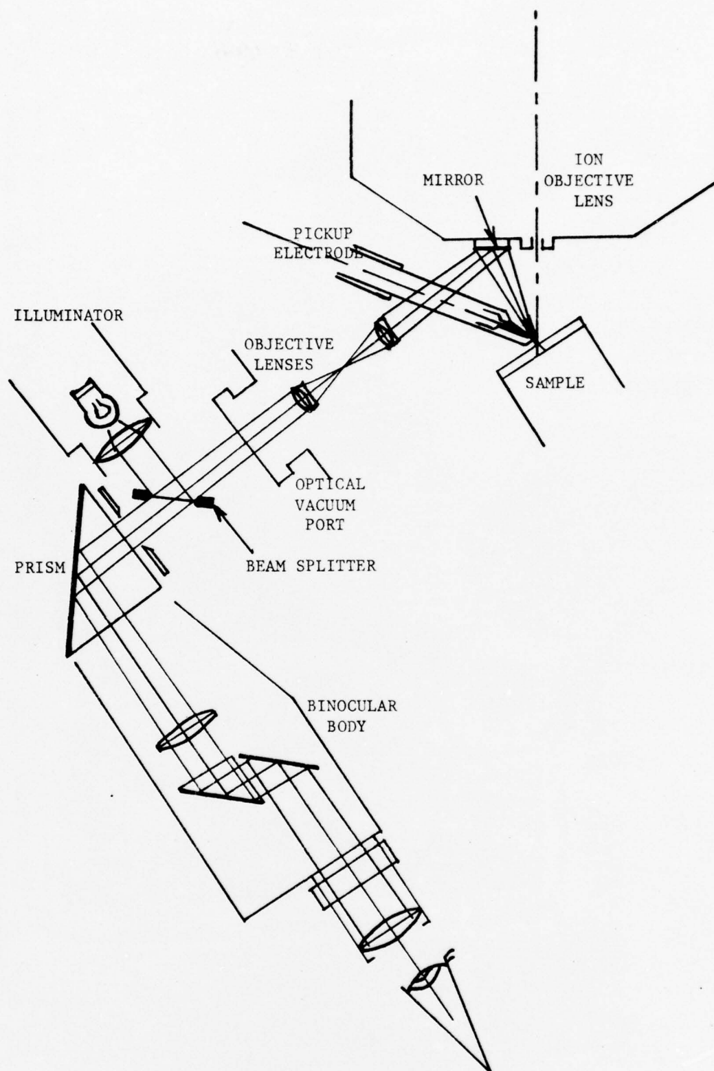
FIGURE 10 Schematic of the Low Power Optical Microscope
