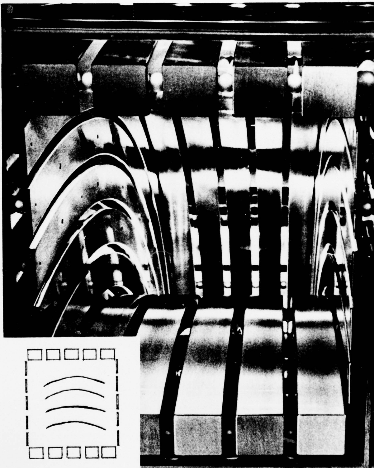
Figure 12. AFSEL - Interior View and Cross Section of Equipotentials
