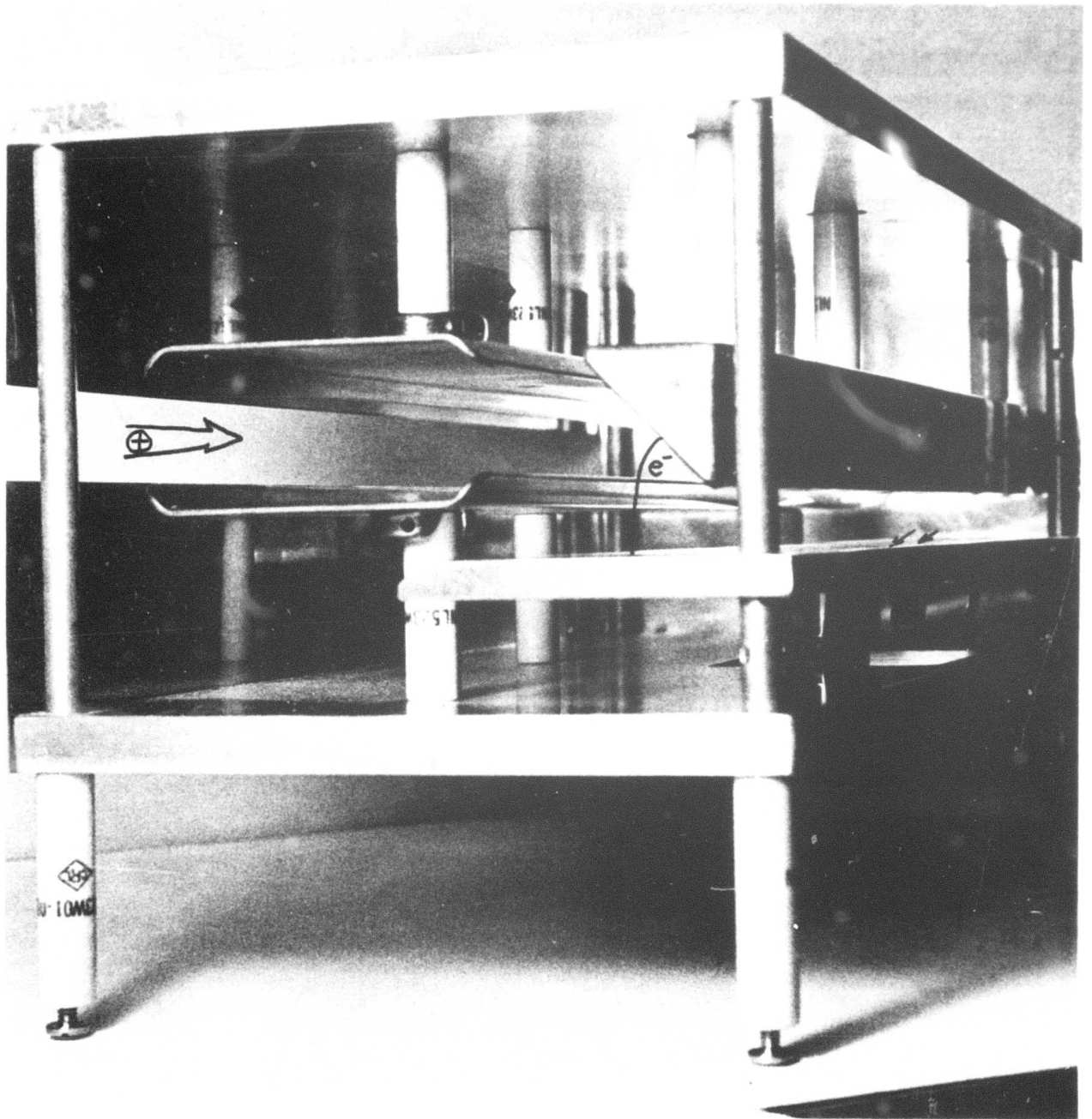
Figure 16. Prototype Converter with Two Detectors in Place
