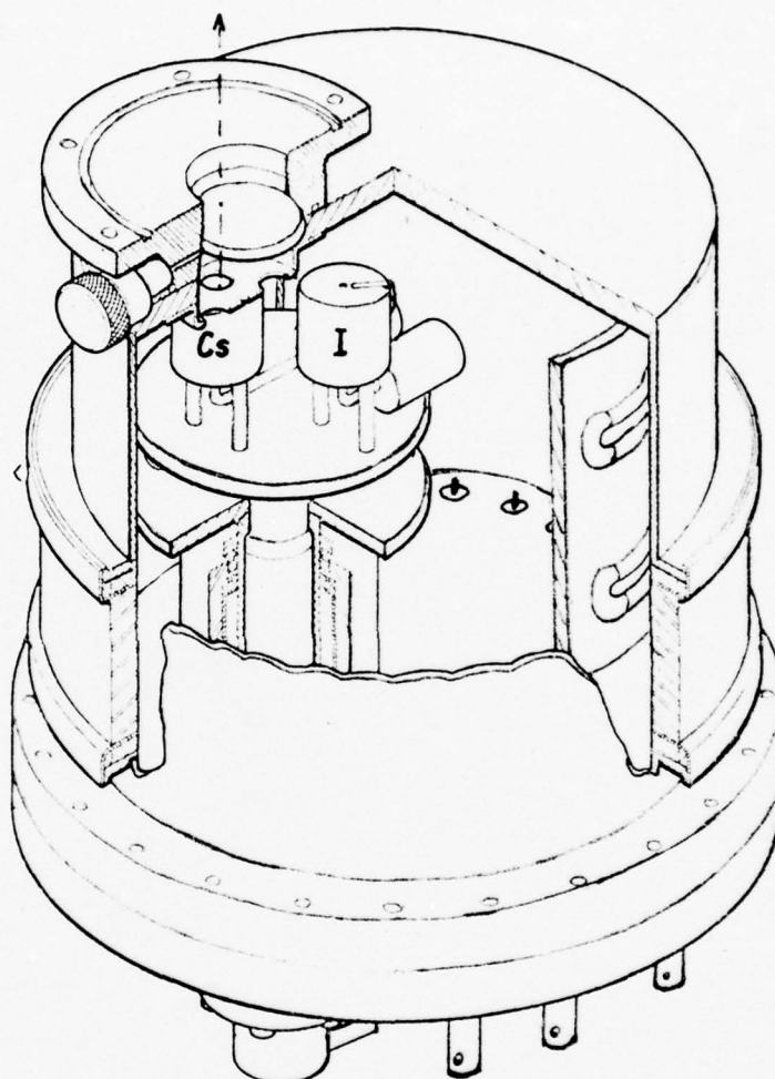
Fig. 5. Isometric view of source chamber showing detail of source positioning mechanism.
