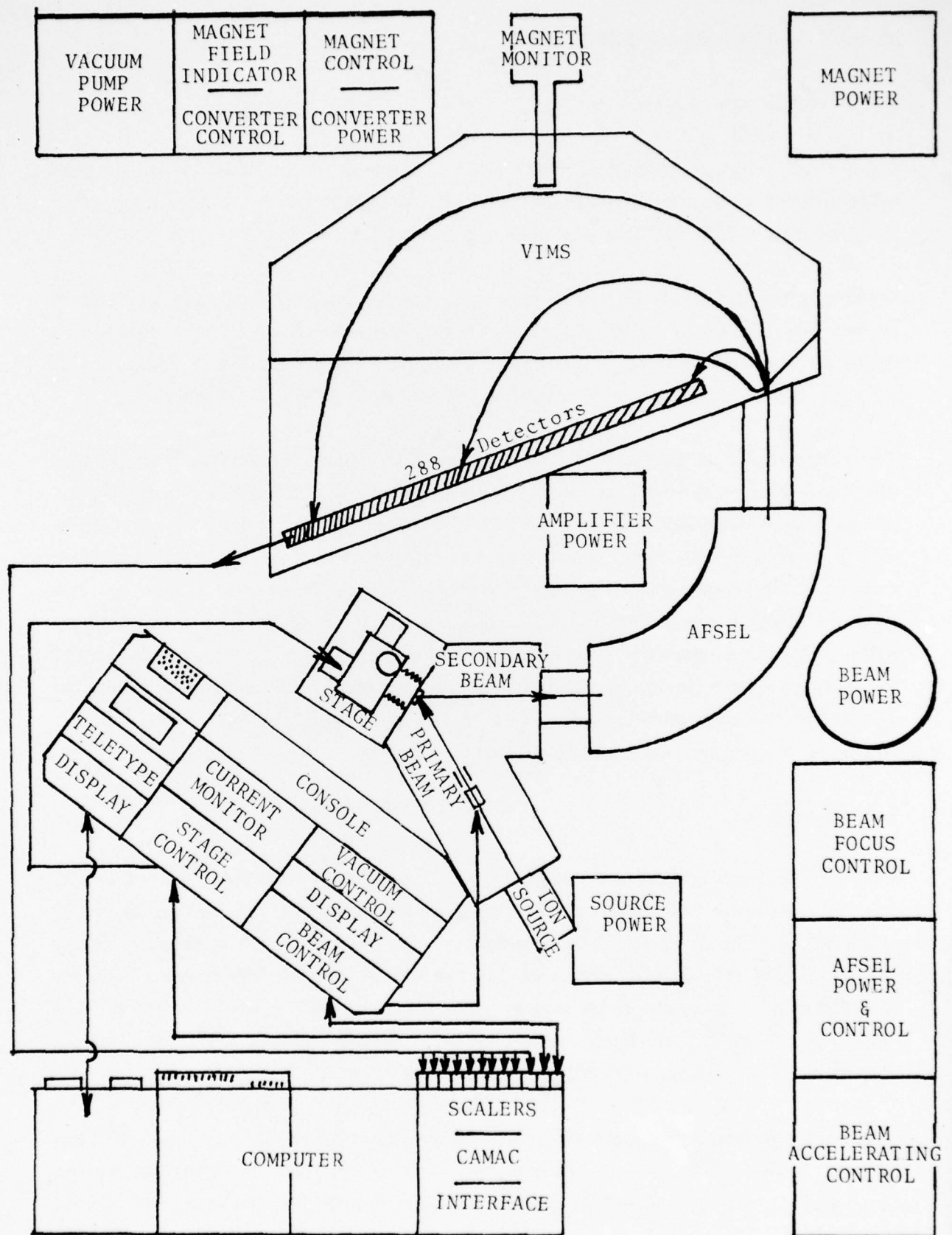
Figure 1. AMS System Diagram
