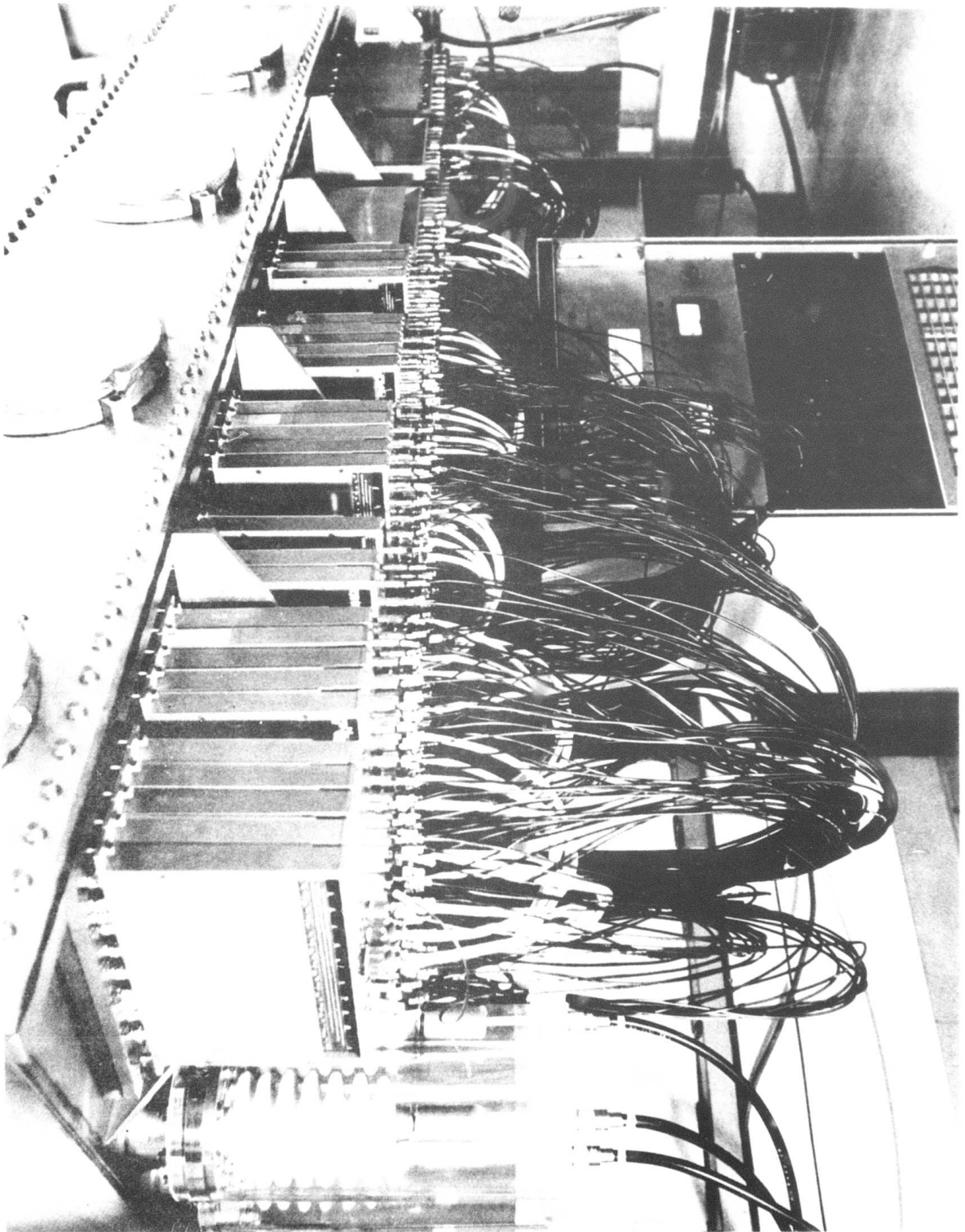
Figure 21. Preamplifier/Amplifiers in Position Under the Detector Vacuum Chamber
