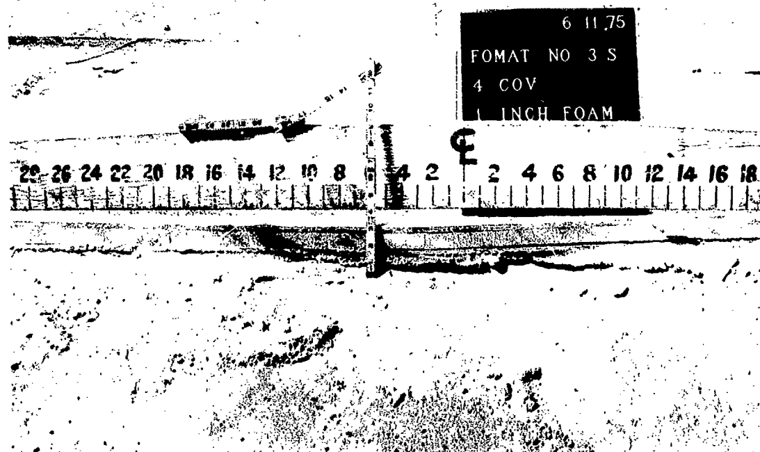
Figure 34. Cross section of FOMAT panel S-1-20 after four passes of the wheel.
