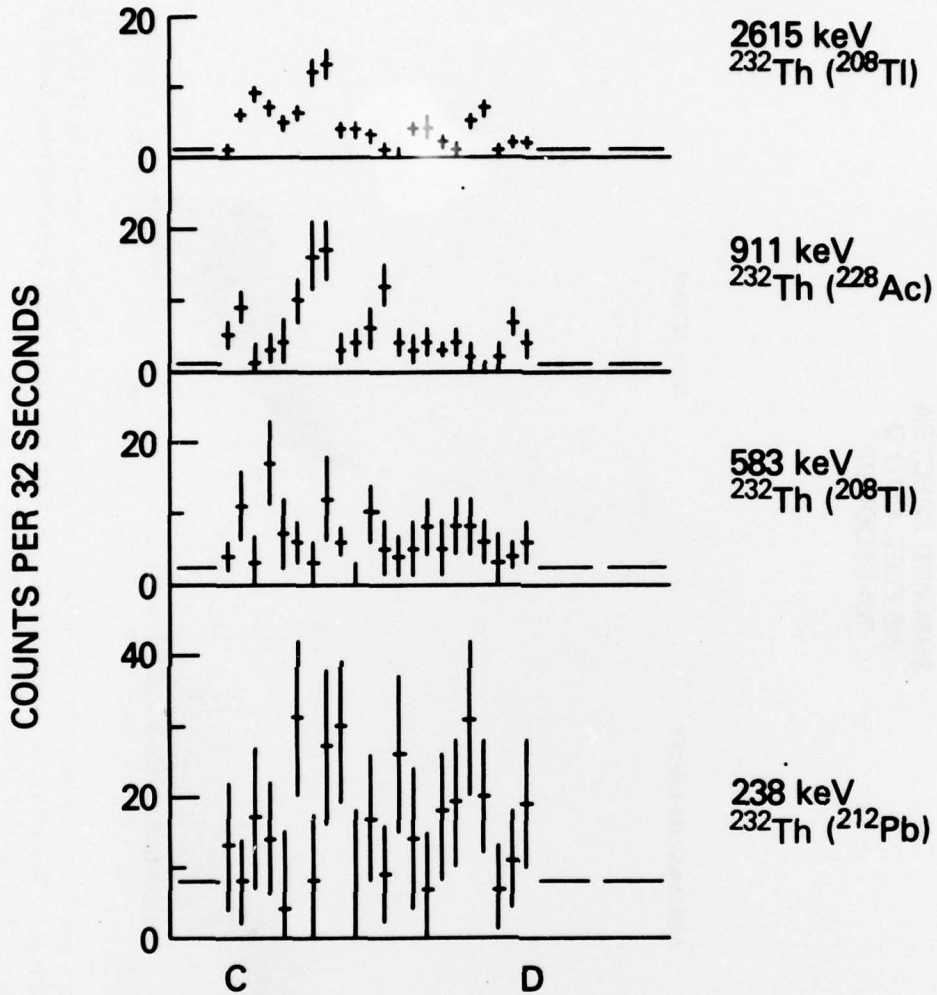
Fig. 4 - Germanium array data at 200 ft altitude from the analysis of the 32-second spectra from the decay of ^{232}\text{Th} . The dashed lines show the background at 17,000 ft.
