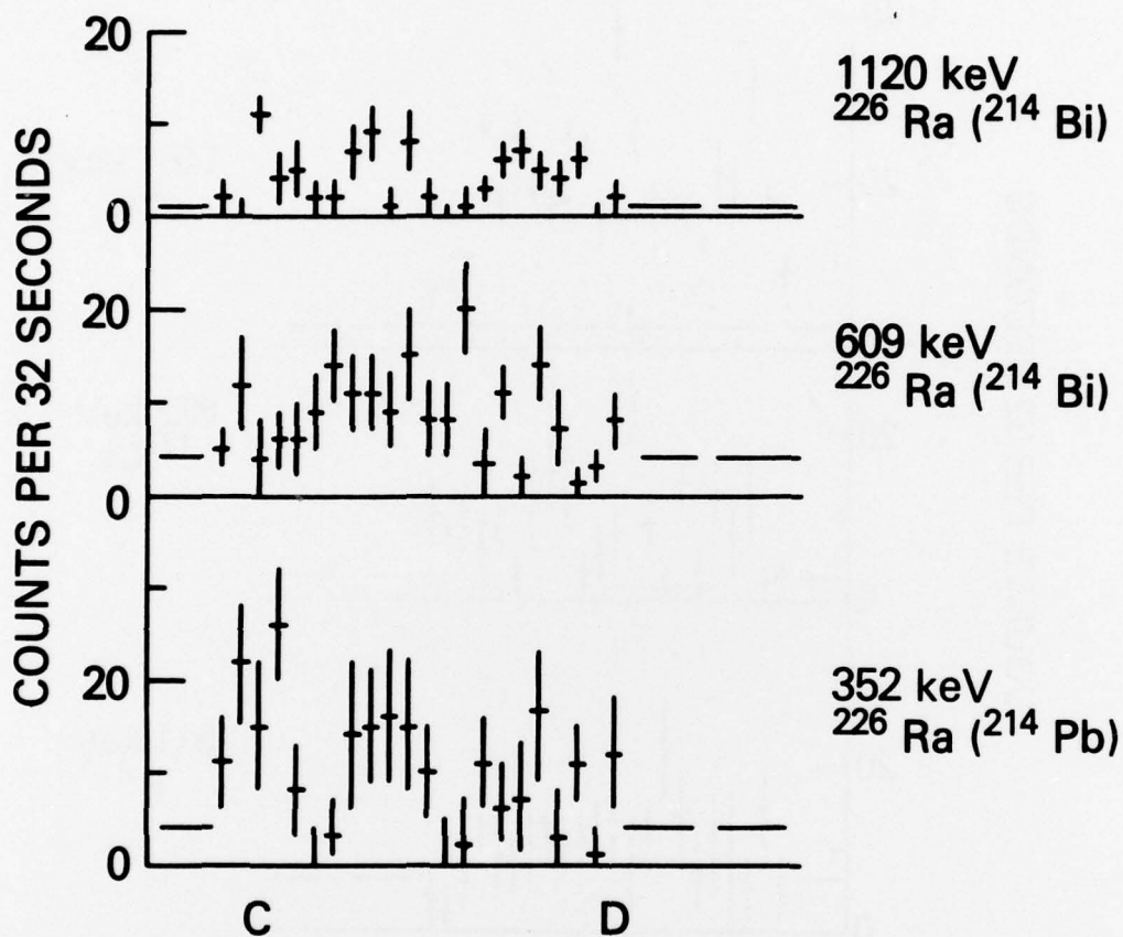
Fig. 6 - Germanium array data at 200 ft altitude from the decay of ^{226}\text{Ra} . Backgrounds at 17,000 ft are indicated by the dashed lines.
