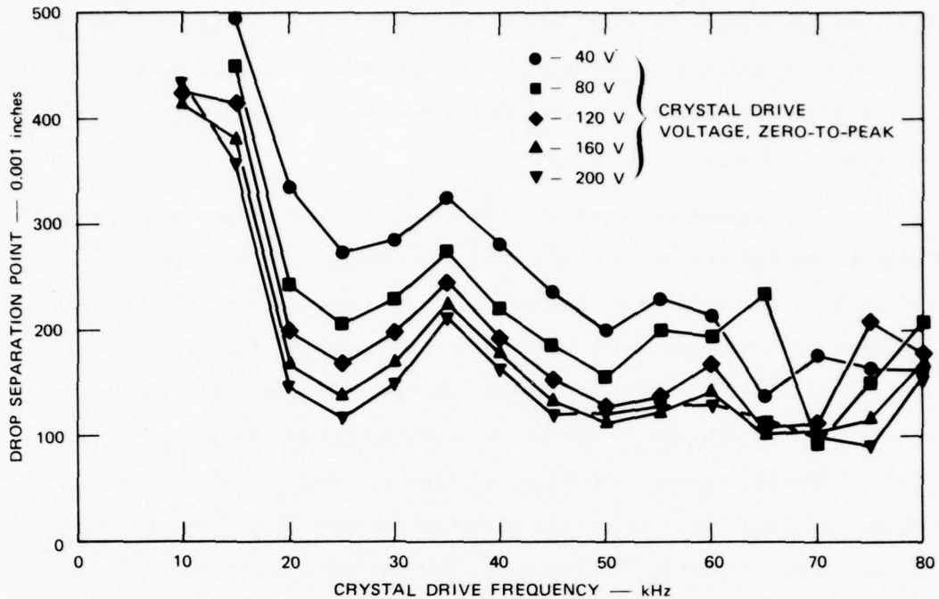
FIGURE 11 DROP SEPARATION POINT VERSUS CRYSTAL DRIVE FREQUENCY Data taken with A.B. Dick ink 16-1000; Supply Pressure = 30 psig
