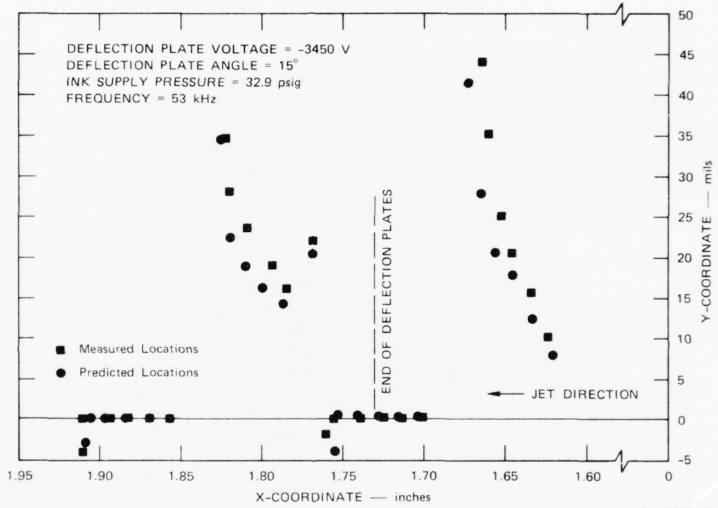
FIGURE 25 IN-FLIGHT DROP COORDINATES, TEST CASE 2
