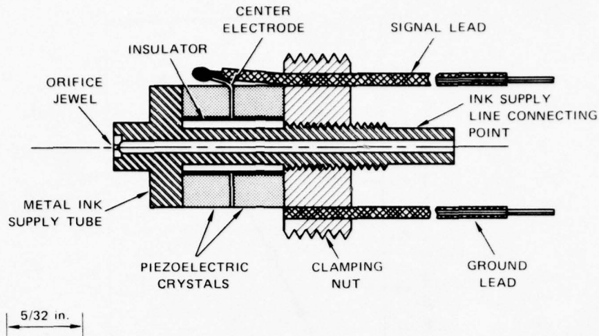
FIGURE 6 CROSS SECTION OF JET PERTURBING APPARATUS
