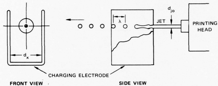
FIGURE 16 CHARGING STATION
