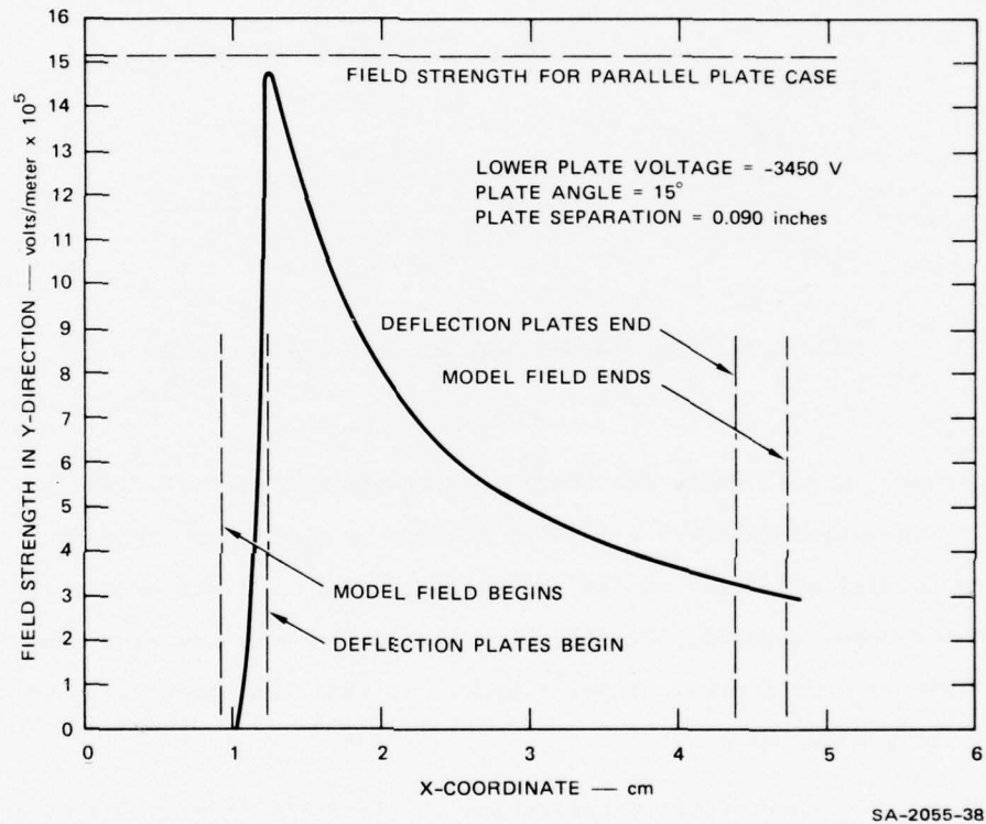
FIGURE 22 DEFLECTING FIELD STRENGTH VERSUS X-COORDINATE
