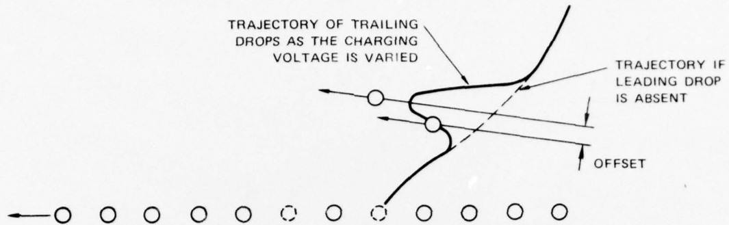
FIGURE E-8 WAKE WIDTH OF LEADING DROP EXPERIMENT
