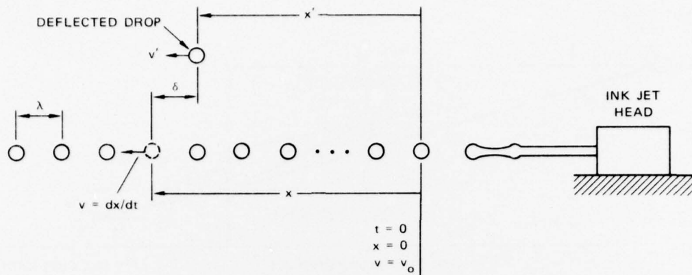
FIGURE E-2 INK JET SEEN UNDER STROBOSCOPIC LIGHT
