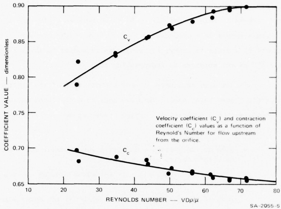
FIGURE 3 ORIFICE COEFFICIENTS VERSUS REYNOLDS NUMBER
