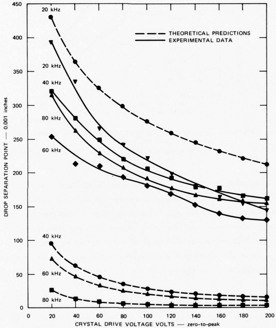
FIGURE 9 DROP SEPARATION POINT VERSUS CRYSTAL DRIVE VOLTAGE Data taken with A.B. Dick ink 16-1000; Supply Pressure = 30 psig
