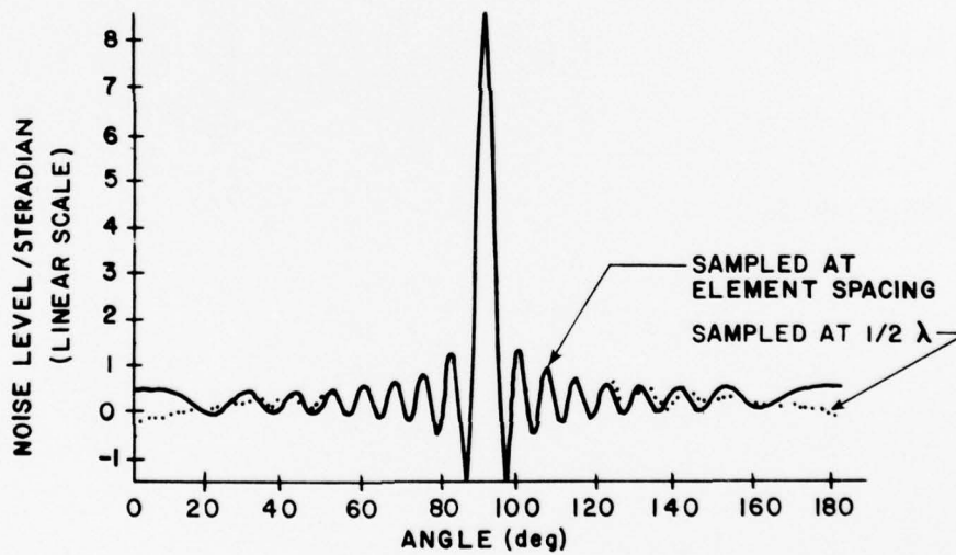
Figure 5b. Estimated Noise Directionality
