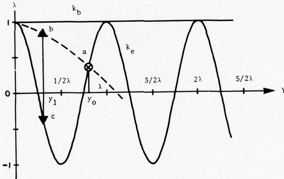
Figure 2. Cross Spectrum of Hydrophone Pair in Response to Directional Wave as a Function of Their Separation Distance
