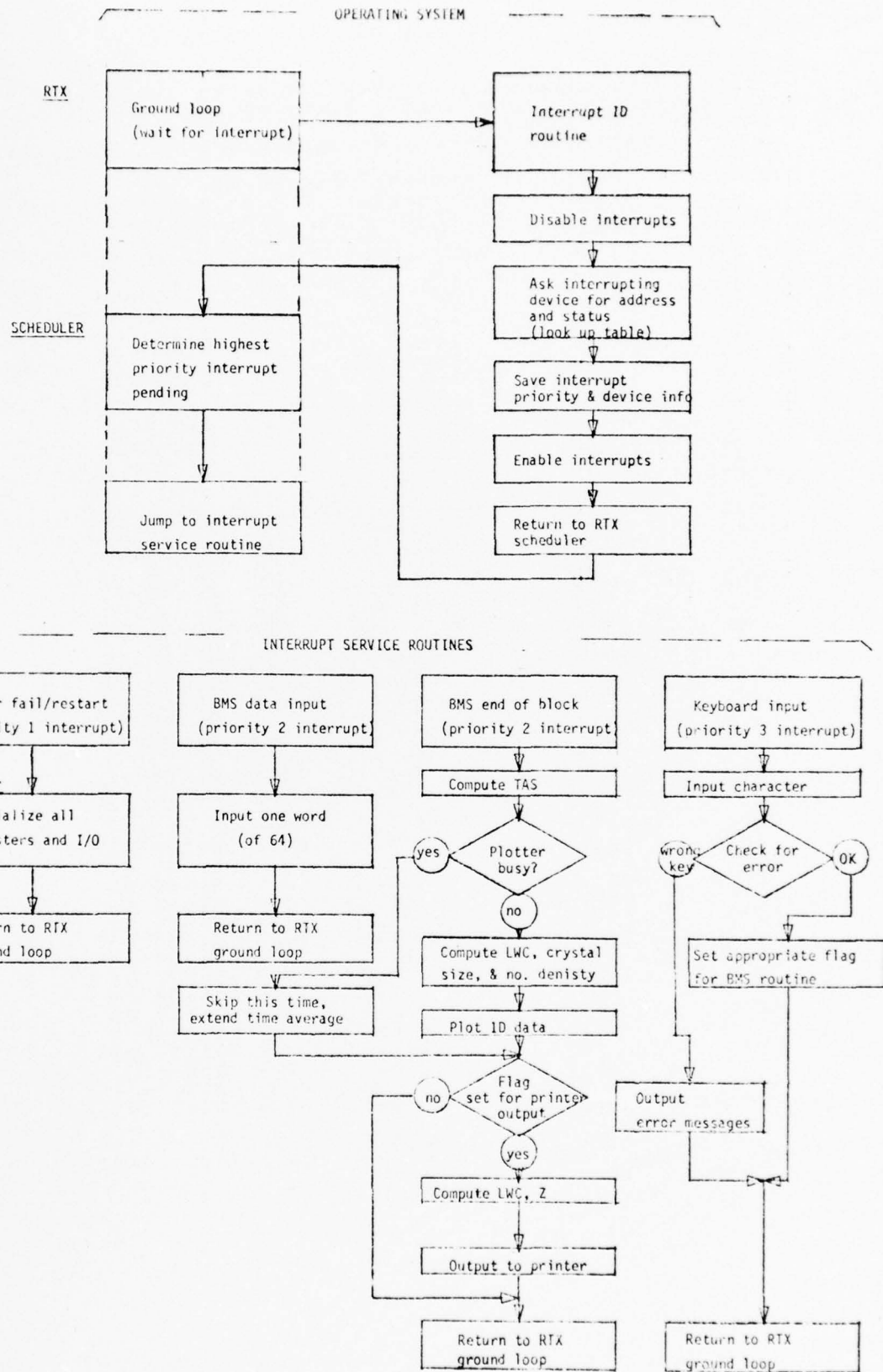
Figure 2.19 Flow diagram, real time program.
