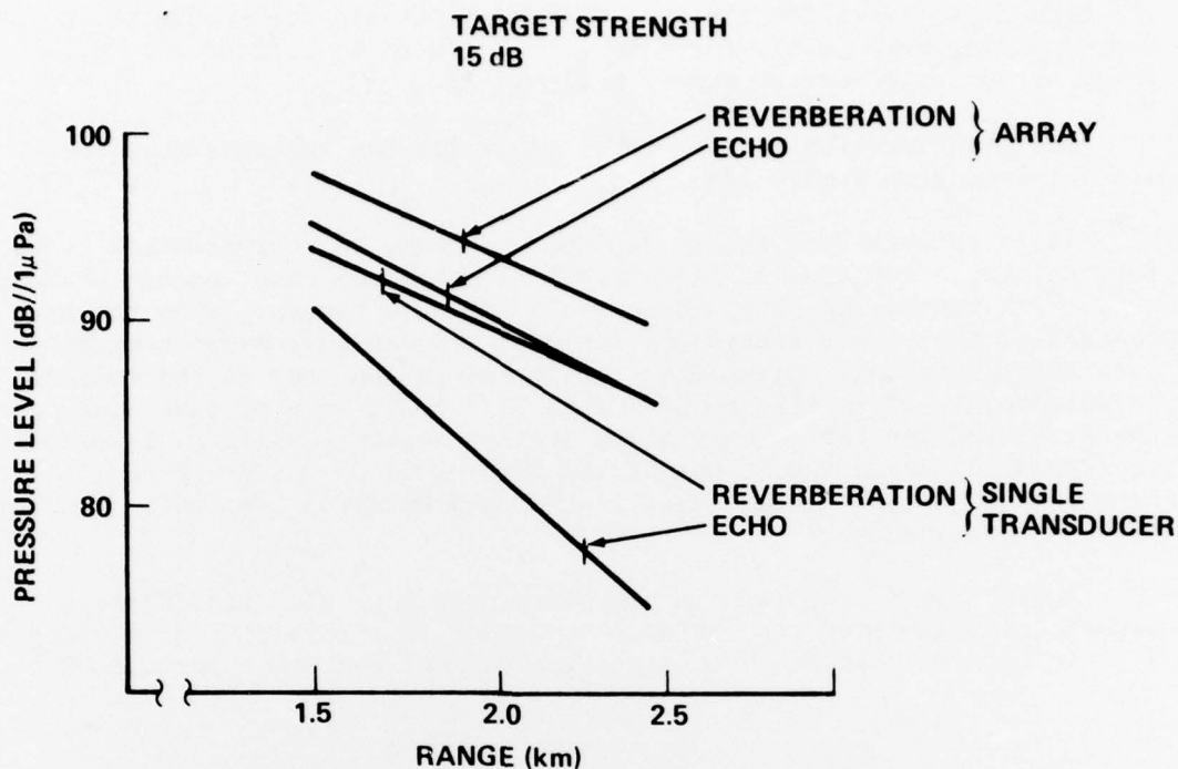
Figure 13. Echo to Reverberation Level Vertical Array Versus Single Transducer Target Strength 15 dB
