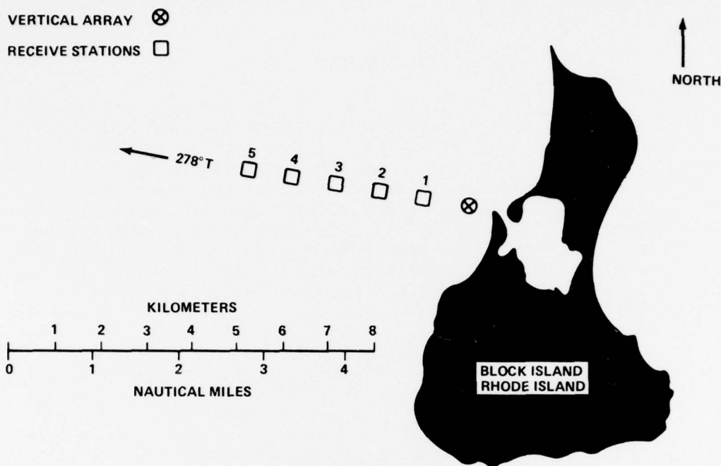
Figure 1. Experiment Diagram
