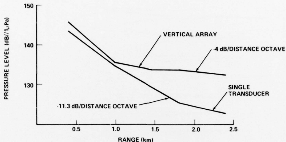
Figure 7. Depth-Average Signal Level Versus Range
